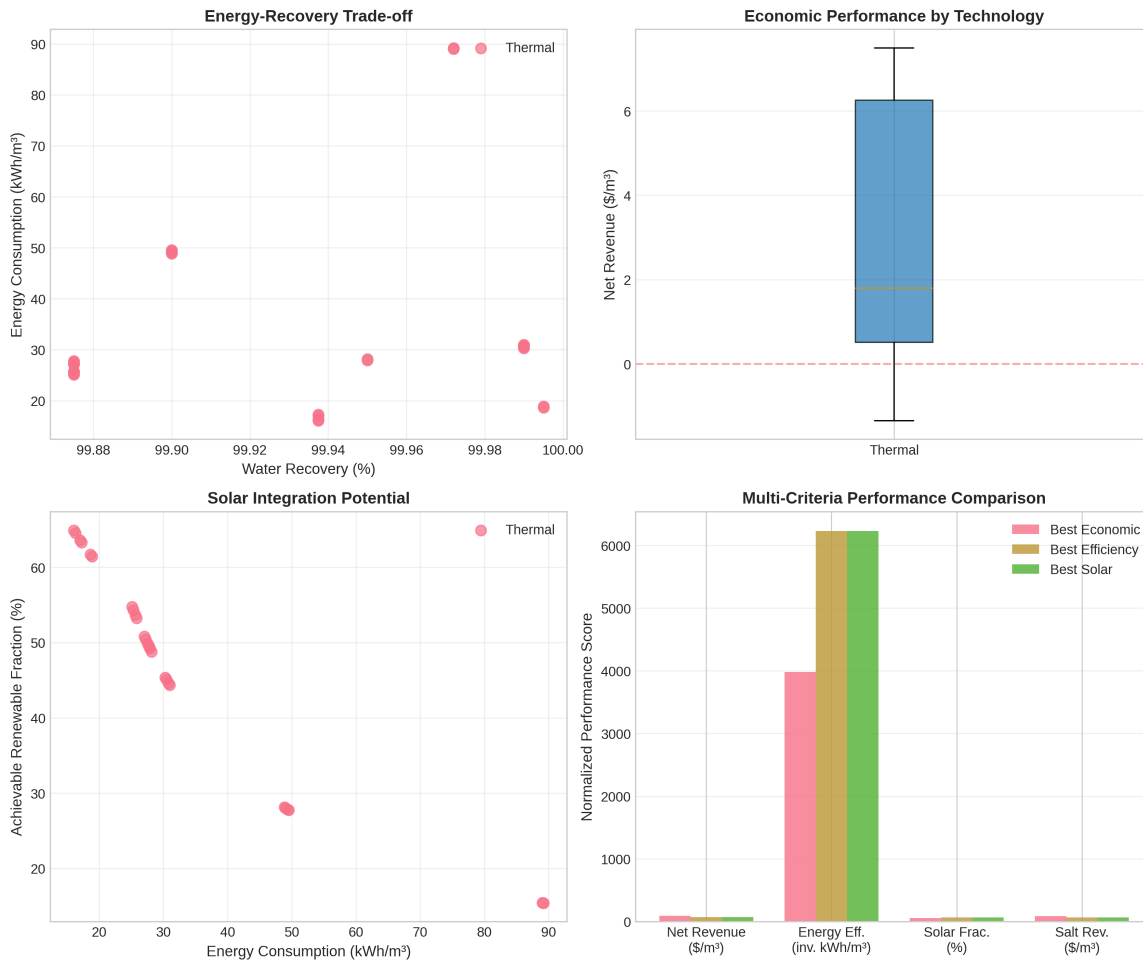
Figure 5. Multi-criteria performance matrix showing (a) energy-recovery trade-offs, (b) economic performance distribution, (c) solar integration potential, and (d) normalized comparison of top configurations.
