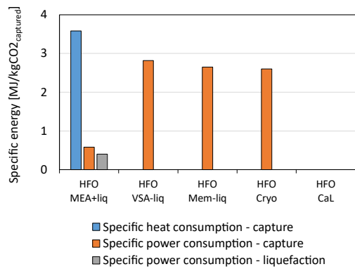
Figure 2. Specific energy consumption of OCCS systems in the retrofit (HFO) scenario.
