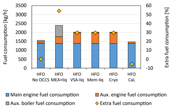
Figure 4. Total and extra fuel consumption of OCCS systems in the retrofit (HFO) scenario.
