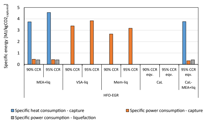
Figure 8. Specific energy consumption of OCCS systems in the newbuilding (HFO-EGR) scenario.
