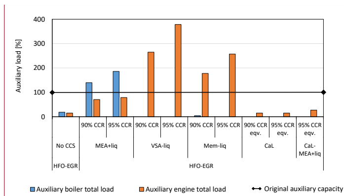
Figure 11. Auxiliary boiler and engine load of OCCS systems in the newbuilding (HFO-EGR) scenario.
