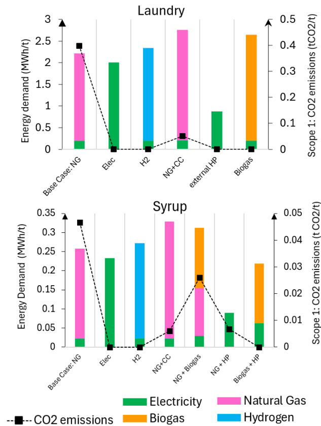
Figure 2. Specific energy consumption and CO 2 emissions in the laundry and syrup sectors based on energy choices
