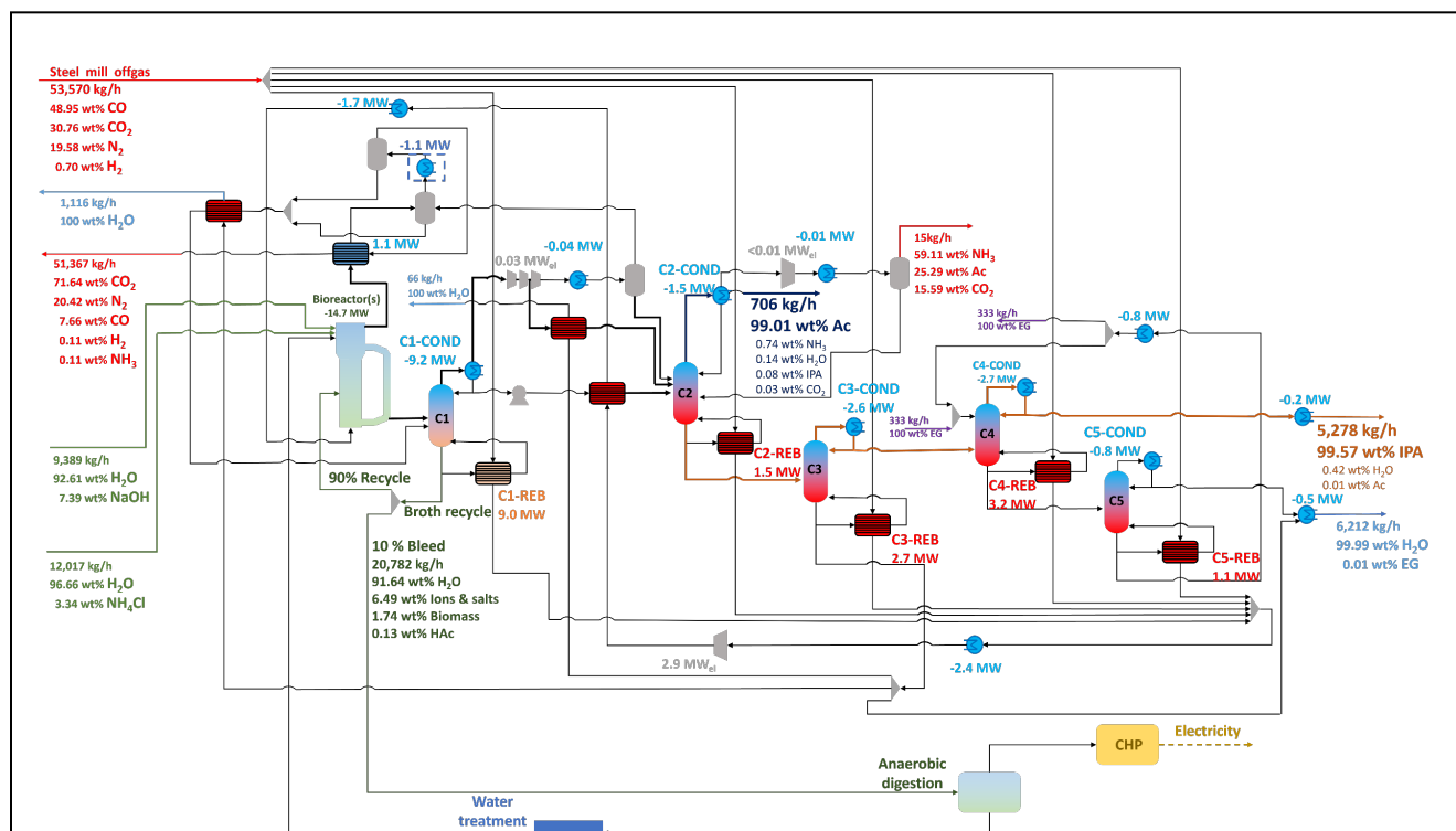
Figure 1: Overview of the 47.5 kton/year syngas fermentation (41.8 kton IPA /y, 5.64 kton acetone /y). The green inflows to the bioreactor are the pH control and nitrogen source, whereas the red in- and outflows are the gas streams. The inflowing syngas (at 1373 K/ 1100 °C) is used for heat exchange before it is compressed (3.84 bar) and fed to the bioreactor. Multi-stage heatpump integrated distillation is used to obtain 99.01 wt. % Ac (C2, dark blue) and 99.57 wt. % IPA (C4, orange). First the broth is separated from the volatile products (C1) by vacuum distillation. Followed by acetone distillation (C2), pre-concentration of IPA (C3), extractive distillation of IPA with ethylene glycol (EG) (C4), and EG recovery (C5). The anaerobic digestion, combined heat and power generation (CHP), and water treatment to demiwater are included within the system boundaries for the economic and environmental assessment.
