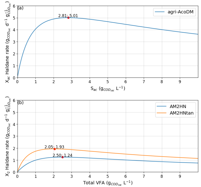
Fig. 2: Haldane's curve with the parameters \theta_{PSS}^* estimated offline: (a) for agri-AcoDM (corrected with temperature = 316.15 K) and (b) for AM2HN and AM2HNtan (values converted to acetate-equivalent, agri-AcoDM-like, units).
