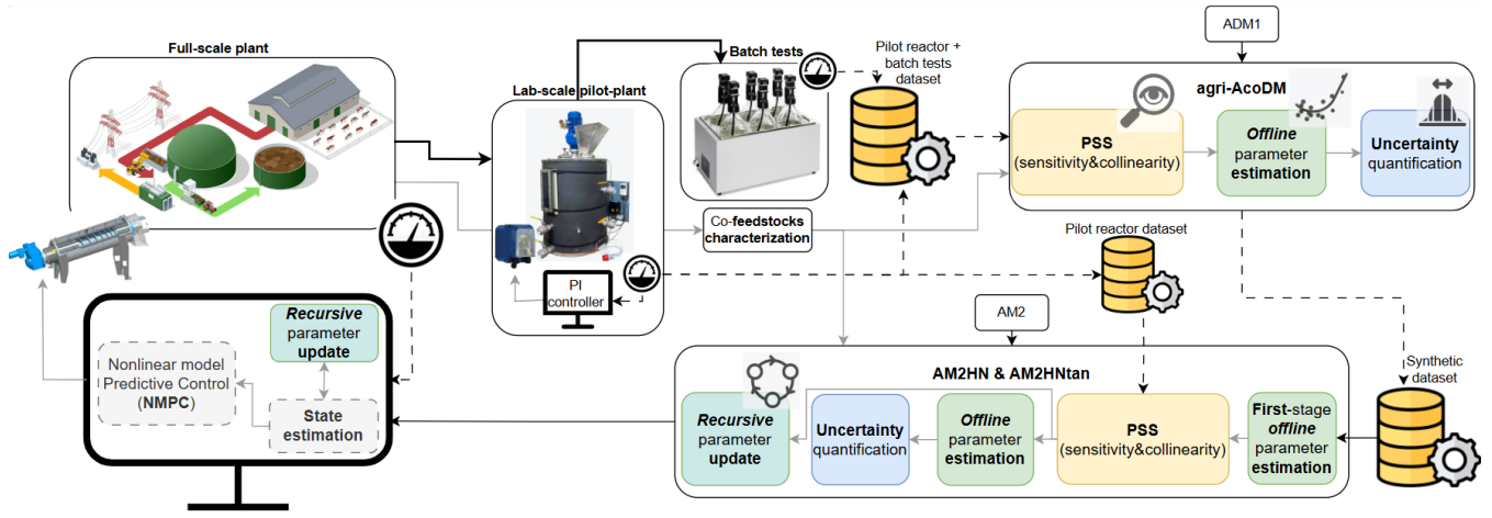
Fig. 1: Visual abstract of the modeling approach followed in this work. Black thick lines represent bacterial inoculum in digestate; black dotted lines represent data, whereas gray lines represent exchange of 'information' in a broader sense; regular black line refers to the reduced-order model that, after the tuning carried out as reported in this work, can be used for the design of state observers and model-based predictive controllers i.e. digital twins.
