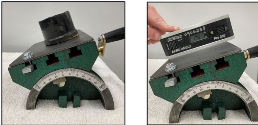
Figure 2. Apparatus used to measure friction coefficient. Note that the container was lifted, thus only kernels were in contact with the surface ( left ). The friction coefficient was estimated at the slope angle at which the kernel layer began to slide by overcoming the sliding friction resistance ( right ).
