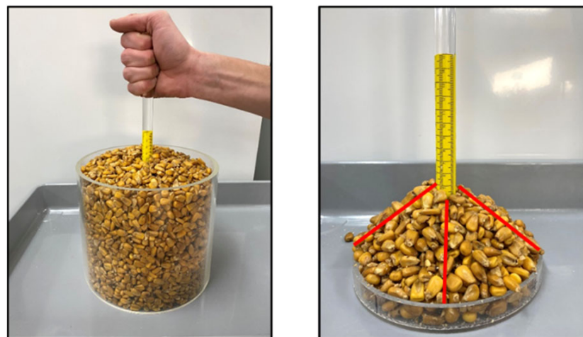
Figure 5. Anchor-lifted device filled with grain and the anchor being slowly lifted ( left ) to avoid particles agitation. Angle of repose was determined by measuring the pile height from the top of the anchor's annular ring to the top of the pile at four radial locations 90 degrees apart ( right ).
