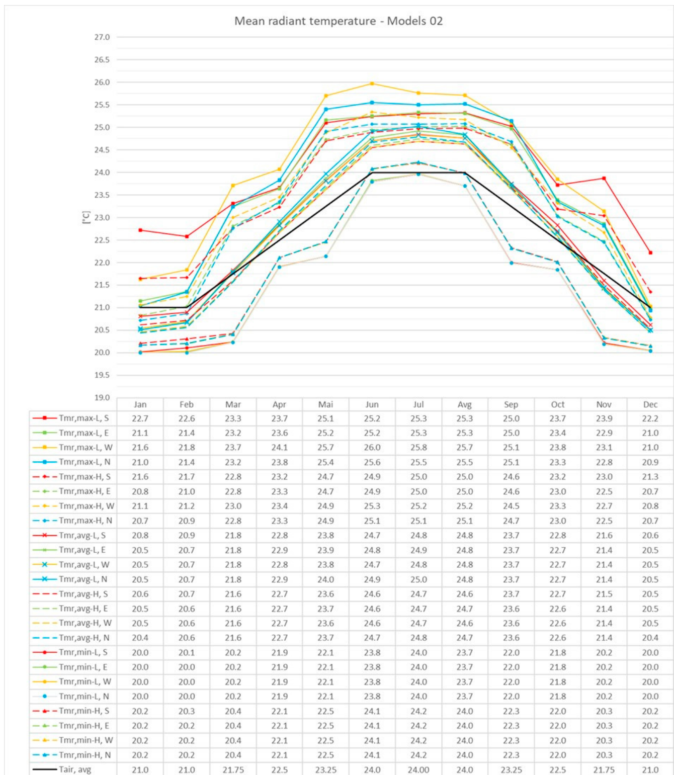
Figure A2. Monthly mean radiant temperature fluctuations for the observed orientations in Models 02.
