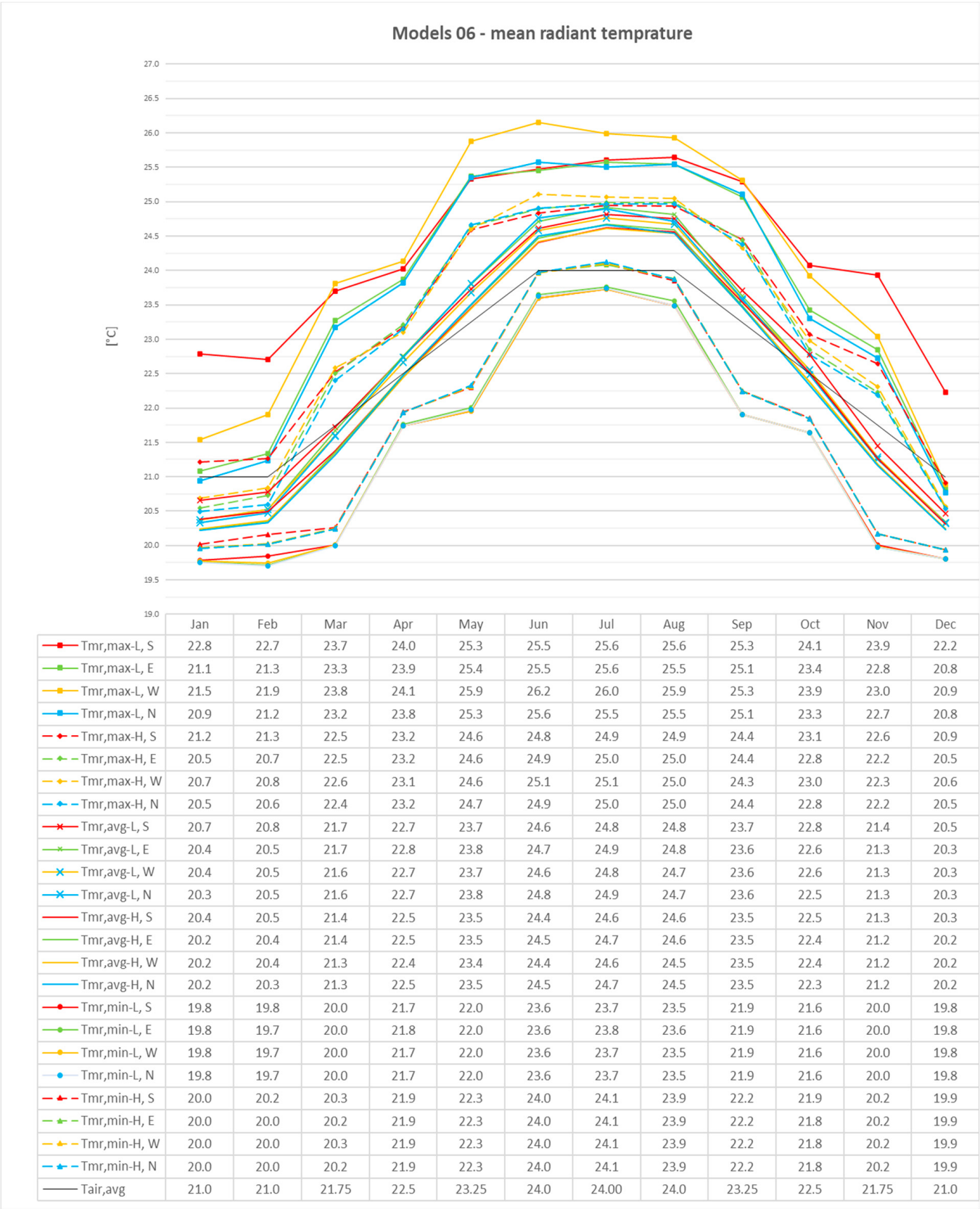
Figure A1. Monthly mean radiant temperature ( T_{mr} (°C)) fluctuations for the observed orientations in Model 06 thermal comfort simulation models.
