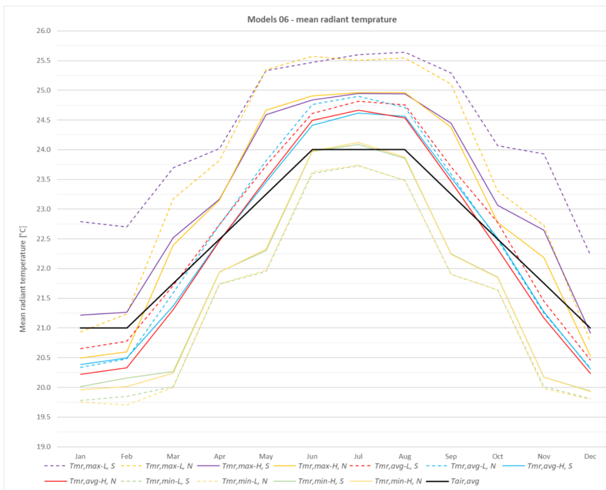
Figure 3. Monthly mean radiant temperature ( T_{mr} (°C)) values for the south and north oriented rooms in Model 06 thermal comfort simulation models.
