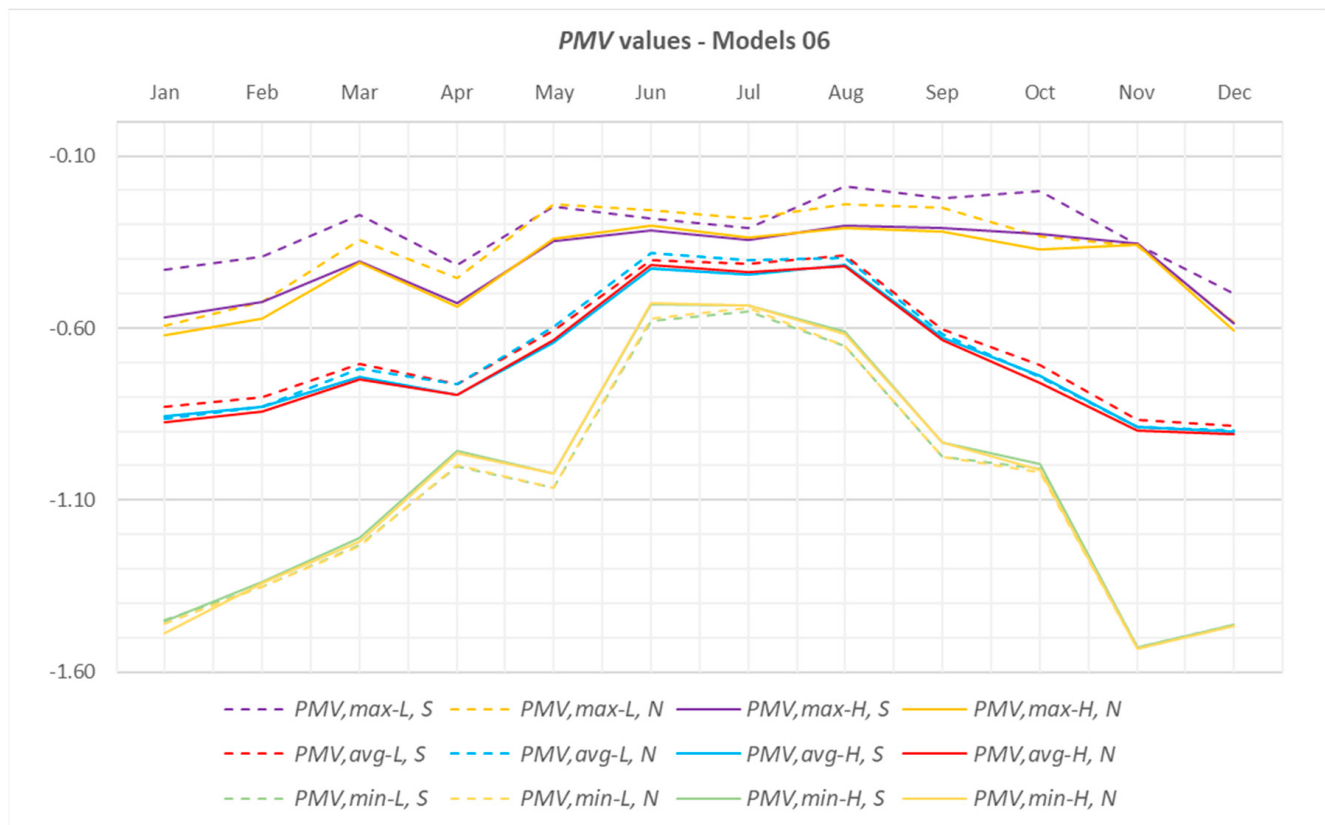
Figure 4. Monthly PMV simulation results for Models 06.
