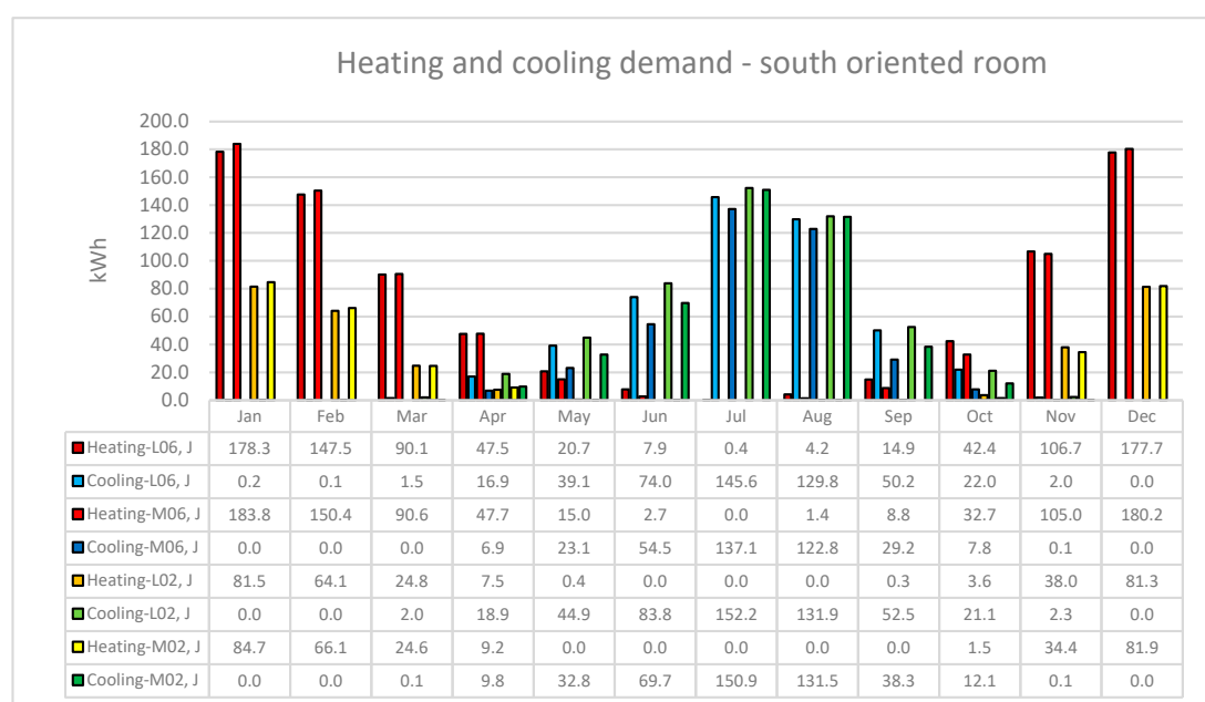
Figure 7. Monthly energy demand comparison for the south oriented room.
