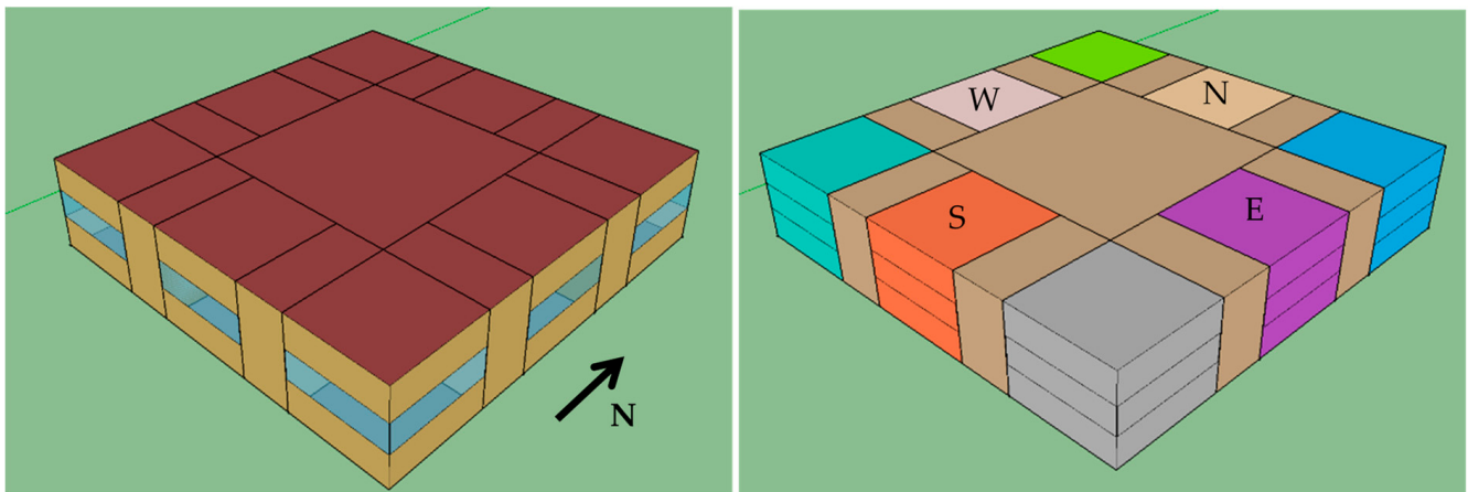
Figure 2. Visual presentation of the interim office floor simulation model and the analysed office cells facing the cardinal directions.
