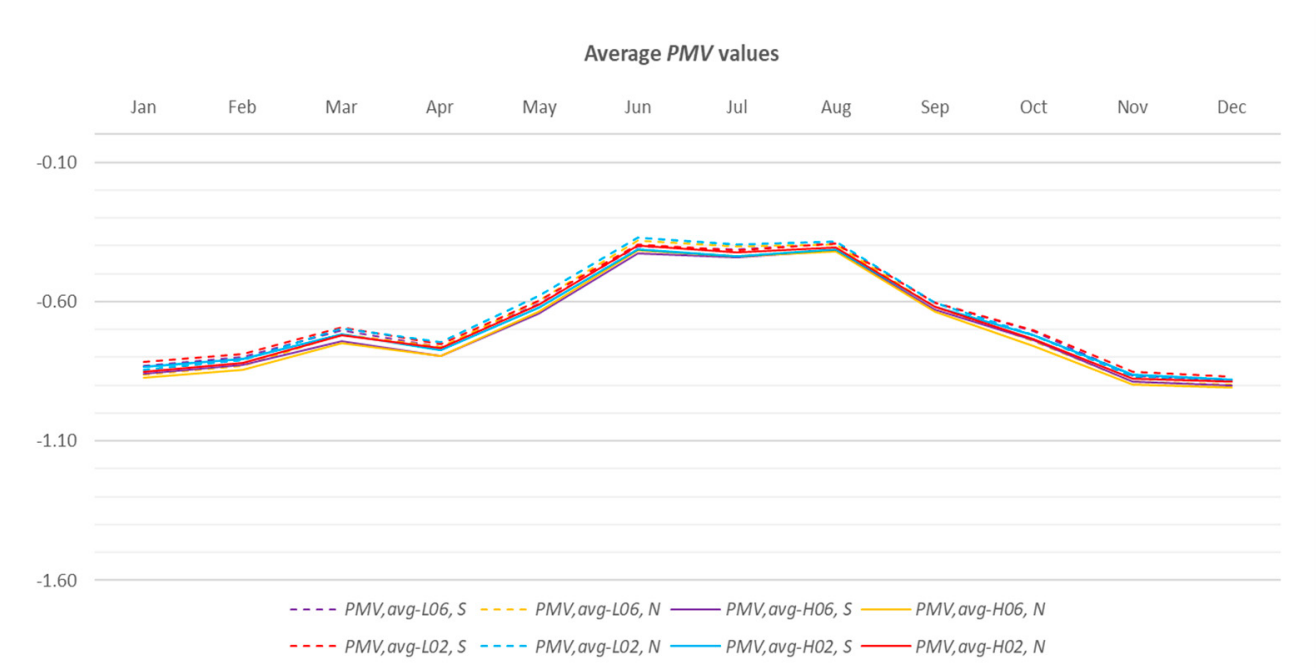
Figure 6. Average PMV values for the south and north oriented office cells of Models 06 and Models 02.
