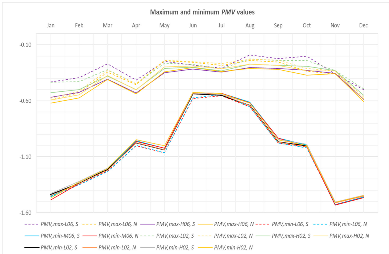
Figure 5. Maximum and minimum PMV values for the south and north oriented office cells of Models 06 and Models 02.
