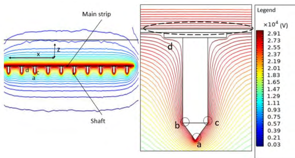
Figure 13. Potential contour of the spiked strip ground electrode.
