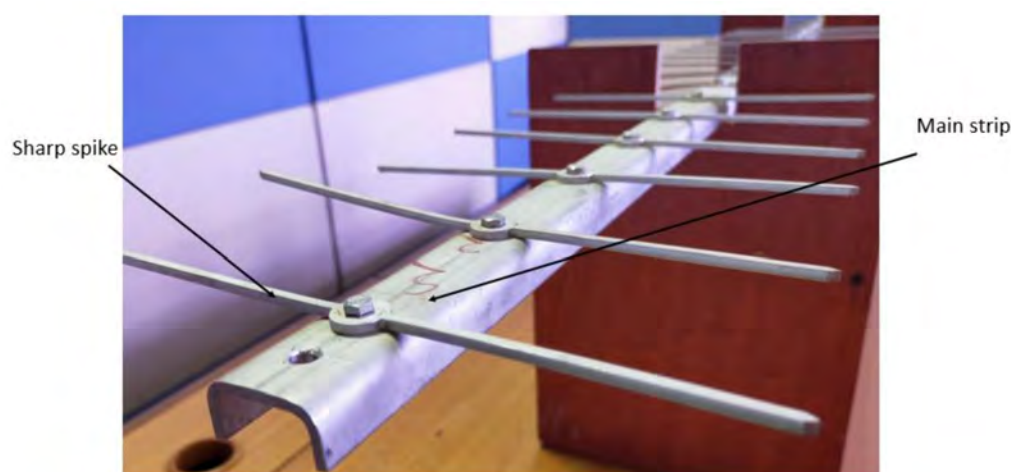
Figure 2. Linear array ground electrodes.
