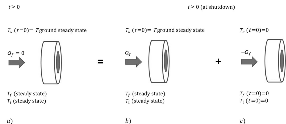
Figure 2. (a) total transient thermal process, (b,c), superposition of two elementary processes, to analyse the cooling of the pipe after shutdown.
