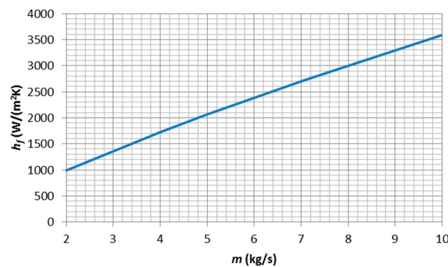
Figure 10. Convective heat transfer coefficient as a function of mass flow in the absorber.
