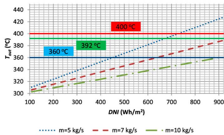
Figure 8. Medium temperature in the absorber at the outlet of a single loop as a function of mass flow and solar radiation (calculations performed for the conditions in Cordoba).
