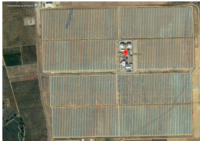
Figure 1. View of solar cylinder parabolic collectors at the Solar Thermal Power Plant “La Africana” (“satellite” view from googlemaps.com).
