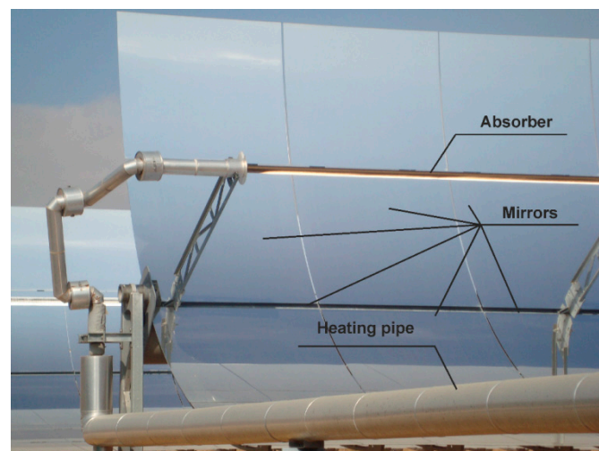
Figure 3. Detail of a cylindrical-parabolic solar collector of a Solar Thermal Power Station (photo by T.J. Teleszewski).
