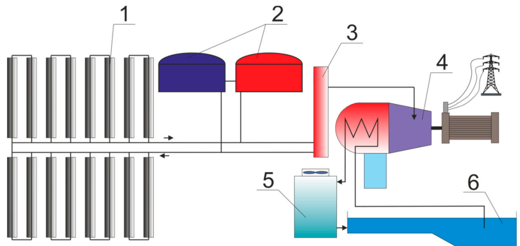
Figure 2. Simplified diagram of a thermal power plant with parabolic solar collectors: 1—parabolic solar collectors, 2—heat storage tanks, 3—steam generation system, 4—steam turbine, 5—cooling tower, 6—water storage reservoirs.
