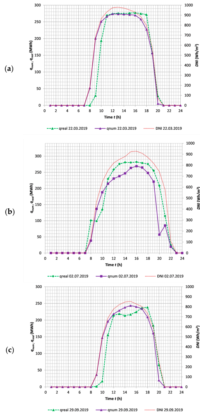
Figure 7. Comparison of heat produced by solar collectors with heat determined from the developed model the Solar Thermal Power Station in Spain for selected days: (a) 22.03.2019, (b) 02.07.2019, (c) 29.09.2019.
