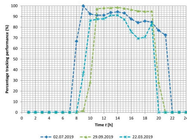
Figure 5. Percentage tracking performance compared to full tracking mode on selected days at the Solar Thermal Power Station in Spain.
