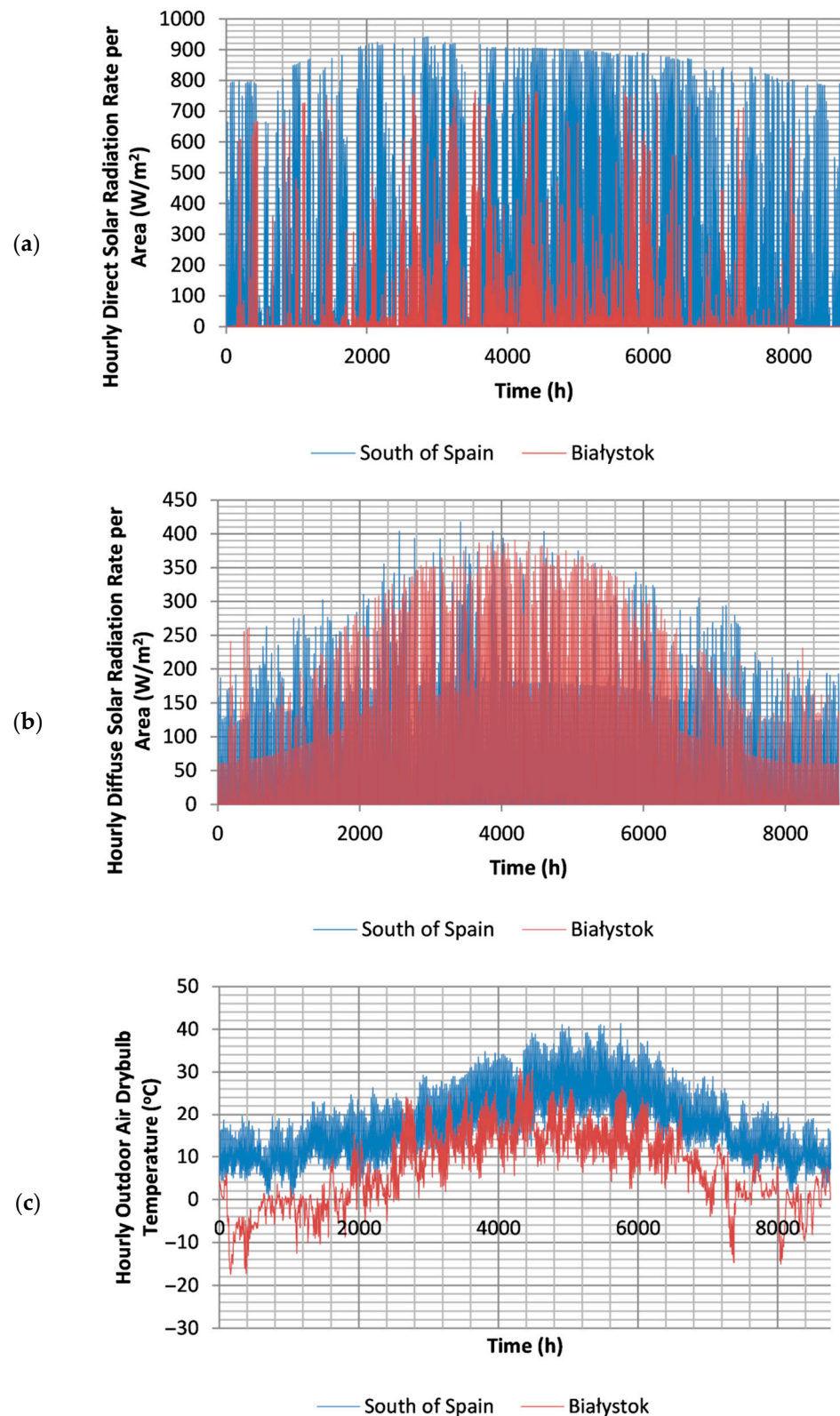
Figure 11. Hourly annual distribution of direct solar radiation (a), diffuse solar radiation (b) and outdoor temperature (c).
