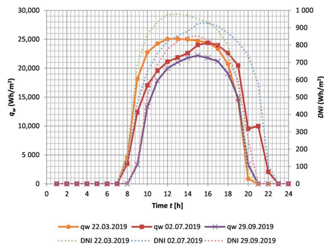
Figure 6. Calculated heat flux density per one square meter of an absorber and DNI for selected days for the Solar Thermal Power Station in Spain.
