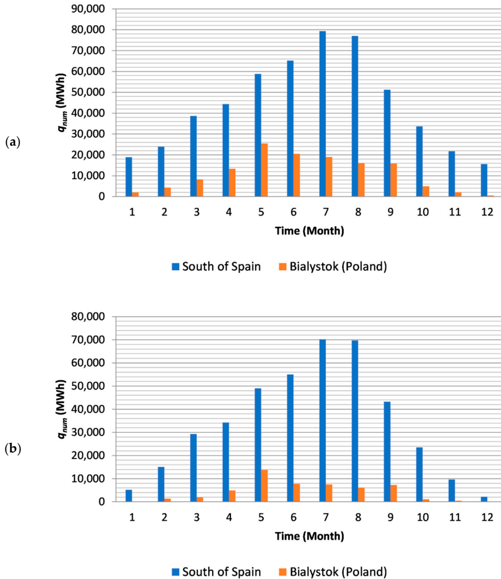
Figure 12. Annual heat produced by parabolic solar collectors for variants A (a) and B (b).
