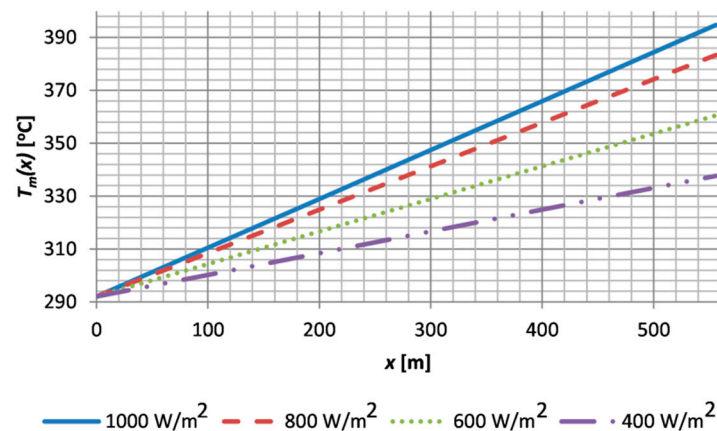
Figure 9. Temperature distribution of the medium flowing through the absorber as a function of the absorber length for different DNI.
