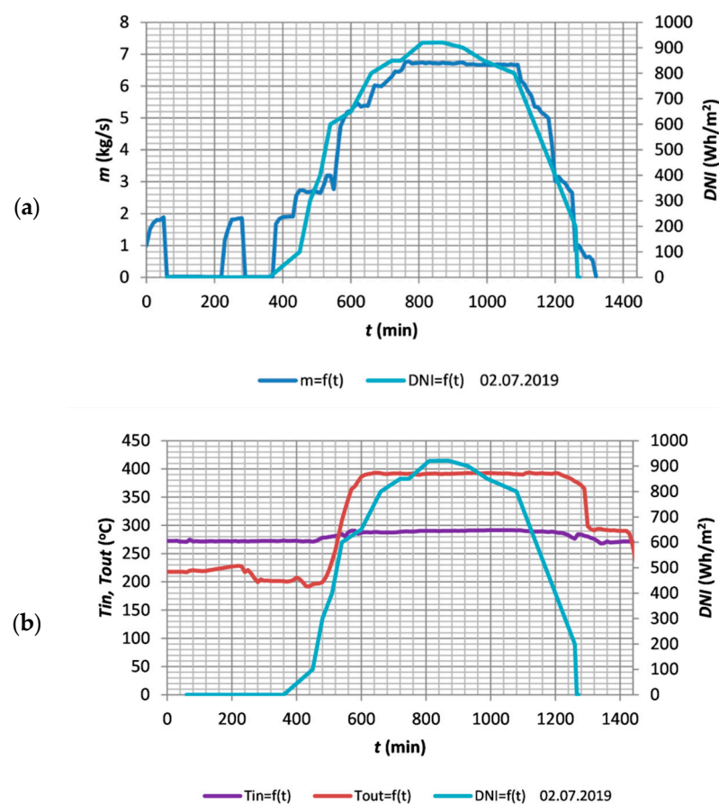
Figure 4. Changes in mass flow m (a) and temperature T_{in} and T_{out} (b) in a single loop on 02/07/2019 for the Solar Thermal Power Station in Spain.
