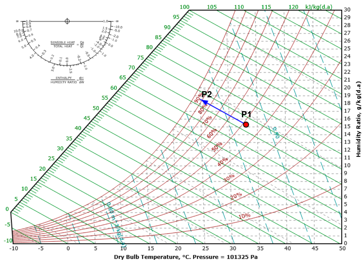
Figure 1. Example of efficiency of an evaporative system.
