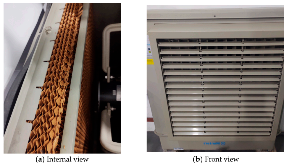
Figure 3. Munters FCA 5–20 evaporative equipment.
