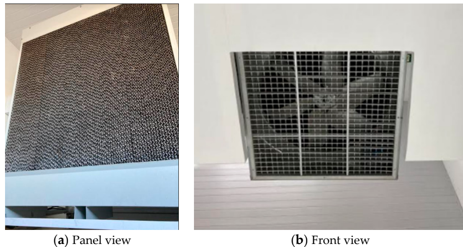
Figure 2. Munters Bb 150 evaporative equipment.
