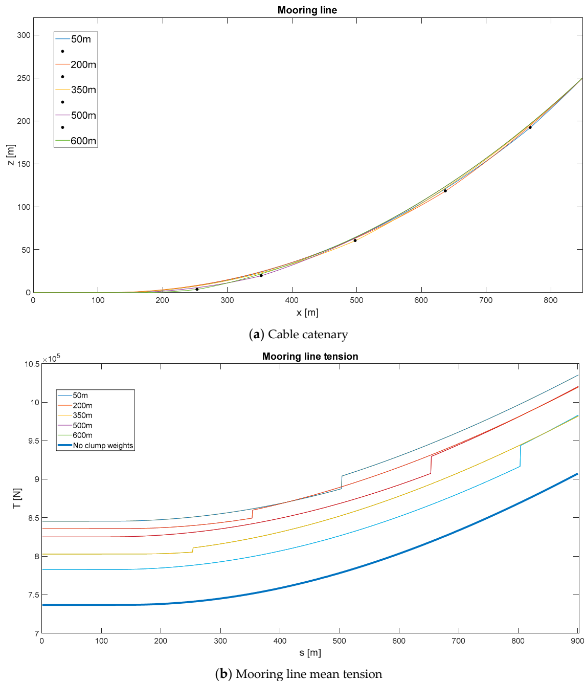
Figure 8. Cable catenary and mooring line tension depending on the ballast position ( M = 5 t).
