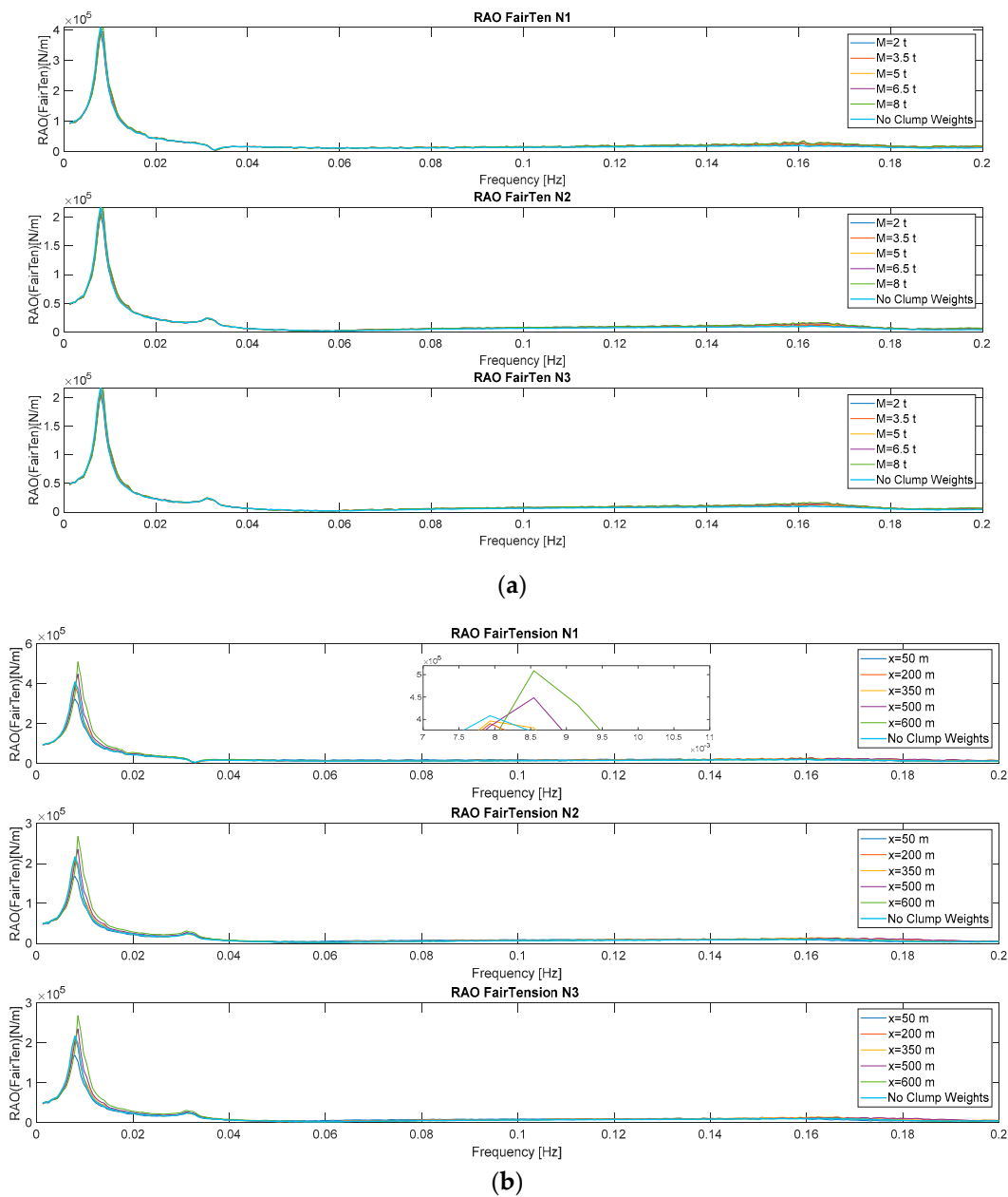
Figure 5. Fairlead Tension RAOs for different weights (a) and positions (b) of the cable ballast. Each figure shows the Fairlead Tension for every cable.
