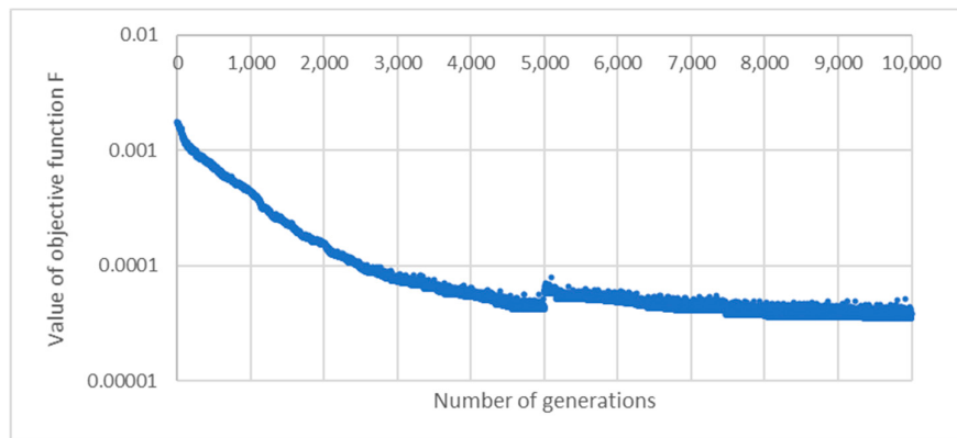
Figure 5. Objective function value against the number of evolution strategy generations for Case 1.1.
