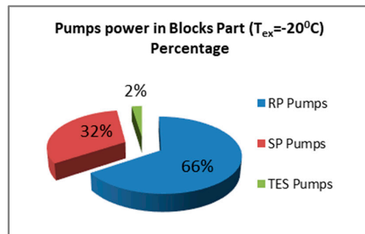
Figure 6. Percentage of pumps power for discharging of TES and temperature T_{ex} = -20^{\circ}\text{C} .
