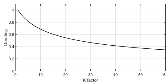
Figure 9. Transformer de-rated capacity depending on the K -factor.
