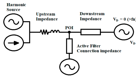
Figure 6. Simplified diagram for a harmonic active filter application considering harmonic voltage and current sources. Note: POI = point of inter-connection.
