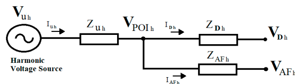
Figure 8. Simplified diagram of the active power filter application for series resonances.
