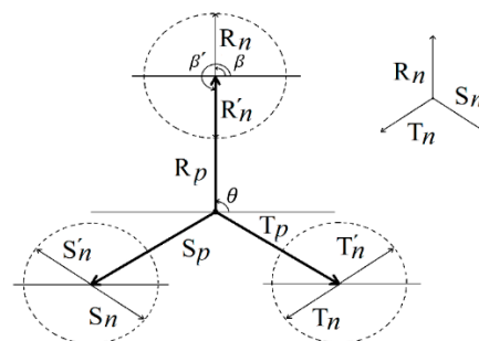
Figure 4. Diagram of positive and negative sequence vectors. The positive diagram with an arbitrary angle \theta is shown along with two cases for the negative sequence ( R_n T_n S_n and R'_n T'_n S'_n ). In the first case \beta is in phase with \theta and in the second case \beta' is in counter-phase with \theta .
