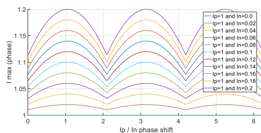
Figure 5. Maximum current out of the three phases for a 1 pu positive sequence current and a negative sequence current from zero to 0.2 pu (0.02 pu steps). \Theta = 0 , and \beta = 0-2\pi .
