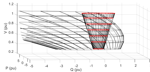
Figure 3. Inverter active and reactive power injection limits depending on the grid voltage. Voltage and current limits are shown separately, where the operational limit is the space within both limits.
