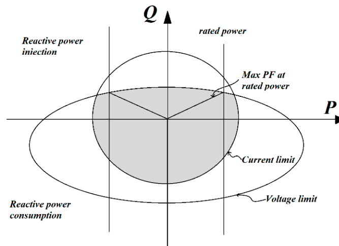
Figure 2. Inverter active and reactive power limits.
