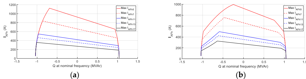
Figure 11. Maximum current at nominal voltage for different harmonics and injected reactive power: (a) considering a correctly sized transformer and (b) considering a transformer designed with K < 2 .
