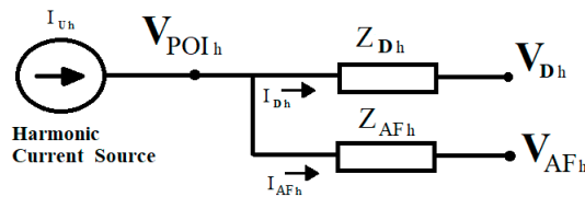
Figure 7. Simplified diagram of the active power filter application for parallel resonances.
