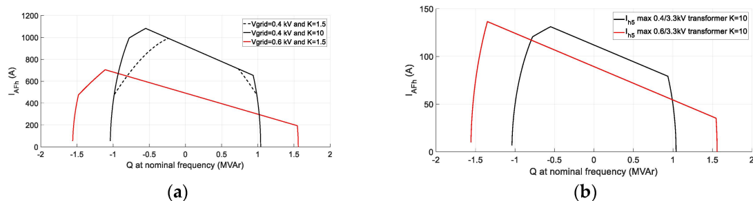
Figure 12. Maximum 5th order current limit at nominal voltage for a 400 V and 600 V nominal grid voltage: (a) current at the LV side of the transformer and (b) current at the MV side of the transformer.
