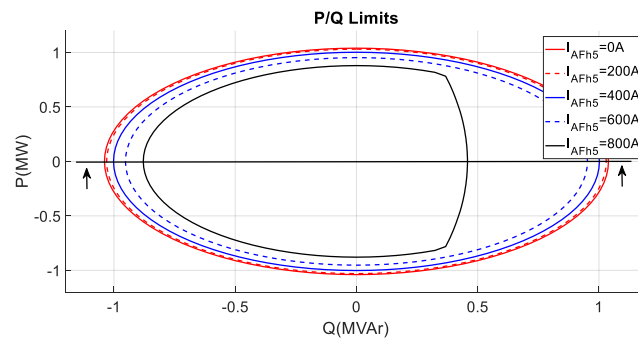
Figure 13. Maximum active and reactive power injection capability for different injected 5th harmonic current values (DHC) at nominal voltage (400 V).
