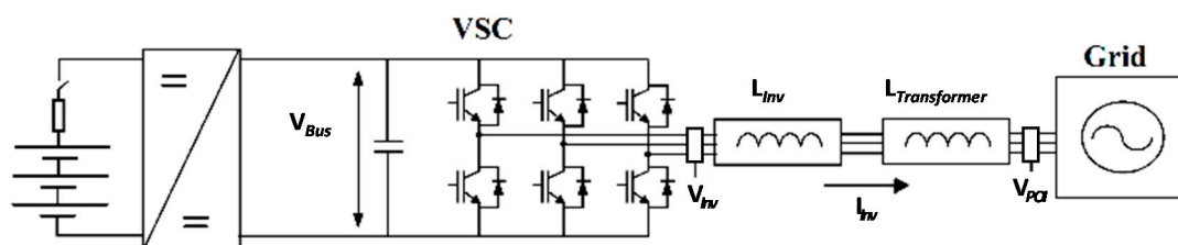
Figure 1. Power conversion system configuration. V_{Bus} represents the dc-link voltage, V_{Inv} is the converter voltage, V_{PCI} is the connection point voltage and I_{Inv} is the converter current. L_{Inv} is the equivalent converter filter inductance and L_{Transformer} is the short-circuit inductance of the grid connection transformer. VSC is the voltage source converter.
