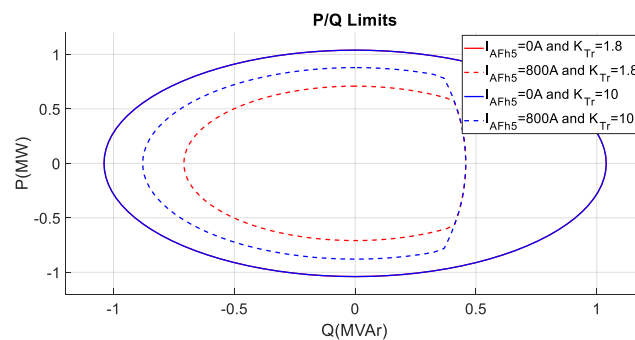
Figure 14. Maximum active and reactive power injection capability for two 5th harmonic currents (DHC) of 0 and 800 A at nominal voltage. In order to show the de-rating effect, two different k -factors for the transformer are considered.
