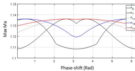
Figure 10. Maximum modulation index (Max Ma: inverter voltage) for a B = 40\% and h = 5 th, 7th, 11th, 13th and 17th voltage harmonics for a PWM modulation with a 3rd harmonic. Maximum modulation index value for all possible phase shifts ( \beta = 0-2\pi ).
