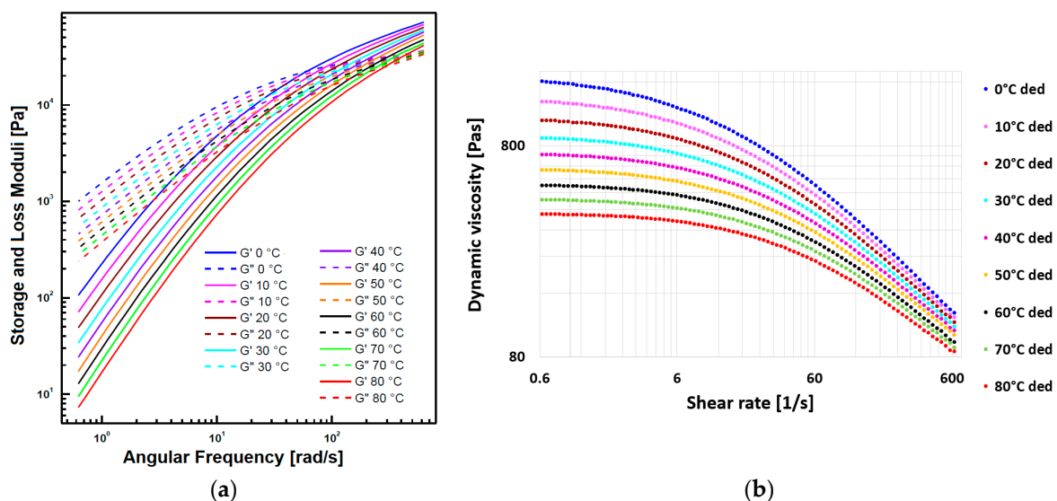
Figure 3. (a) Measured storage and loss moduli data of Small Amplitude Oscillatory Shear (SAOS) tests (reproduced with permission from Z. Kőkuti [13]). (b) Deduced dynamic viscosity data in 96 selected shear rates, at each temperature.
