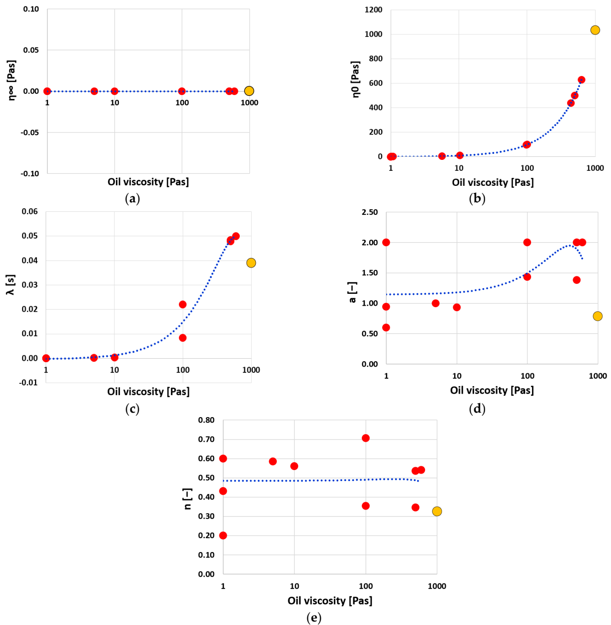
Figure 6. Validation of model parameters (orange dots) with parameter data available in the literature (red dots) with fitted trend line (dotted blue line) for (a) infinite-shear dynamic viscosity, (b) zero-shear dynamic viscosity, (c) relaxation time, (d) transition control factor and (e) power law index.
