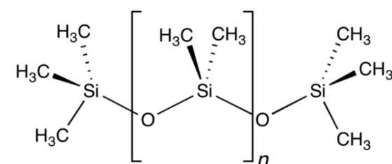
Figure 1. The constitutional formula of polydimethylsiloxane.
