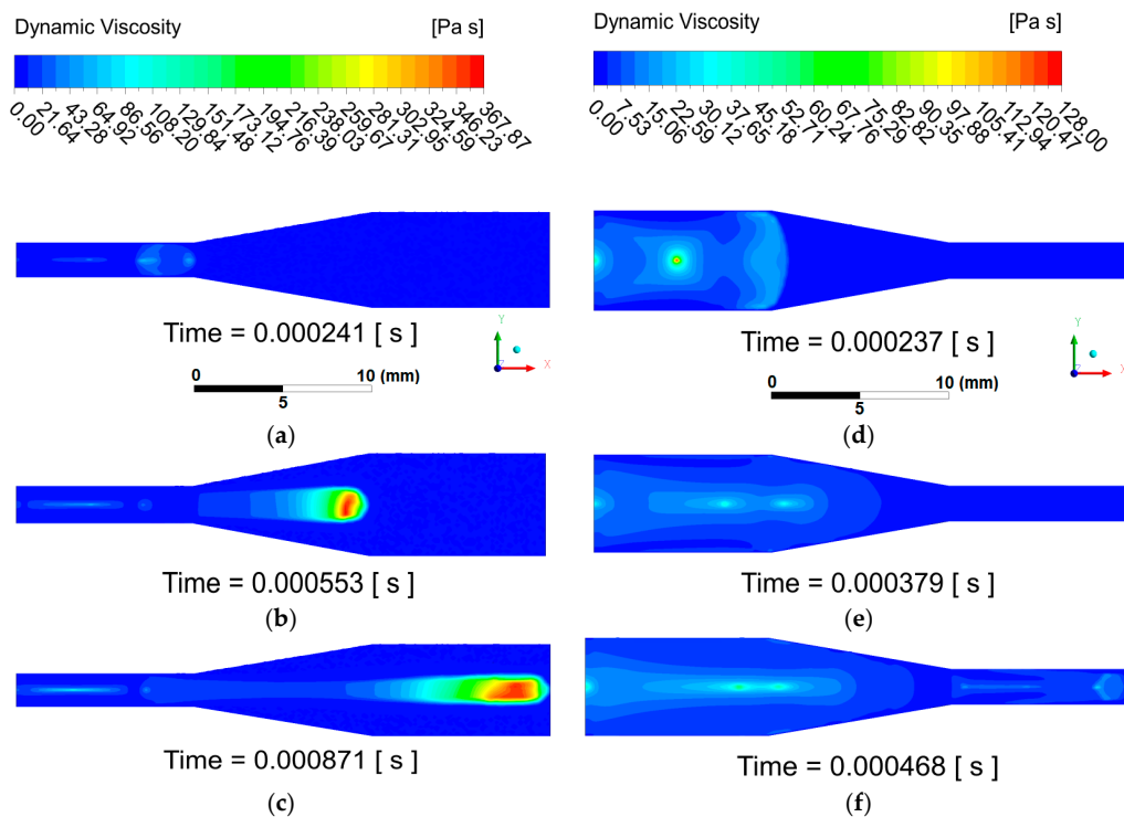
Figure 11. Dynamic viscosity results of (a) diffuser case in the first selected timestep, (b) diffuser case in the second selected timestep, (c) diffuser case in the third selected timestep, (d) confusor case in the first selected timestep, (e) confusor case in the second selected timestep and (f) confusor case in the third selected timestep.
