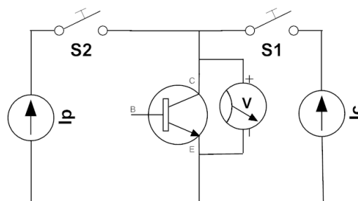
Figure 2. Circuit used in direct and thermo-sensitive electrical parameter (TSEP)-based temperature measurement.
