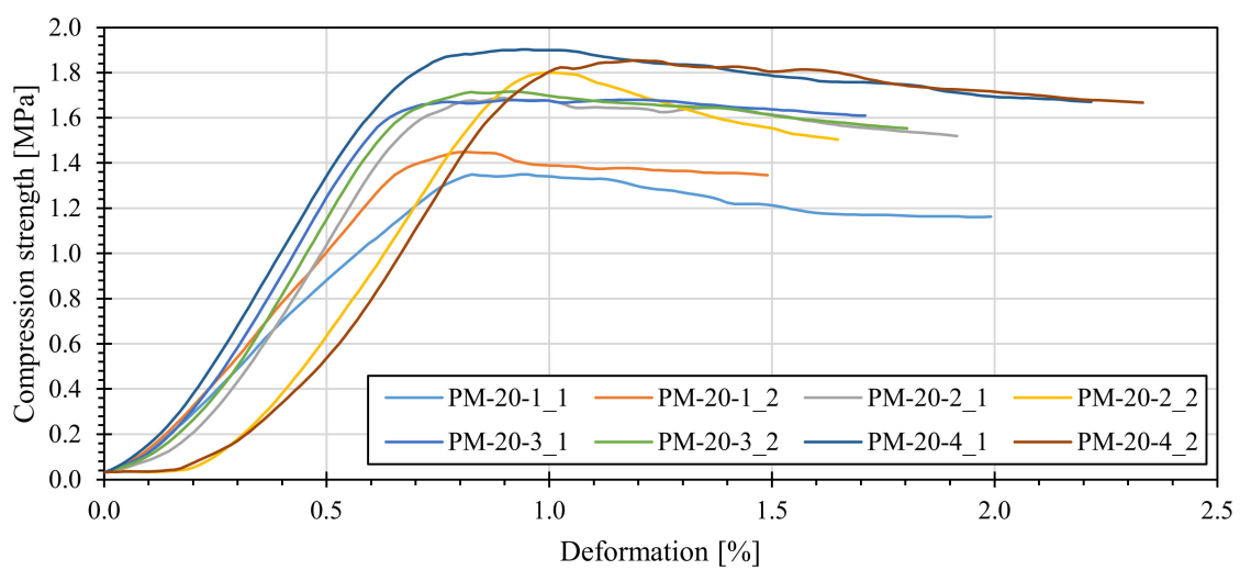
Figure 9. Compression strength PM-20.
