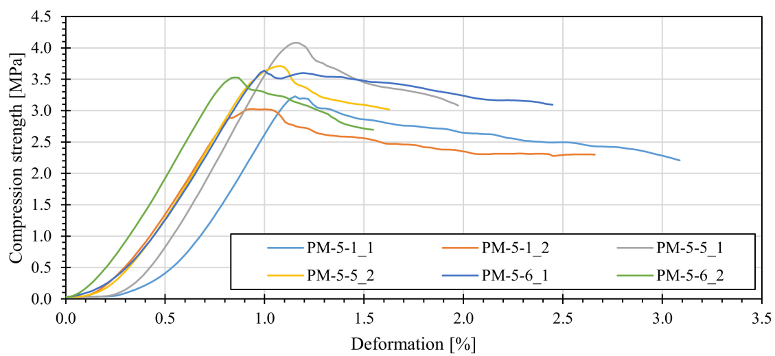
Figure 7. Compression strength PM-5.
