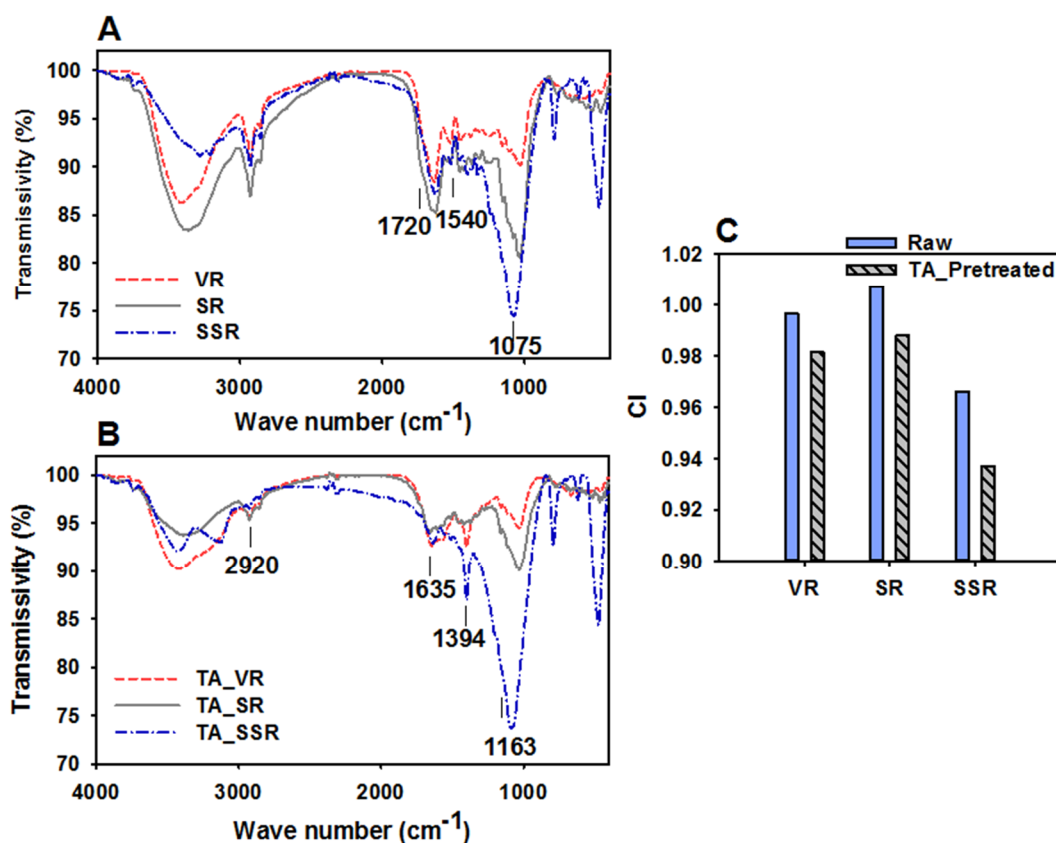
Figure 1. FTIR spectra and crystallinity indexes (CI) of the three PWs, (A) for raw PWs, (B) for pretreated PWs, (C) for CI of the raw and pretreated PWs.
