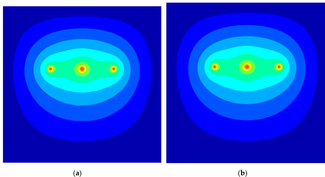
Figure 8. Temperature distribution around the heaters for T_{air} = 40\text{ }^{\circ}\text{C} and P = 20\text{ W} (a), and T_{air} = 3.7\text{ }^{\circ}\text{C} and P = 20\text{ W} .
