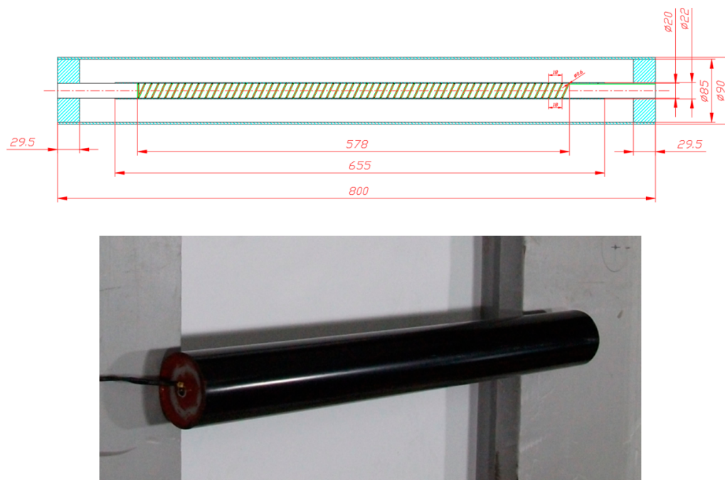
Figure 3. A view of the electric heater.
