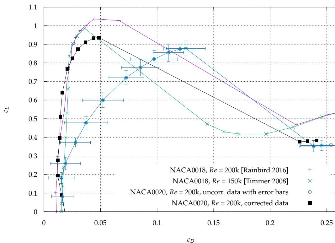
Figure 6. Comparison of corrected and uncorrected polars from our study with two similar flapless profiles from the literature; the uncorrected polar includes error bars with standard deviation.
