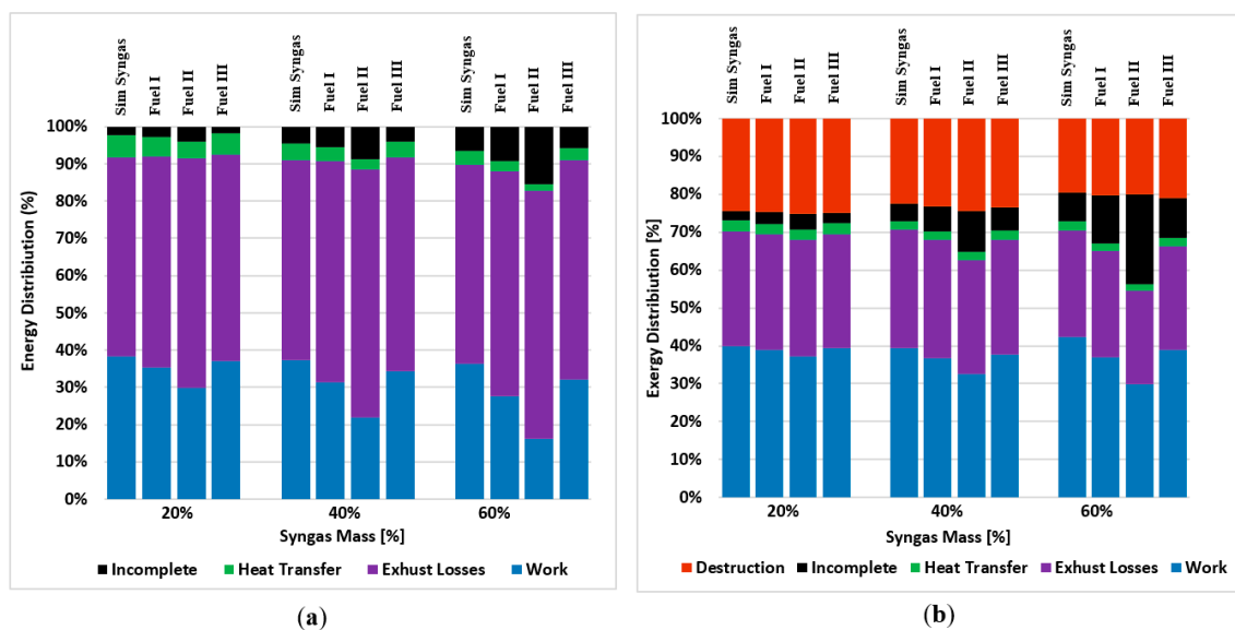
Figure 10. Energy (a) and exergy (b) distributions of the four fuels at various syngas masses.
