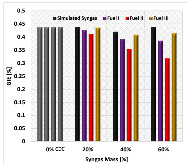
Figure 7. Thermal efficiency for the studied RCCI Engine fed by various fuel mixtures.
