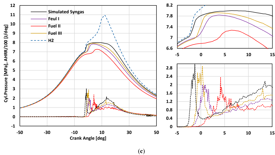
Figure 4. Cylinder pressure and HRR for RCCI engine fueled with diesel and different syngas mixtures with varying syngas substitution ratios in constant energy per cycle for syngas, (a) 20%; (b) 40%; (c) 60%.
