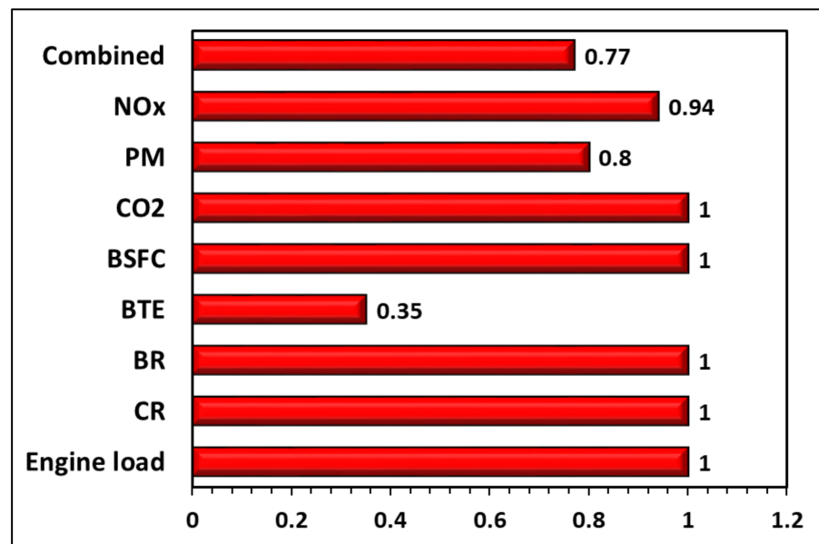
Figure 12. Bar graph for desirability.
