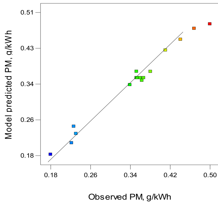
Figure 5. Observed and predicted PM (g/kWh).
