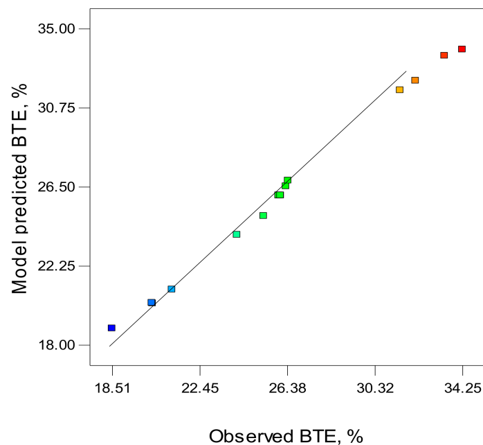
Figure 2. Observed vs. MORSM predicted BTE (%).
