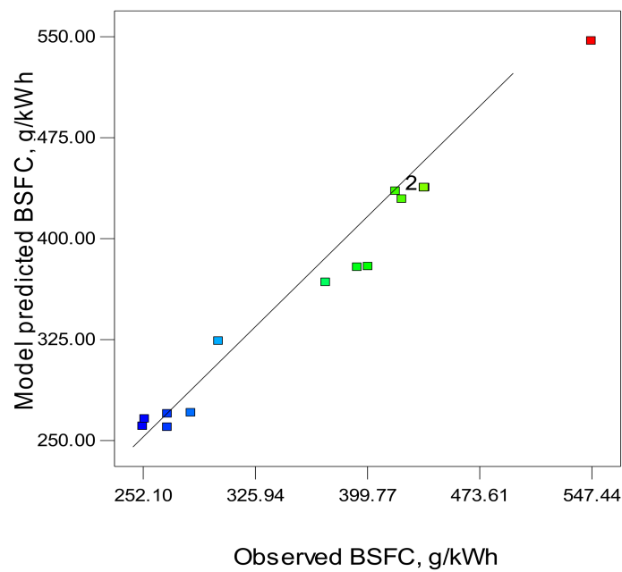
Figure 3. Observed vs. predicted BSFC (g/kWh).
