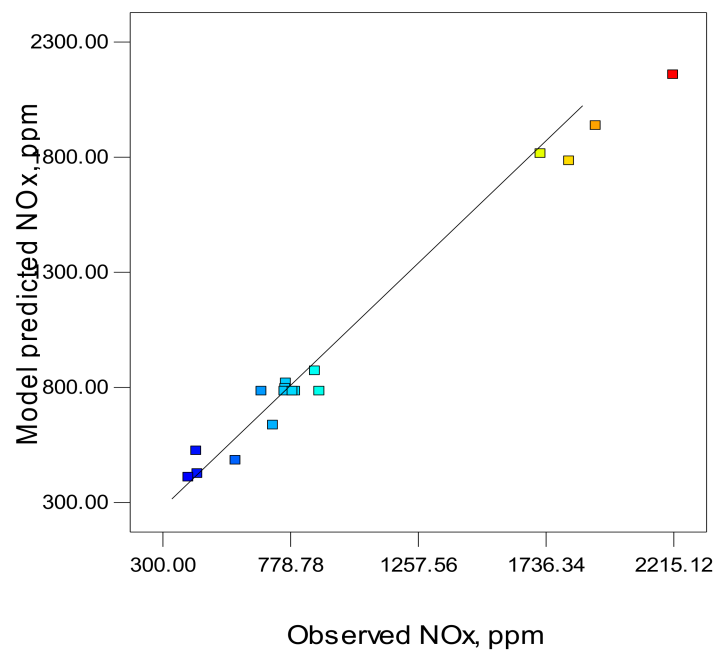
Figure 6. Observed and predicted NOx (ppm).
