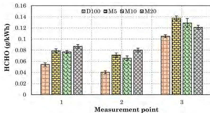
Figure 14. Specific HCHO emissions for all test fuels at all measurement points (error bars represent the standard deviation).
