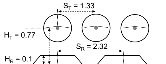
Figure 1. Geometric specifications of the ETC investigated with respect to the outer tube diameter.
