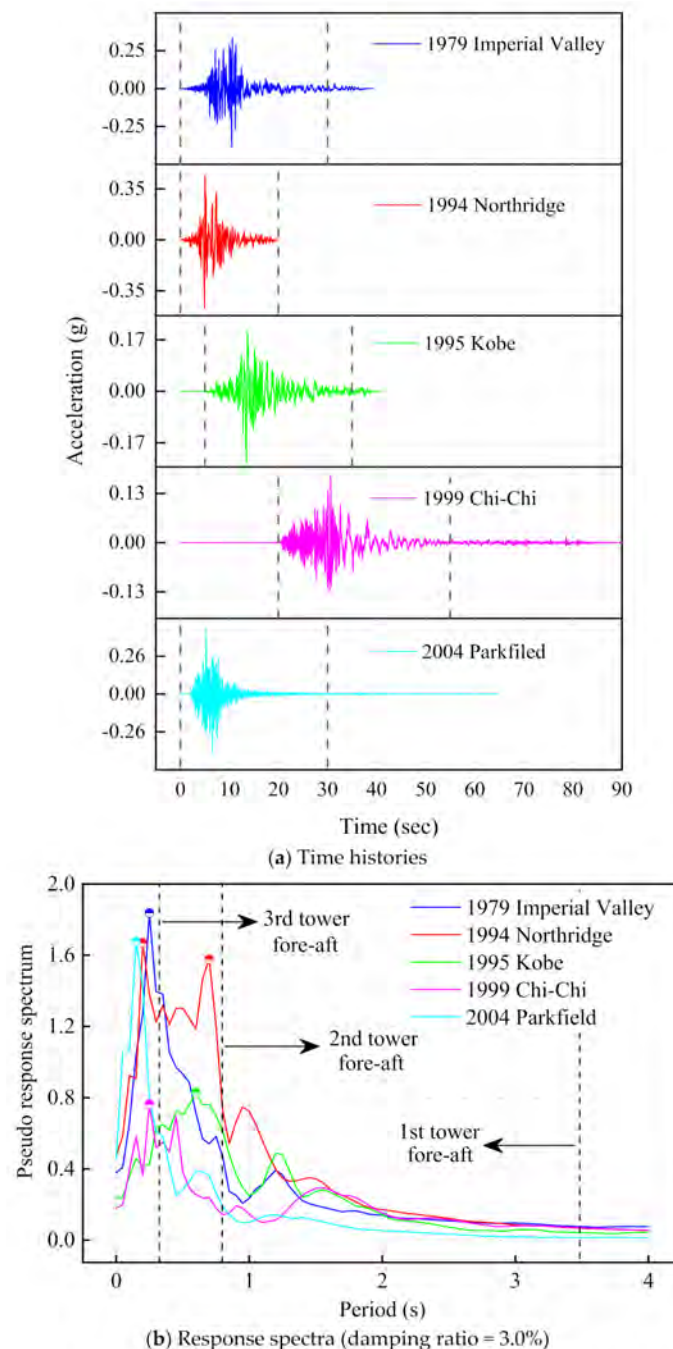
Figure 6. Acceleration time histories and response spectra of five selected ground motion records.
