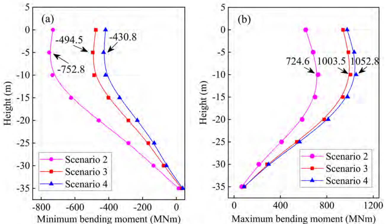
Figure 13. Bending moment distributions along the monopile under the Kobe earthquake (a) Minimum bending moment; (b) Maximum bending moment.
