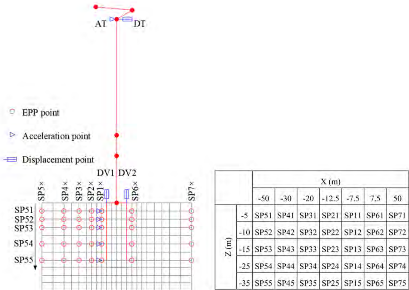
Figure 8. Monitoring points in dynamic response and liquefaction analysis.
