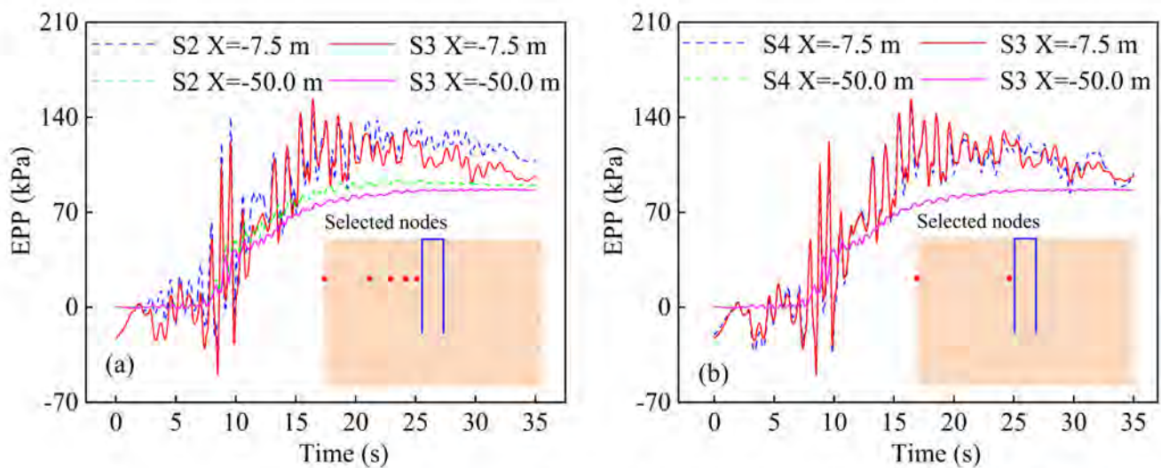
Figure 15. EPP comparison of soil nodes with different distances from the pile under Kobe earthquake in: (a) Scenarios 2 and 3; and (b) Scenarios 3 and 4.
