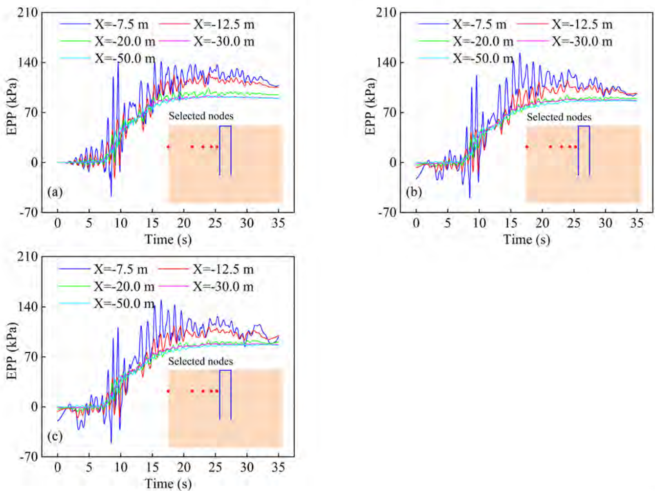
Figure 12. EPP of soil nodes with different distances from the pile under Kobe earthquake: (a) EPP accumulation in Scenario 2; (b) EPP accumulation in Scenario 3; and (c) EPP accumulation in Scenario 4.
