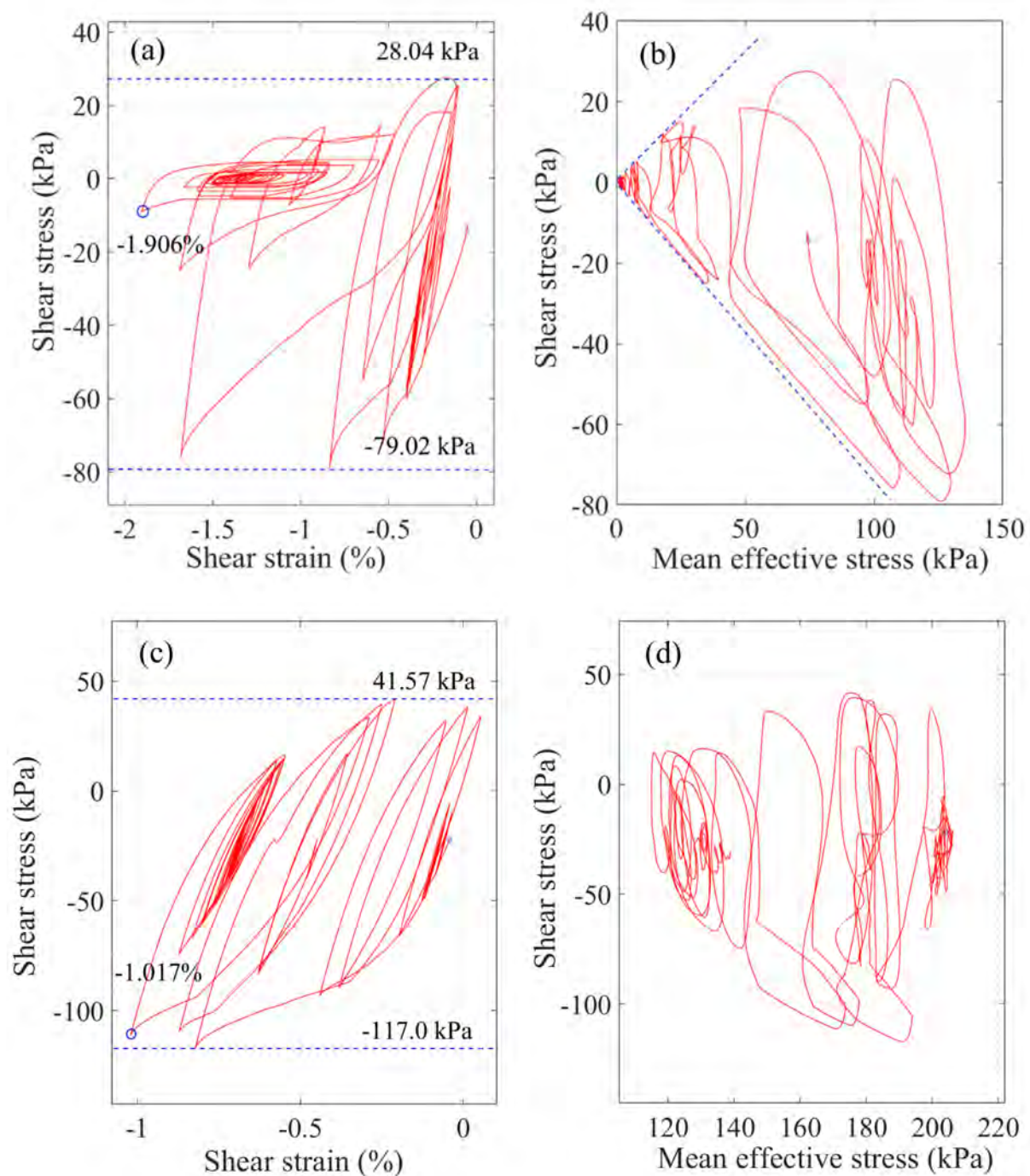
Figure 17. Shear stress–strain and shear stress–mean effective stress relationships of soil nodes around the piles under Kobe earthquake in Scenario 3: (a) shear stress–strain relationship at Z = -10 m; (b) shear stress–mean effective stress relationship at Z = -10 m; (c) shear stress–strain relationship at Z = -25 m; and (d) shear stress–mean effective stress relationship at Z = -25 m.
