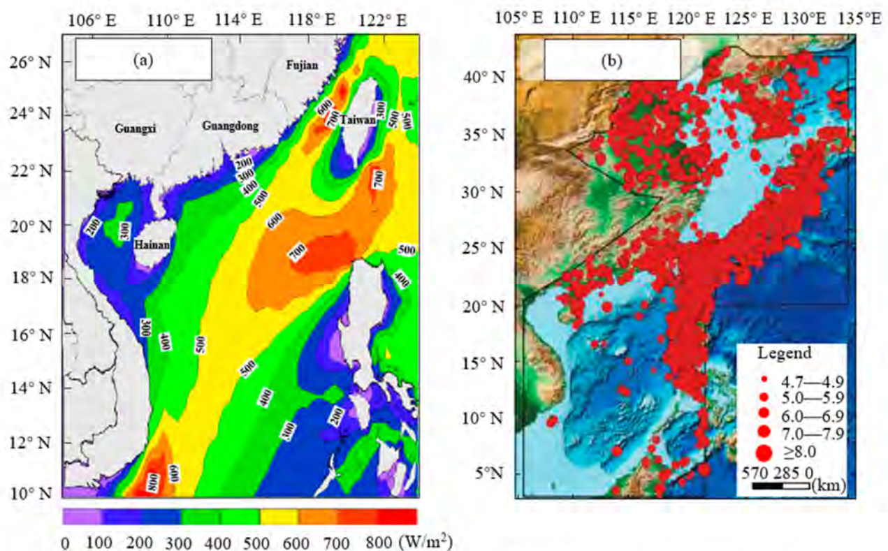
Figure 2. Wind power and earthquake distribution in the South China Sea: (a) the average wind power density (1979–2016) [13]; and (b) seismic epicenter distribution (BC1767–2018) [14].
