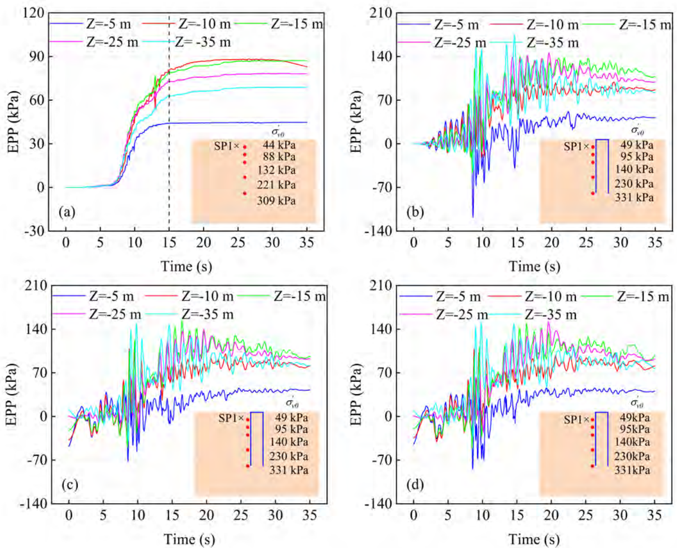
Figure 10. EPPs at different depths ( Z ) under the Kobe earthquake: (a) Free-field in Scenario 1; (b) WT system in Scenario 2; (c) WT system in Scenario 3; and (d) WT system in Scenario 4.
