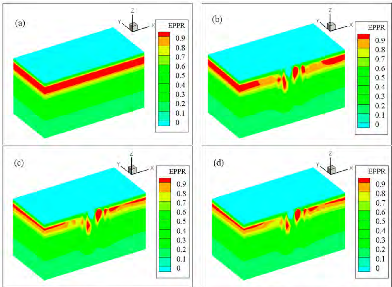
Figure 11. Liquefaction distribution of the soil domain under the Kobe earthquake: (a) Free-field in Scenario 1; (b) WT system in Scenario 2; (c) WT system in Scenario 3; and (d) WT system in Scenario 4.
