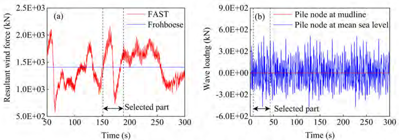
Figure 5. Environment loading: (a) wind loading imposed at the hub; and (b) wave loadings on pile nodes.
