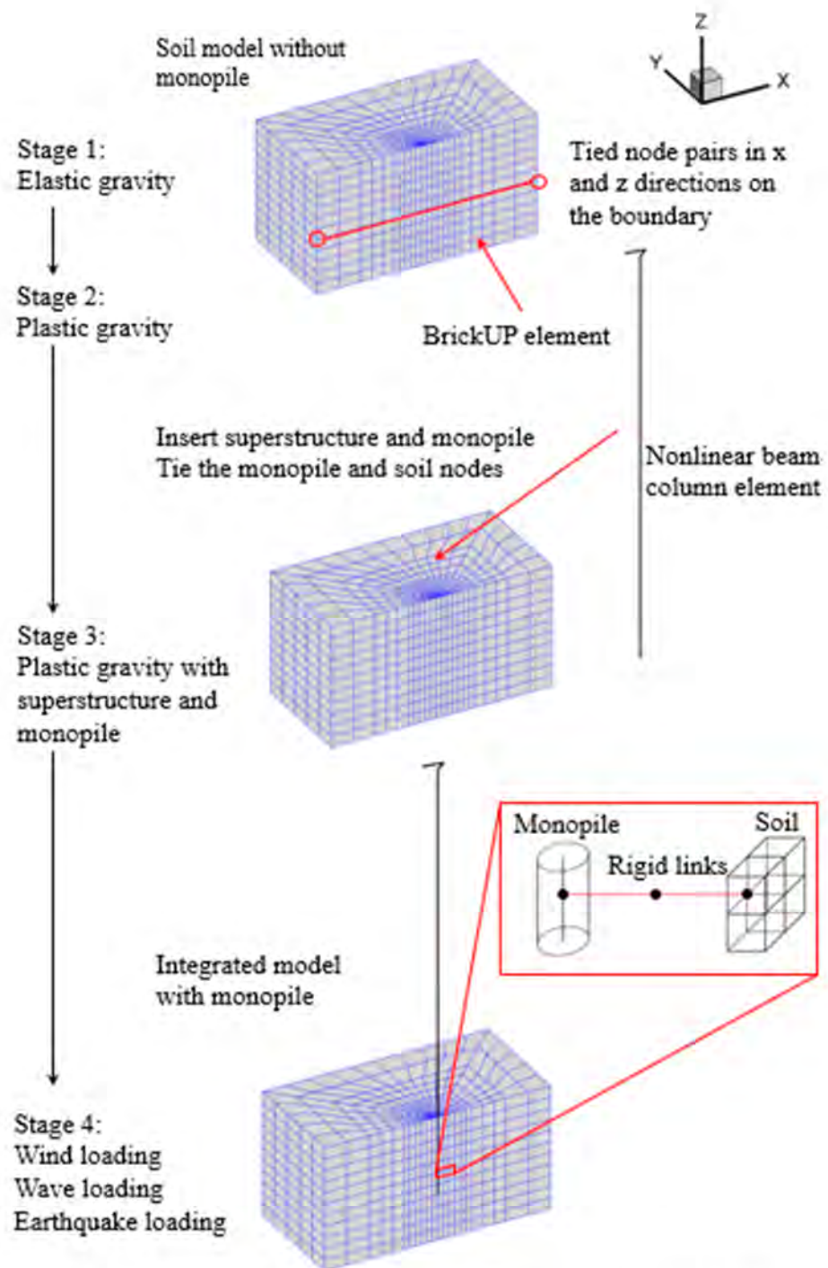
Figure 7. Simulation procedure for the OWT system in liquefiable soil.
