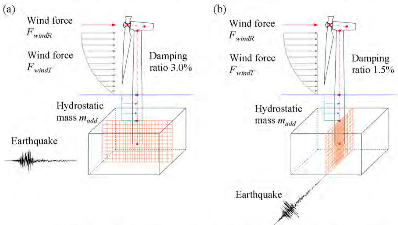
Figure 9. OWT model considering different earthquake induction directions in Scenario 3: (a) Case 1; and (b) Case 2.
