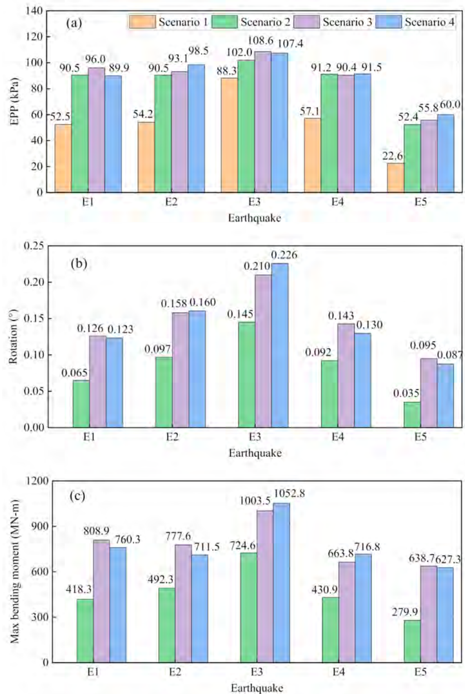
Figure 16. Comparison of various performance indices among four scenarios: (a) EPP of soil node with a depth of 10 m; (b) pile rotation angle at the mudline; and (c) maximum bending moment along the pile.
