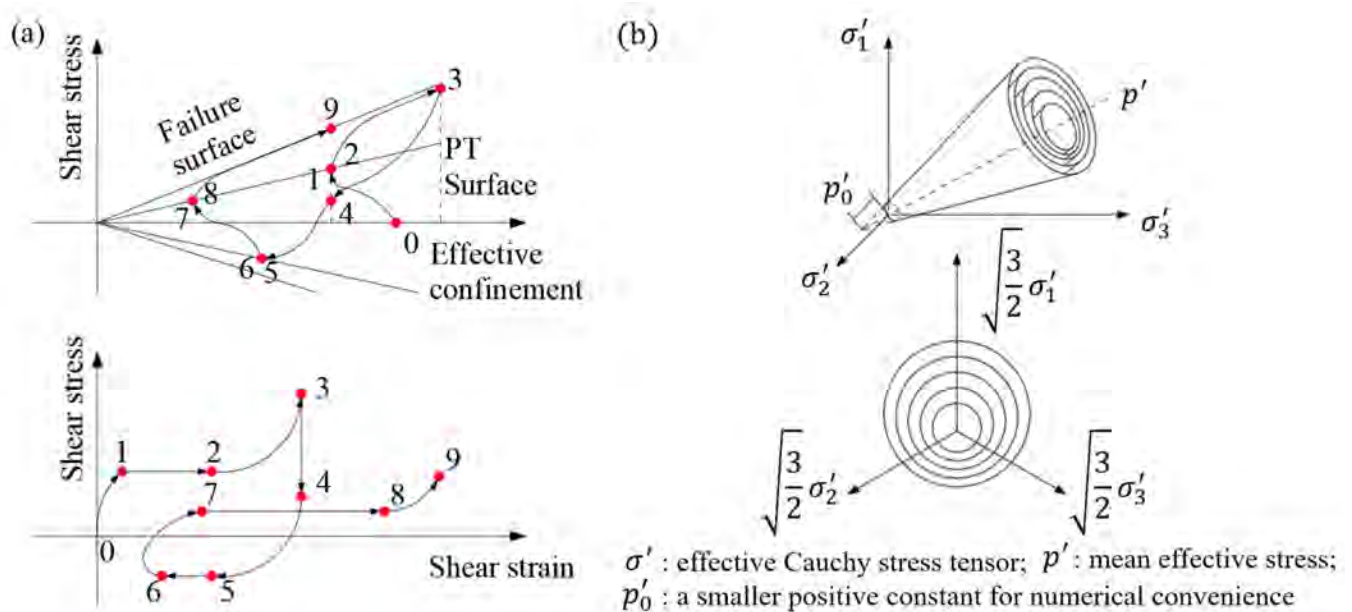
Figure 4. Constitutive model of PressureDependentMultiYield material [81]: (a) schematic of the constitutive model; and (b) conical yield surfaces in principal stress space and deviatoric plane.
