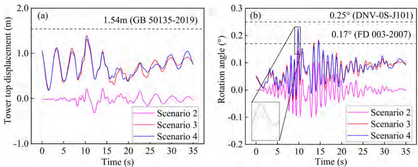
Figure 14. Tower top displacement and pile rotation under the Kobe earthquake in Scenarios 2–4: (a) tower top displacements; and (b) pile rotation angles at the mudline.
