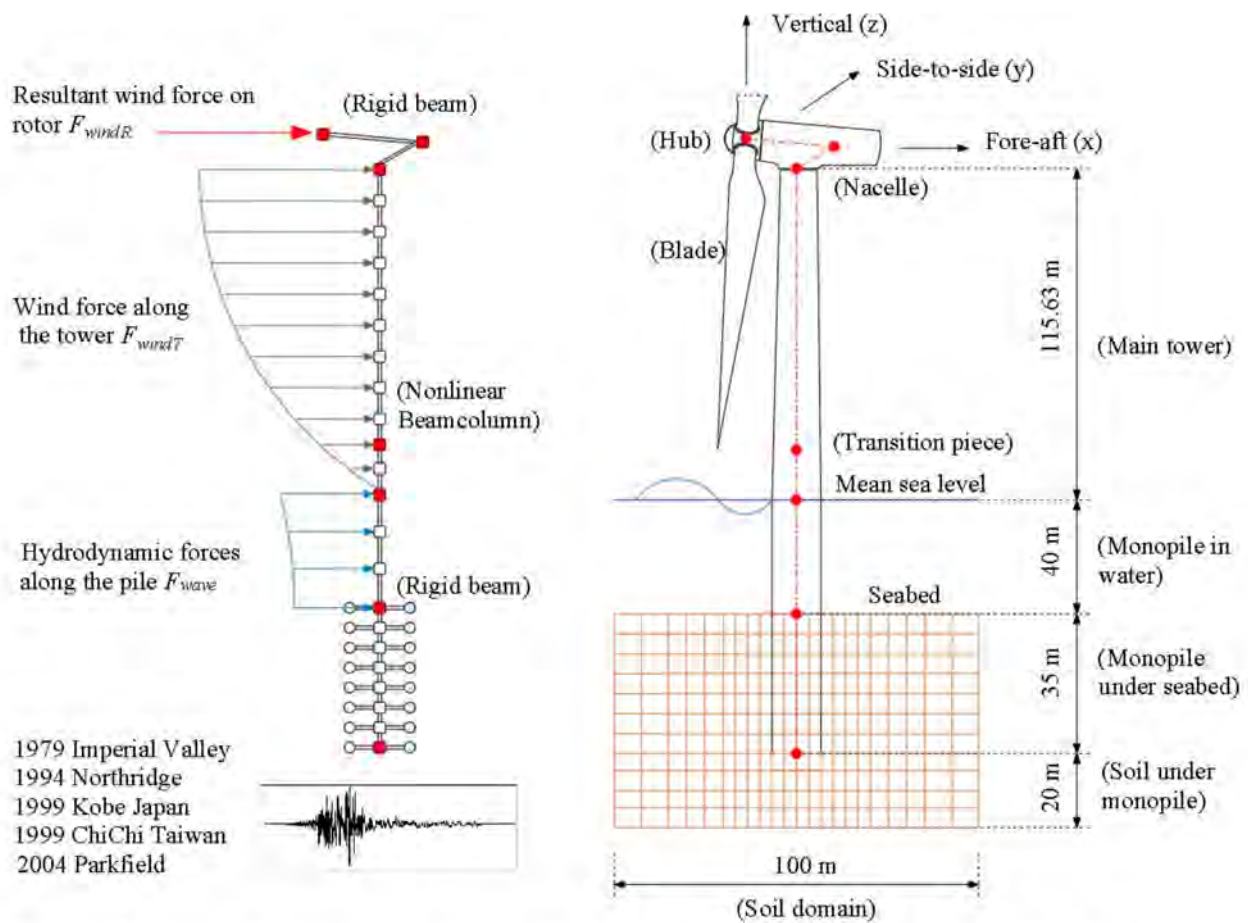
Figure 3. Schematic representation of the OWT model and environmental loading.
