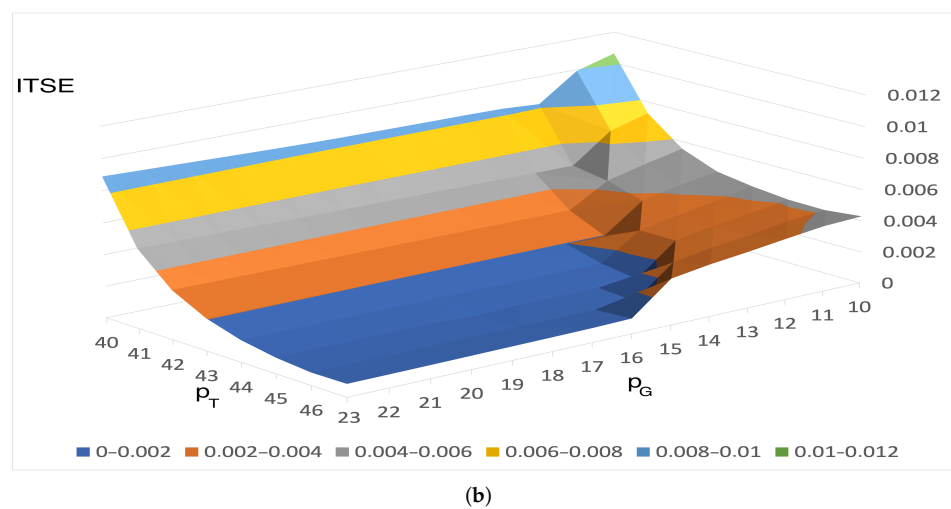
Figure 7. Indices for a = 1, b = 1, c = 1 [\cdot 10^{-2}] ; (a) ISE, (b) ITSE.
