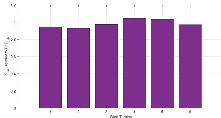
Figure 26. Normalised D_{ratio} using wind rose data only for a range of wind turbines.
