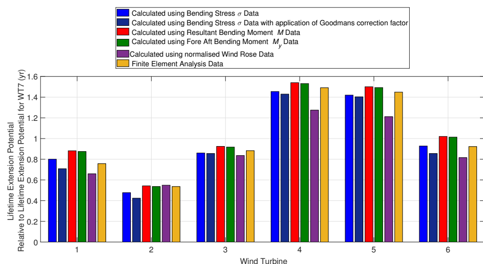
Figure 28. Relative lifetime extension potential for a range of scenarios range of wind turbines.
