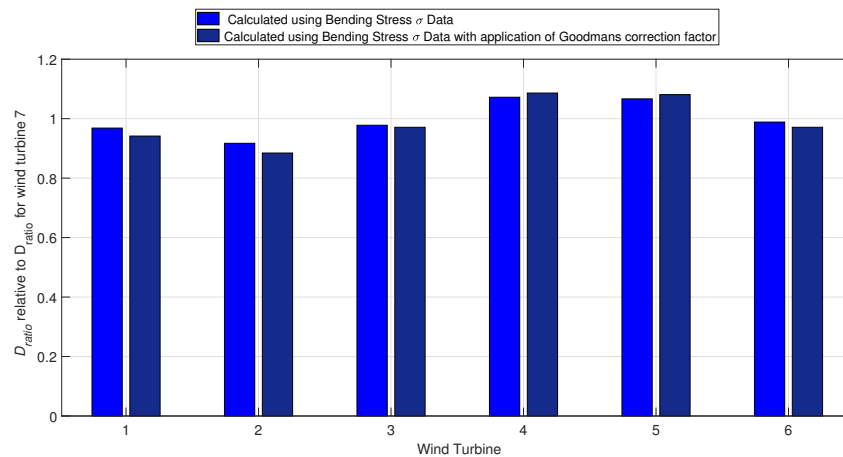
Figure 25. Normalised D_{ratio} using bending stress \sigma with and without the application of the Goodman's correction factor for a range of wind turbines.
