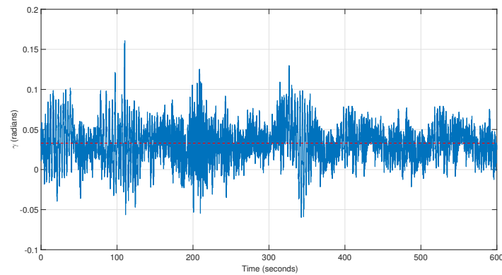
Figure 10. Deviation \gamma for rated wind speed (10 m/s).
