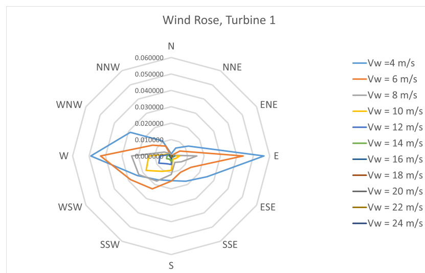
Figure A2. Wind Rose 1—wind speed and wind direction probability for wind turbine 1 with prevailing wind direction.
