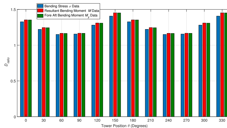
Figure 20. Absolute D_{ratio} between uni-directional fatigue damage and fatigue damage at a range of tower positions \theta for wind rose 1.
