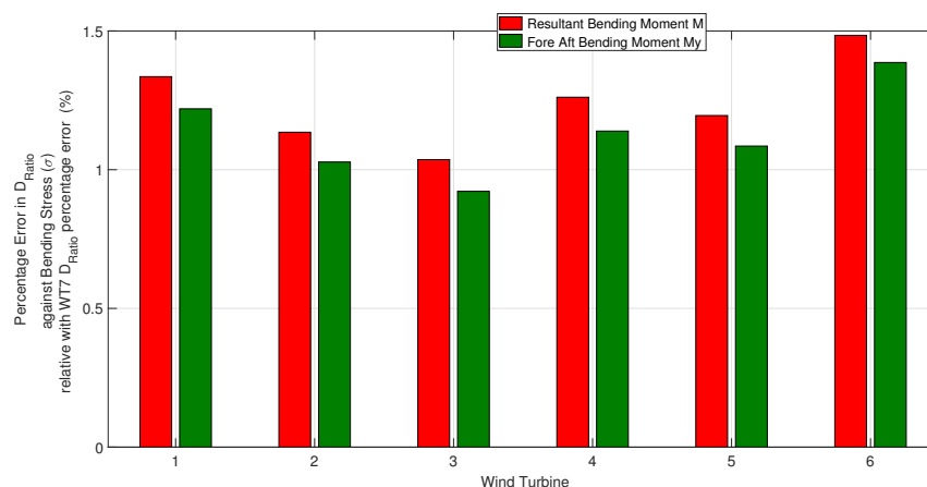
Figure 24. Percentage difference in normalised D_{ratio} between resultant bending moment M and fore-aft bending moment M_y and bending stress \sigma , for a range of wind turbines.
