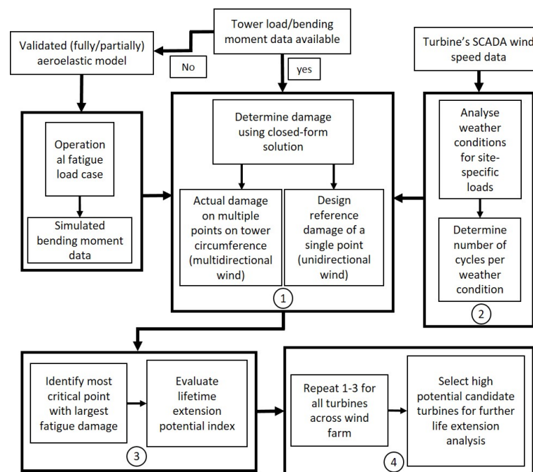
Figure 1. Flowchart of lifetime extension potential assessment [15].
