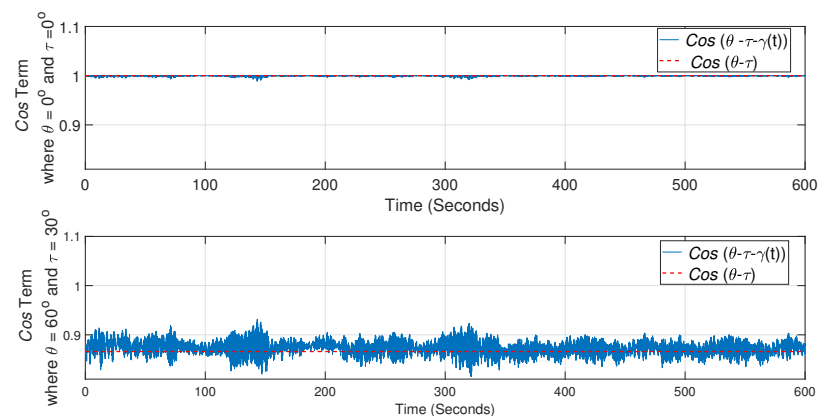
Figure 12. Cos term evaluation for a below-rated wind speed (6 m/s) for set \theta = 0^\circ , \tau = 0^\circ (above) and for set \theta = 60^\circ , \tau = 30^\circ (below).
