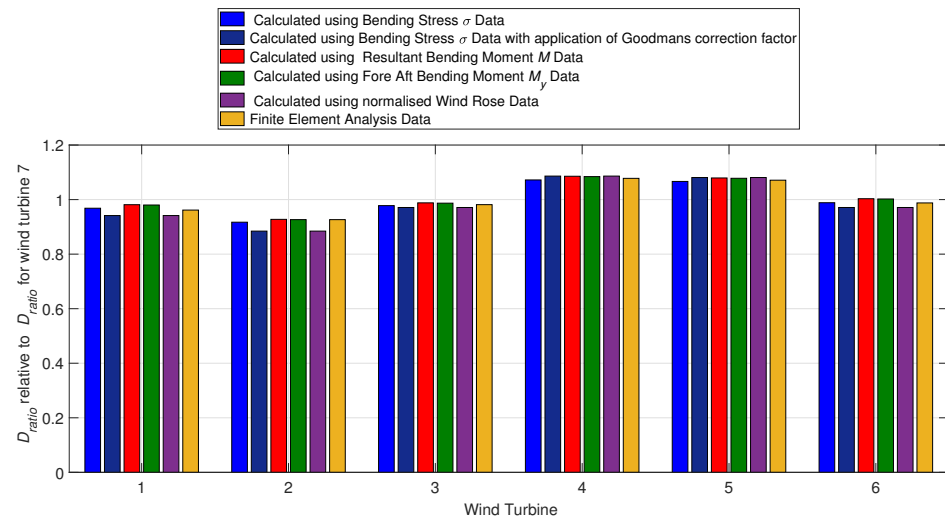
Figure 27. Normalised D_{ratio} results for a range of scenarios compared to relative D_{ratio} calculated using finite element analysis for a range of wind turbines.
