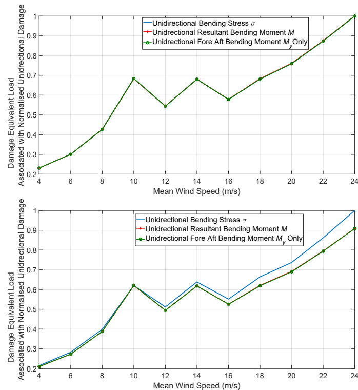
Figure 18. Normalised damage equivalent load associated with uni-directional fatigue damage using 10 min bending stress \sigma , resultant bending moment M and fore-aft bending moment M_y time series where \theta and \tau are fixed at 0^\circ ( above ) and where \theta and \tau are fixed at 60^\circ and 30^\circ , respectively ( below ).
