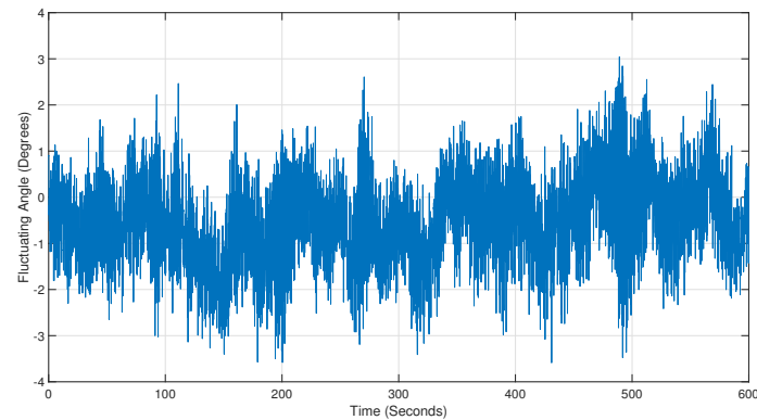
Figure 6. Aeroelastic model results for fluctuating angle between hub thrust and lateral forces for wind speed for a below-rated wind speed of 6 m/s.
