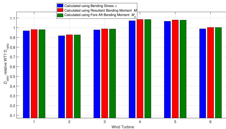
Figure 23. Normalised D_{ratio} calculated using bending stress \sigma , resultant bending moment M and fore-aft bending moment M_y for a range of wind turbines.
