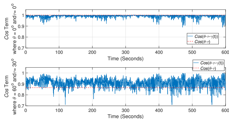
Figure 14. Cos term evaluation for above-rated wind speed (22 m/s) for set with \theta = 0^\circ , \tau = 0^\circ (above) and for set with \theta = 60^\circ , \tau = 30^\circ (below).
