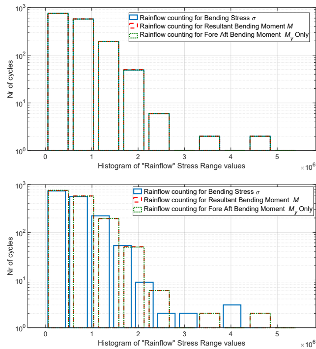
Figure 15. Histograms of 10 min bending stress \sigma , resultant bending moment M , and fore-aft bending moment M_y time series for below-rated mean wind speed (6 m/s), set \theta = 0^\circ , \tau = 0^\circ (above), set \theta = 60^\circ , \tau = 30^\circ (below).
