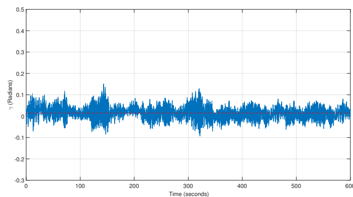
Figure 9. Deviation \gamma for below-rated wind speed (6 m/s).
