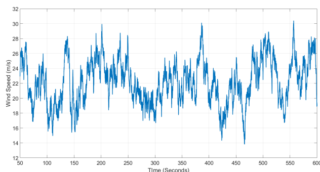
Figure 5. Aeroelastic model results for wind speed for an above-rated wind speed of 22 m/s.
