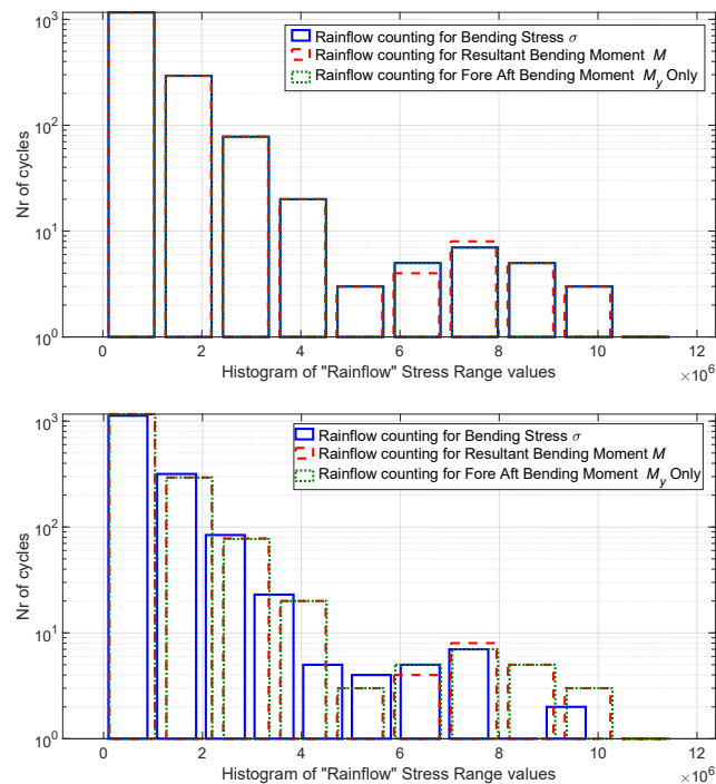
Figure 16. Histograms of 10 min bending stress \sigma , resultant bending moment M , and fore-aft bending moment M_y time series for rated mean wind speed (10 m/s), set \theta = 0^\circ , \tau = 0^\circ (above), set \theta = 60^\circ , \tau = 30^\circ (below).
