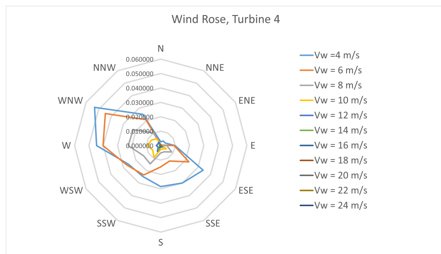
Figure A3. Wind Rose 4—wind speed and wind direction probability for wind turbine 4.
