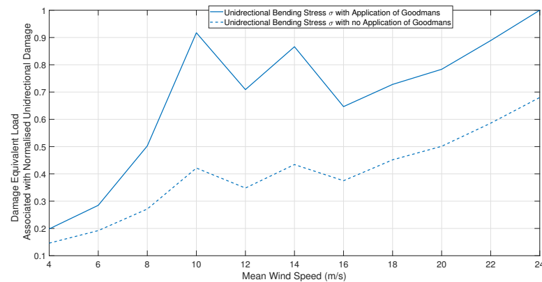
Figure 19. Comparison of normalised damage equivalent load associated with uni-directional fatigue damage using 10 min bending stress \sigma time series with and without Goodman's correction where \theta and \tau are fixed at 0^\circ .
