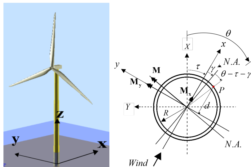
Figure 2. Wind turbine elevation co-ordinate system [18] (left), the tower co-ordinate system and cross section parameters as defined in this study (right).
