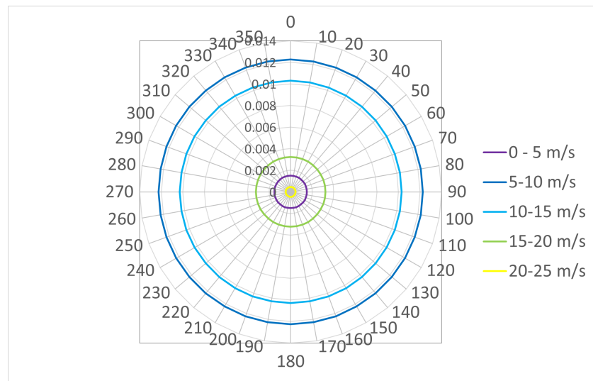
Figure A5. Wind Rose A –An equally distributed wind rose.
