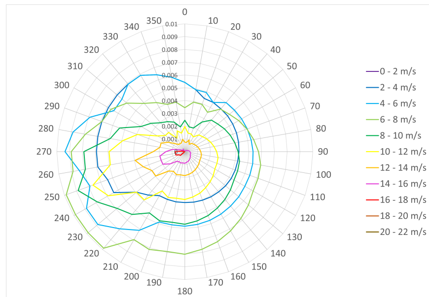
Figure A7. Wind Rose C – with prevailing wind direction.
