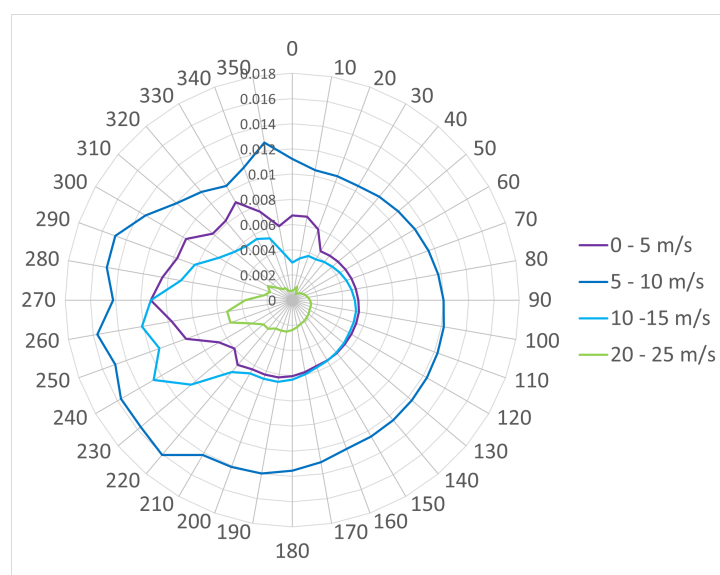
Figure A6. Wind Rose B – with prevailing wind direction.
