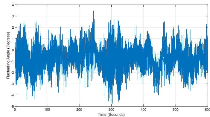
Figure 7. Aeroelastic model results for fluctuating angle between hub thrust and lateral forces for wind speed for a rated wind speed of 10 m/s.
