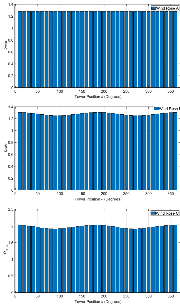
Figure 22. Absolute D_{Ratio} between uni-directional fatigue damage and fatigue damage at a range of tower positions \theta for a range of wind roses.
