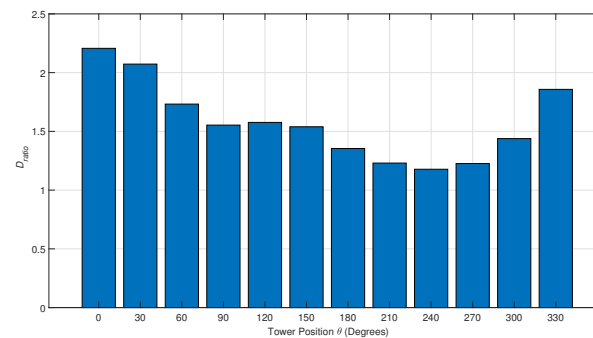
Figure 21. Absolute D_{Ratio} between uni-directional fatigue damage and fatigue damage at a range of tower positions \theta for wind rose 1 with the application of the Goodman's correction factor.
