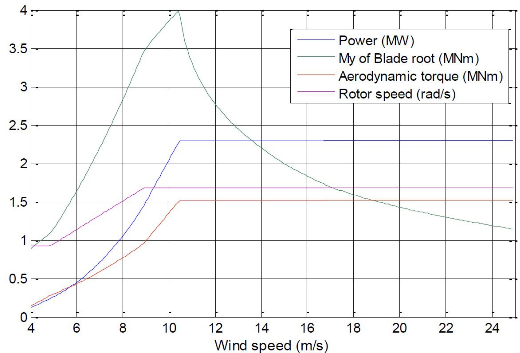
Figure A1. Variation of general parameters of wind turbine's base model as a function of mean wind speed in steady-state conditions [15].
