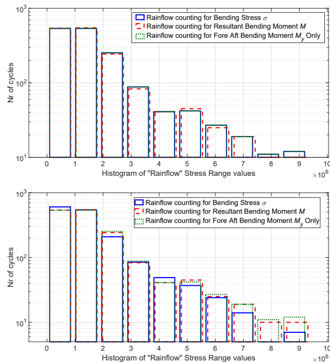
Figure 17. Histograms of 10 min bending stress \sigma , resultant bending moment M , and fore-aft bending moment M_y time series for above-rated mean wind speed (22 m/s) set \theta = 0^\circ , \tau = 0^\circ (above), set \theta = 60^\circ , \tau = 30^\circ (below).
