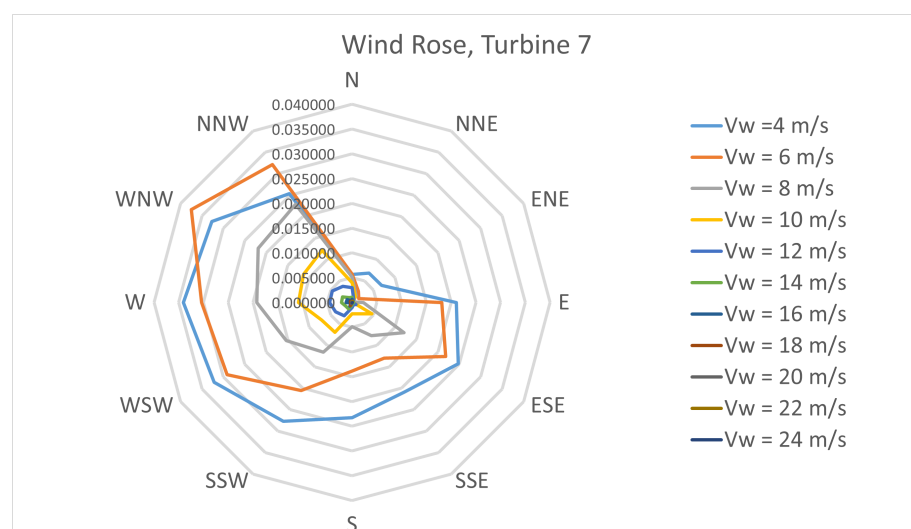
Figure A4. Wind Rose 7—wind speed and wind direction probability for wind turbine 7.
