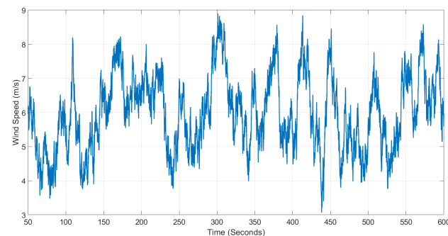
Figure 3. Aeroelastic model results for wind speed for a below-rated wind speed of 6 m/s.
