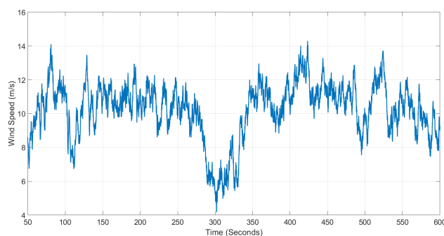
Figure 4. Aeroelastic model results for wind speed for a rated wind speed of 10 m/s.
