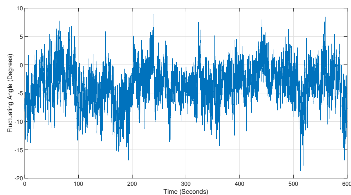
Figure 8. Aeroelastic model results for fluctuating angle between hub thrust and lateral forces for an above-rated wind speed of 22 m/s.
