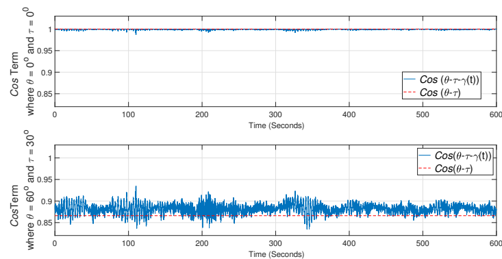
Figure 13. Cos term evaluation for rated wind speed (10 m/s) for set \theta = 0^\circ , \tau = 0^\circ (above) and for set \theta = 60^\circ , \tau = 30^\circ (below).
