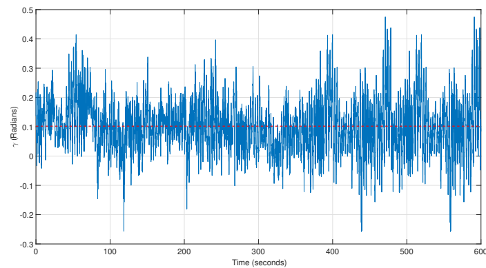
Figure 11. Deviation \gamma for above-rated wind speed (22 m/s).
