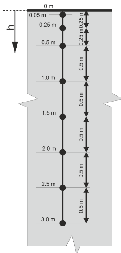
Figure 3. Diagram of the test stand for measuring the temperature distribution in the soil.
