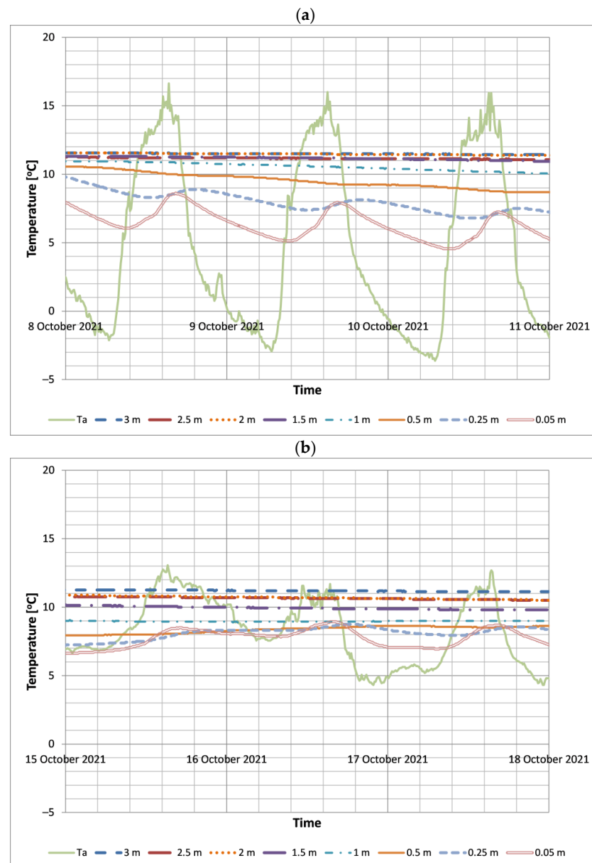
Figure 7. The daily evolution of the temperatures in the ground of point No. 2 for the diurnal temperature ranges: (a) \Delta T_a = 20\text{ }^{\circ}\text{C} , (b) \Delta T_a = 8\text{ }^{\circ}\text{C} .
