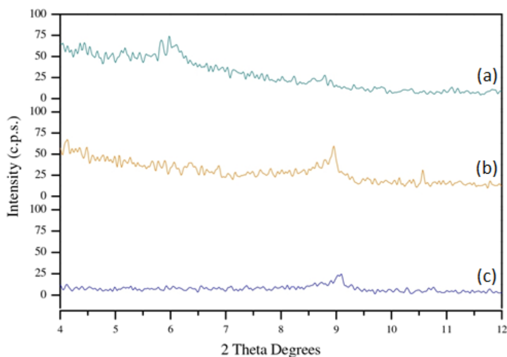
Figure 5. Mineralogical identification: (a) sample from measurement point 1; (b) sample saturated in \text{K}^+ ; (c) sample saturated in \text{K}^+ and subsequently calcined at 550^\circ\text{C} .
