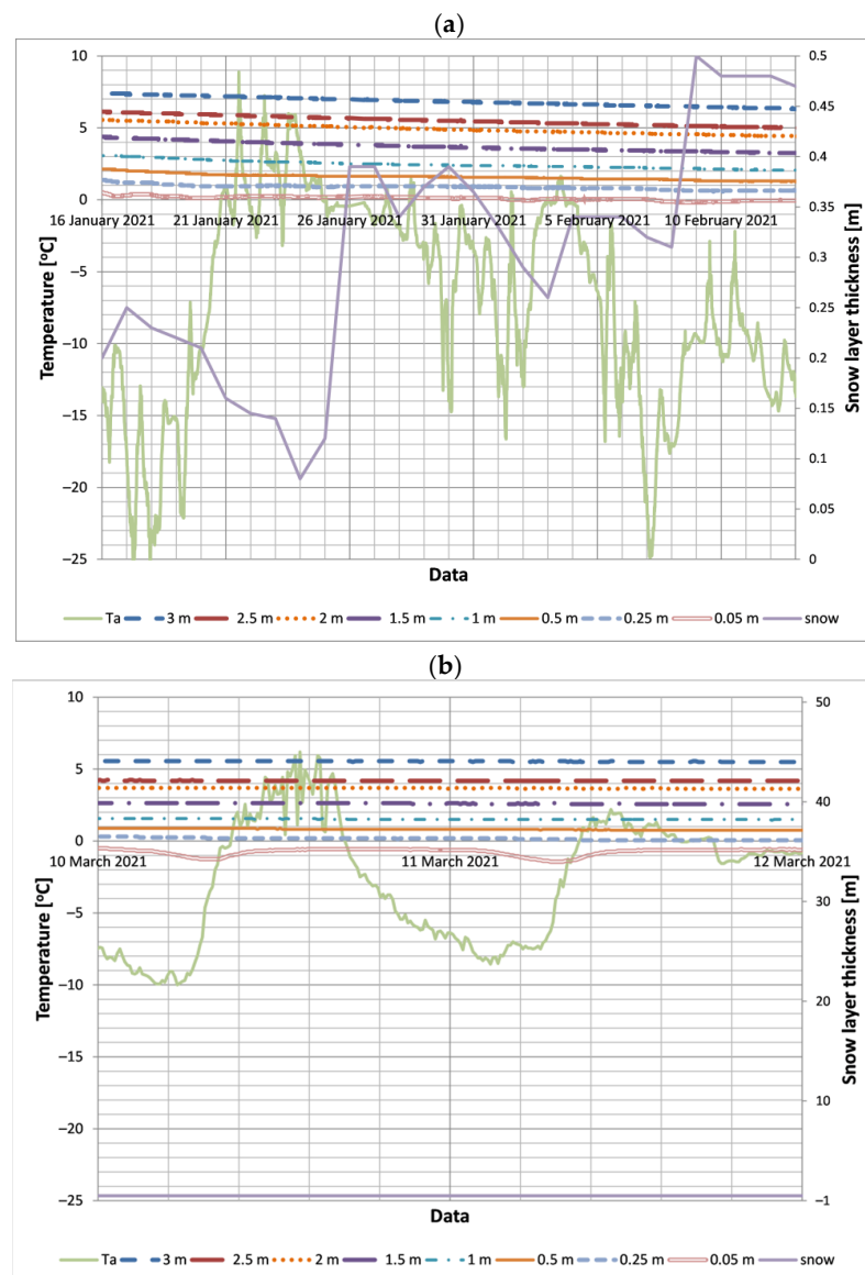
Figure 10. Temperature changes in the ground of point No. 2 in the snowy (a) and snowless (b) winter period.
