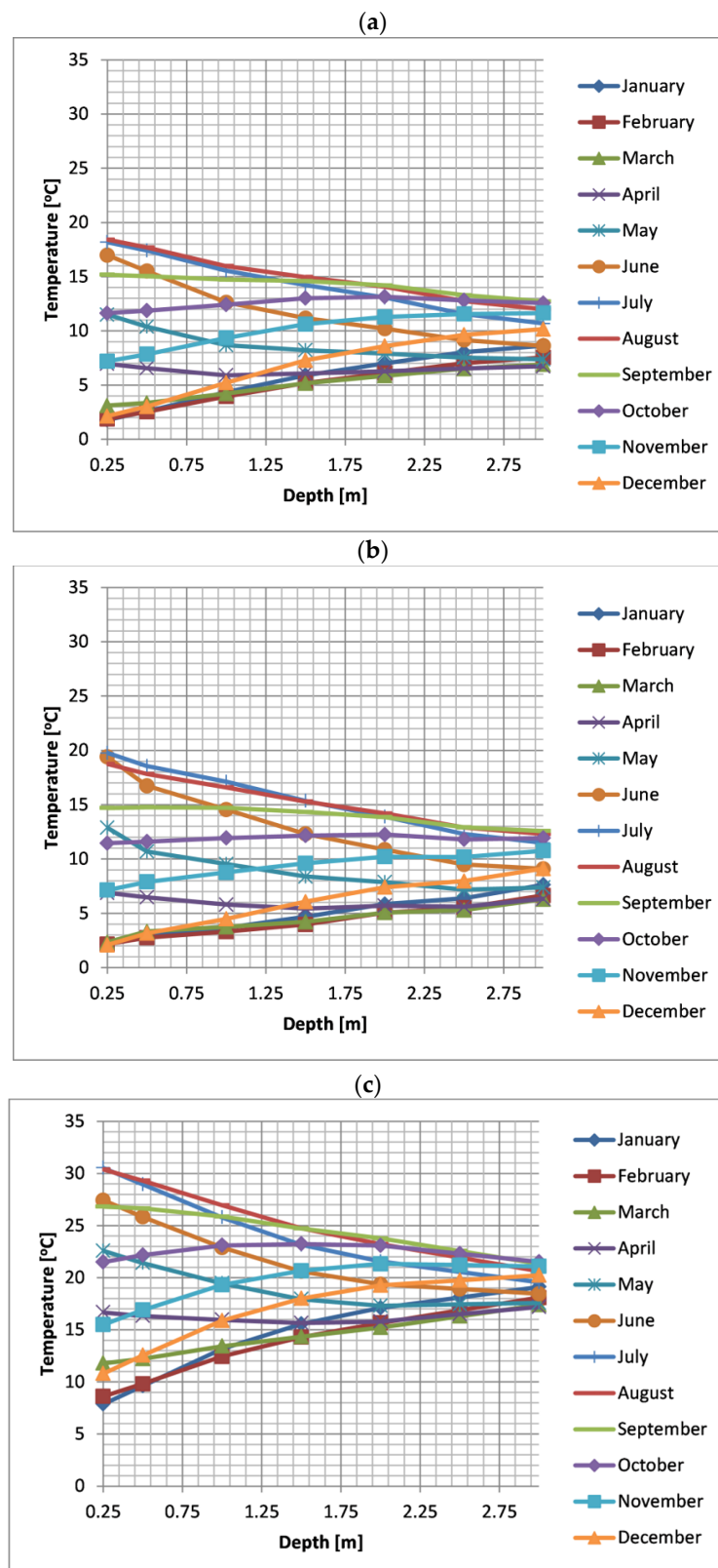
Figure 8. Average monthly temperatures as a function of depth for three measurement points: (a) No. 1, (b) No. 2, (c) No. 3.
