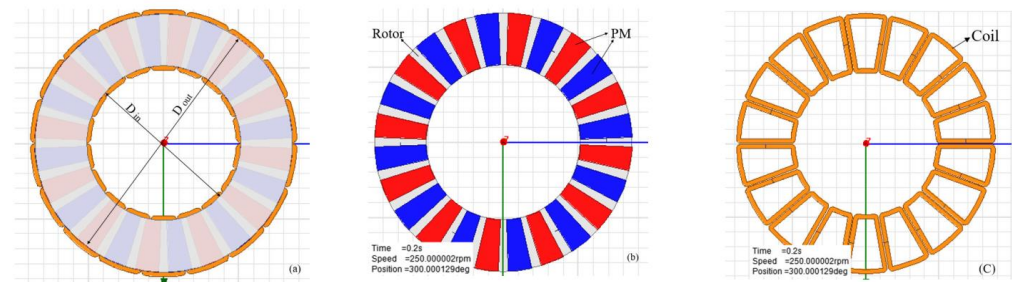
Figure 2. Structure of ironless AFPMSC: (a) general structure, (b) Rotor and PMs structure, and (c) ironless stator.
