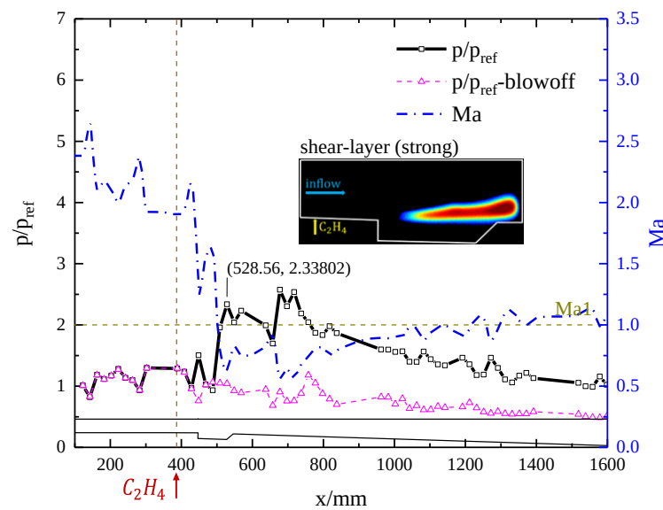
Figure 7. Dimensionless pressure/Mach number along x axis and mean pseudo-color image of \text{CH}^* chemiluminescence at Case 11 ( 1.7D_0\text{I}0.144 ).
