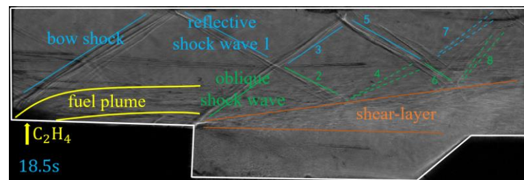
Figure 8. Shadowgraph at Case 11 ( 1.7D_0\text{I}0.144 ). 1—Reflected shock wave, 2—Intersecting shock waves, 3—Intersecting shock waves, 4—Reflected expansion wave, 5—Reflected shock wave, 6—Intersecting shock waves, 7—Intersecting expansion wave, 8—Reflected shock wave.
