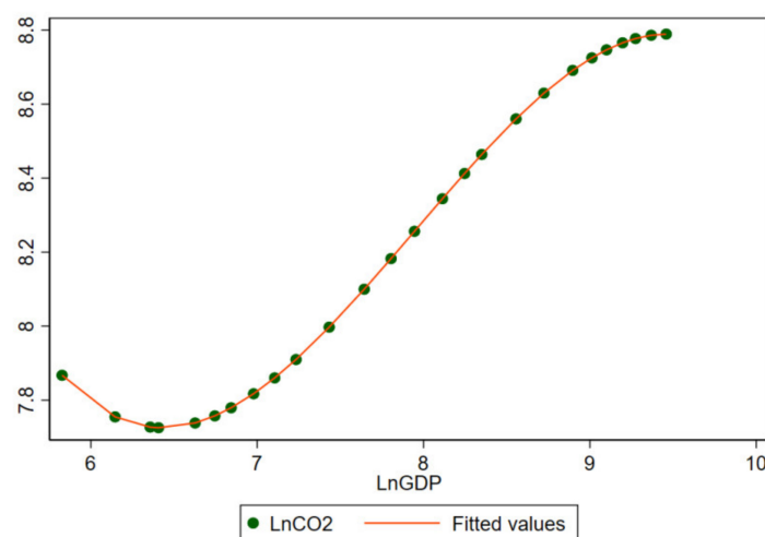
Figure 9. Equation (7).
