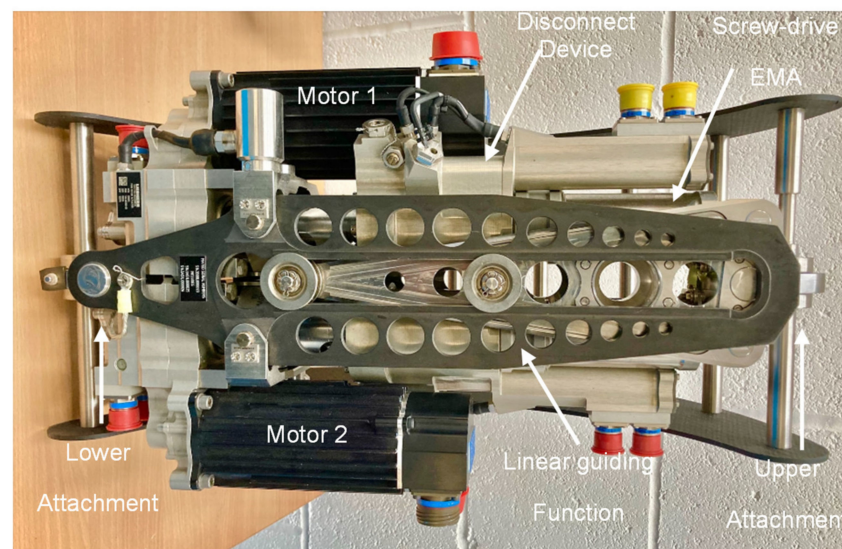
Figure 1. Helicopter electromechanical actuation system.
