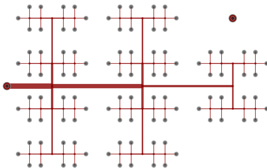
Figure 5. The spanning-tree network structure of the generic constructed district heating system: The various thicknesses of the edges symbolise the diameter of the installed pipes. Grey nodes represent the connected buildings and larger grey nodes with a red ring symbolise the heat sources.
