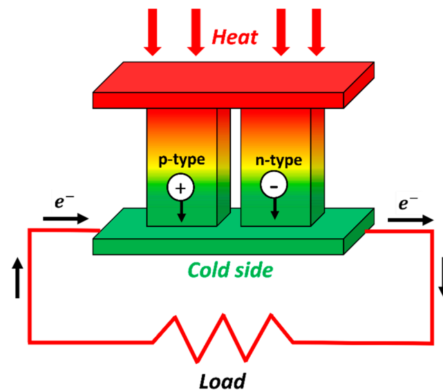
Figure 4. Physical principle of thermoelectric generator [35].
