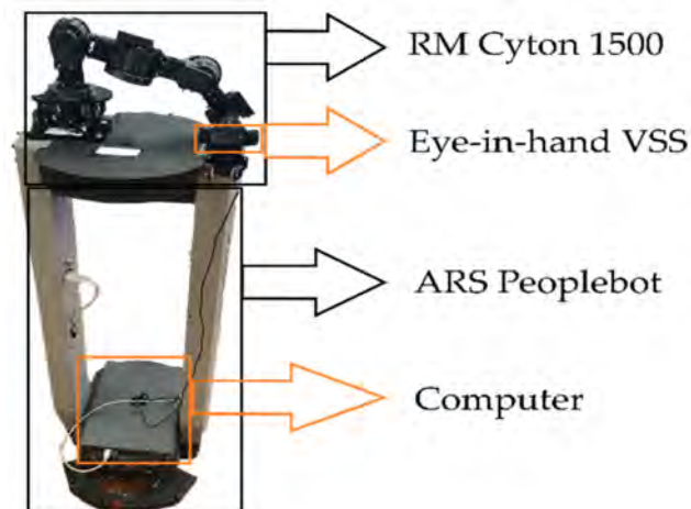
Figure 5. The CAS composed of ARS, RM, eye-in-hand VSS, and a computer.
