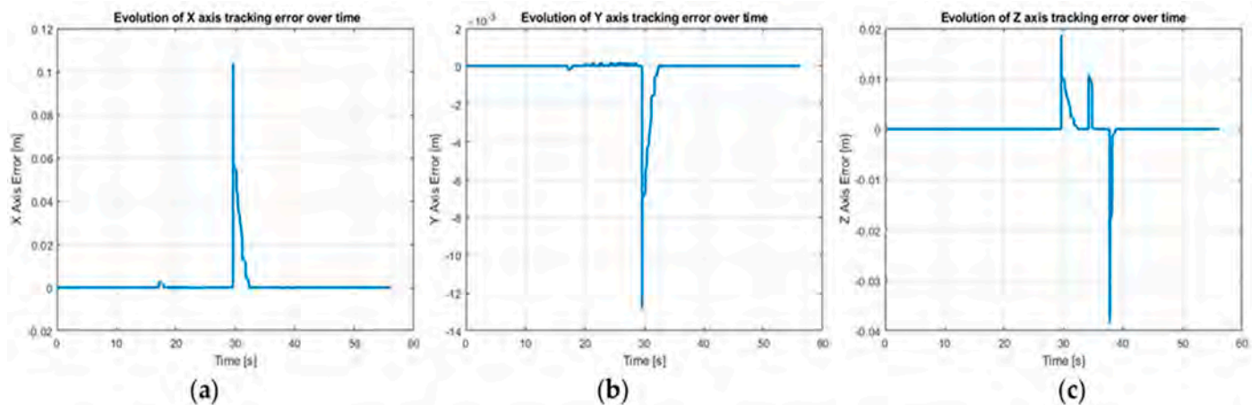
Figure 26. Tracking errors for RM Cyton picking object trajectory on: (a) X axis, (b) Y axis, (c) Z axis.
