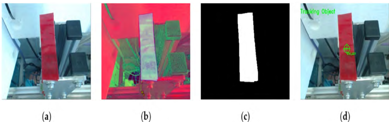
Figure 22. Warehouse reference color detection: (a) raw RGB image, (b) BGR to HSV conversion, (c) HSV limits are imposed and the result is shown as a white blob with a black background, (d) the reference color is detected, and the centroid is tracked.
