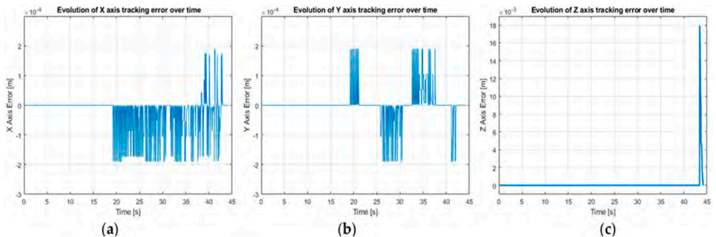
Figure 28. Tracking errors for RM Cyton placing object trajectory on: (a) X axis, (b) Y axis, and (c) Z axis.
