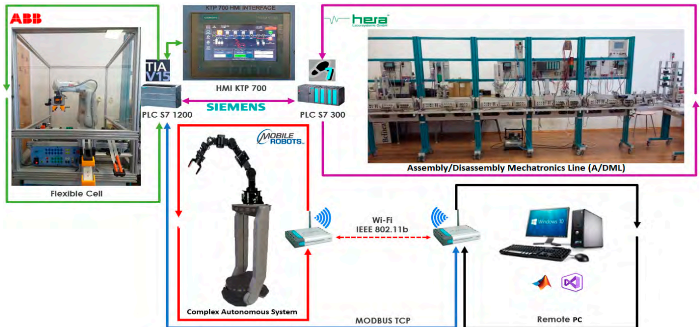
Figure 1. Control structure of A/DML Hera&Horstmann, FC with ABB IRM and CAS with PeopleBot WMR and Cyton 1500 RM.
