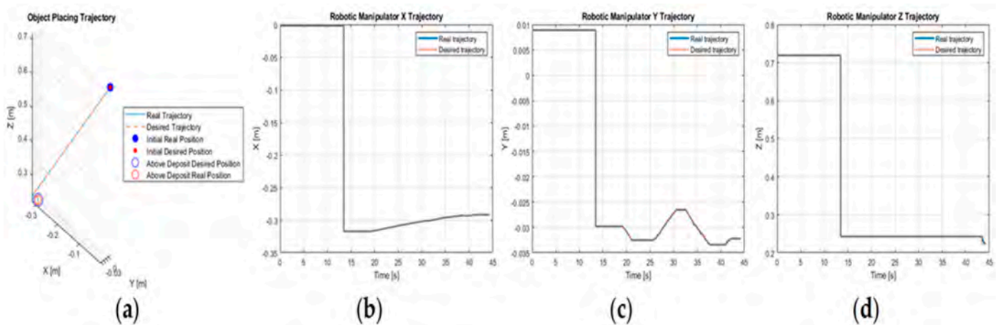
Figure 27. Desired and real object placing trajectories of the RM Cyton based on inverse kinematics control and eye-in-hand VSS for positioning at the warehouse: (a) signifies the complete trajectory, while (b–d) are the trajectories separated on the X, Y, and Z axes, respectively.
