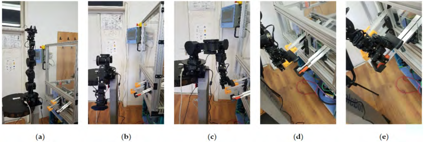
Figure 18. Real-time control of the 7-DOF Cyton 1500 RM located at the FC with the following sequences: (a) home position, (b) intermediary position, (c,d) scanning position, (e) picking object.
