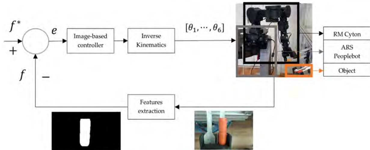
Figure 13. Closed-loop control of the RM Cyton based on eye-in-hand type VSS.
