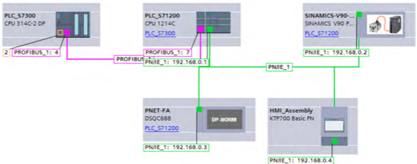
Figure 2. Flexible Cell Siemens S7-1200 PLC hardware structure.
