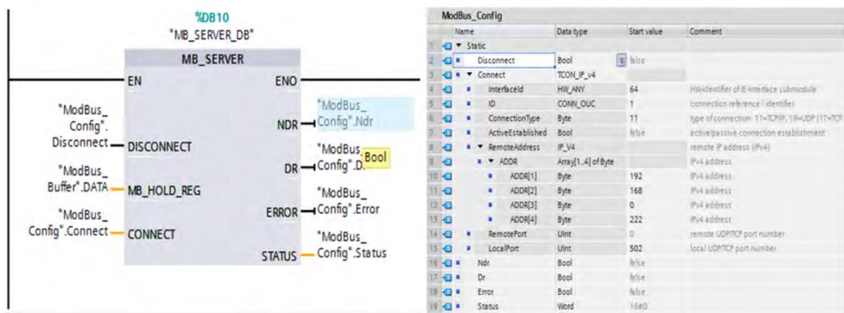
Figure 16. Siemens Modbus Server configuration in main routine.
