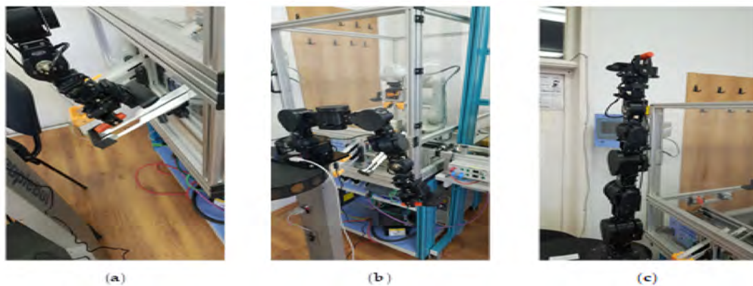
Figure 19. Real-time control of the RM Cyton 7-DOF located at the FC with the following sequences: (a) lifting object, (b) moving to the intermediate position, (c) parking position with the piece in the gripper.
