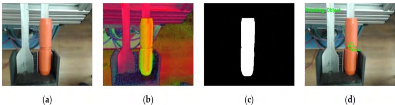
Figure 20. Object Detection with the following steps: (a) raw RGB image taken from the camera, (b) conversion from BGR to HSV (c) image segmentation after HSV limits are set, with morphological operations of erosion and dilation, (d) object is detected and the centroid is being tracked.
