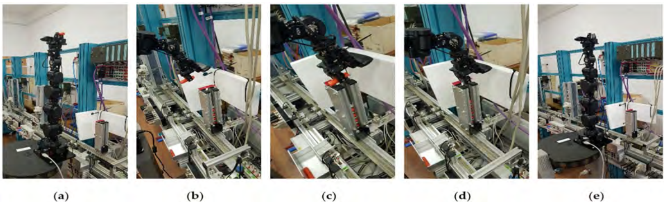
Figure 21. Real-time control of the RM Cyton located at the cylinders warehouse which has the resulting actions: (a) parking position with the object in the gripper, (b) scanning position, (c) moving above the warehouse, (d) placing the piece in the depot, (e) returning to home position.
