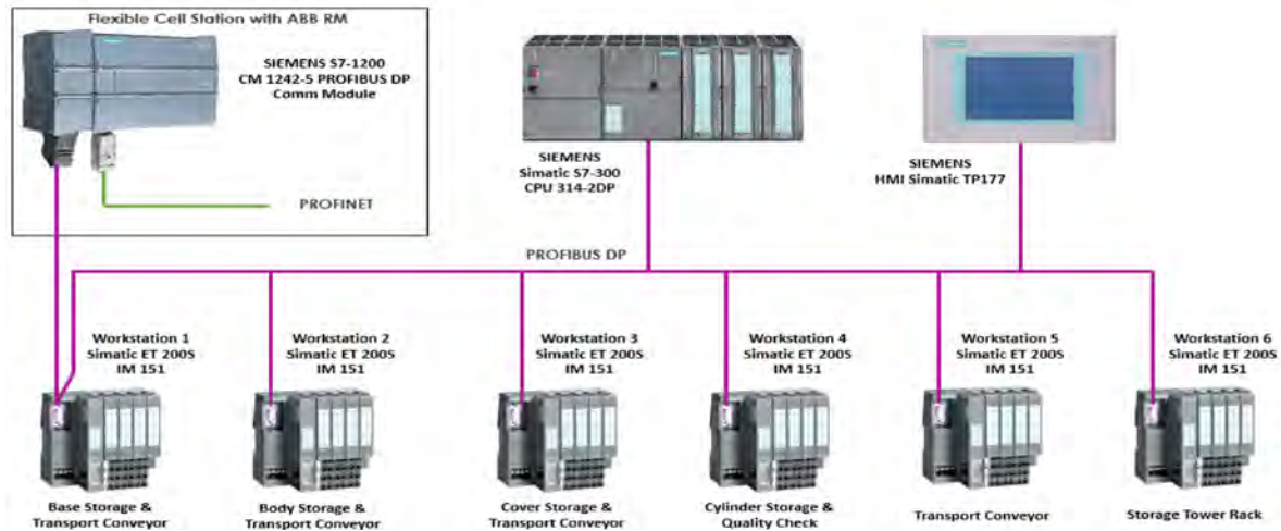
Figure 12. PLC hardware structure of the Mechatronics line Hera&Horstmann.
