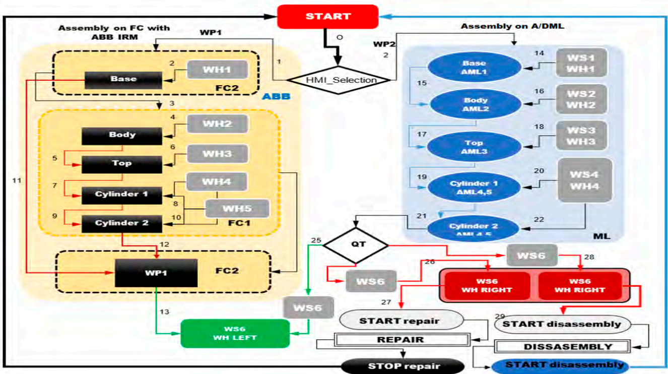
Figure 9. Task scheduling for assembly functionality.
