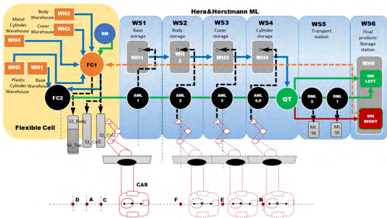
Figure 8. A/D/RML assisted by CAS.
