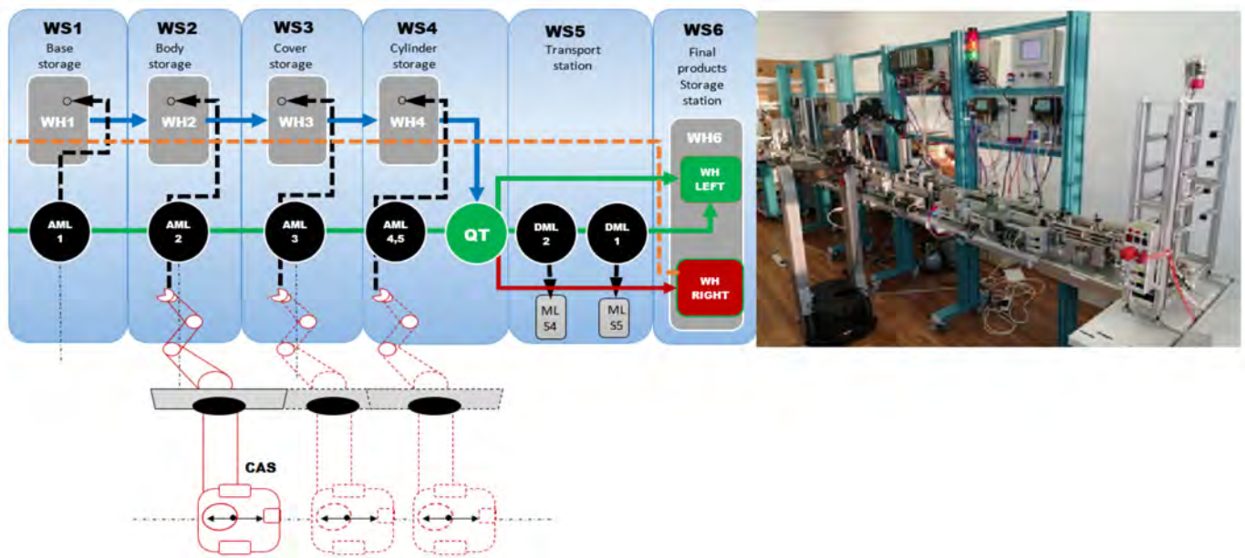
Figure 4. A/D/M L Hera&Horstmann ML with symmetrical final product storage.
