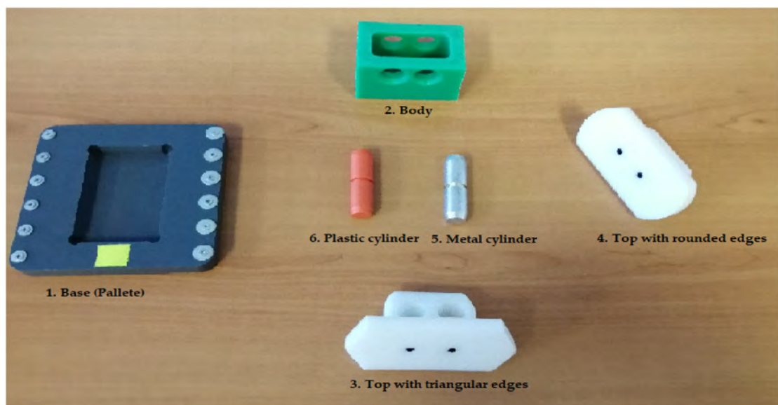
Figure 6. Workpiece parts.
