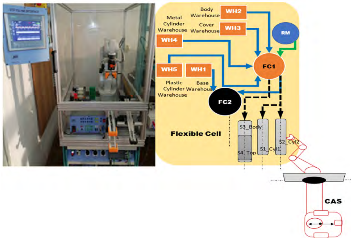
Figure 3. Flexible Cell Station with 6-DOF ABB IRB120.
