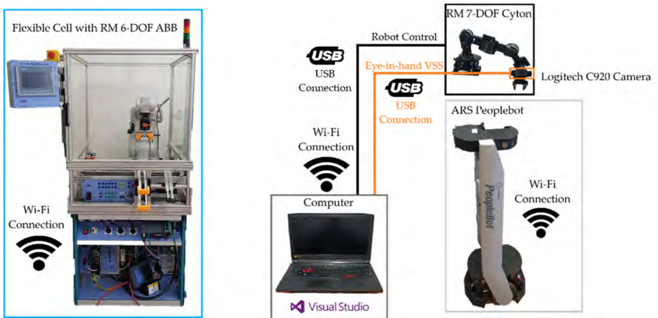
Figure 14. Communication block set of the computer between the FC, ARS PeopleBot WMR equipped with the Cyton RM and eye-in-hand VSS.
