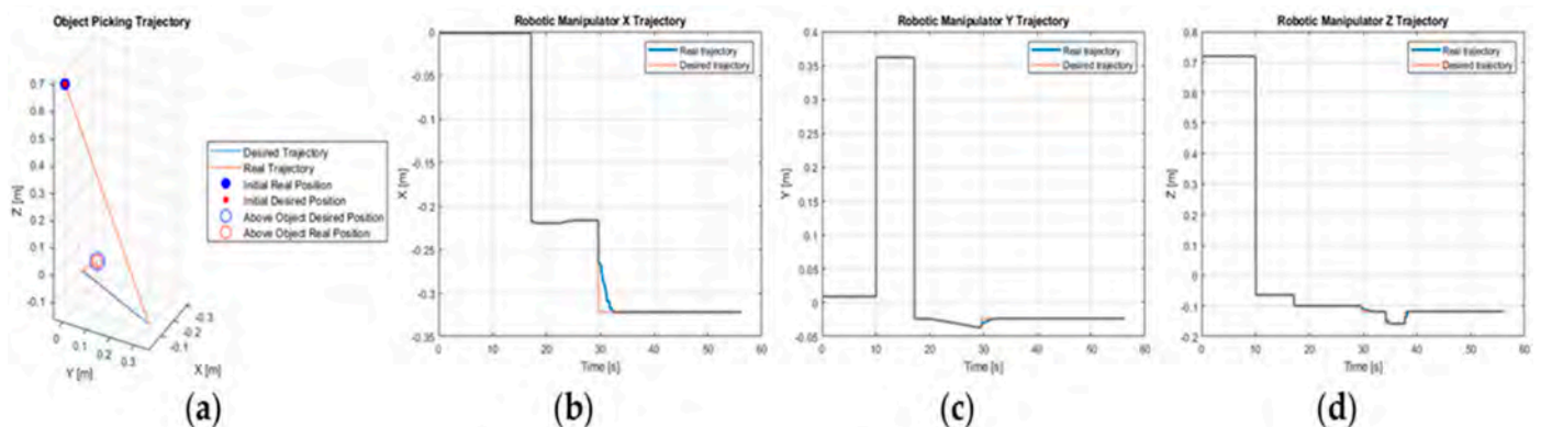
Figure 25. Desired and real object picking trajectories of the RM Cyton based on inverse kinematics control and eye-in-hand VSS for accurate positioning at the FC: (a) the complete trajectory, from the home position to above object position, (b) X axis, (c) Y axis, (d) Z axis trajectories.
