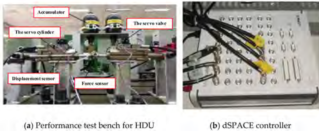
Figure 12. Photos of the experimental platform.
