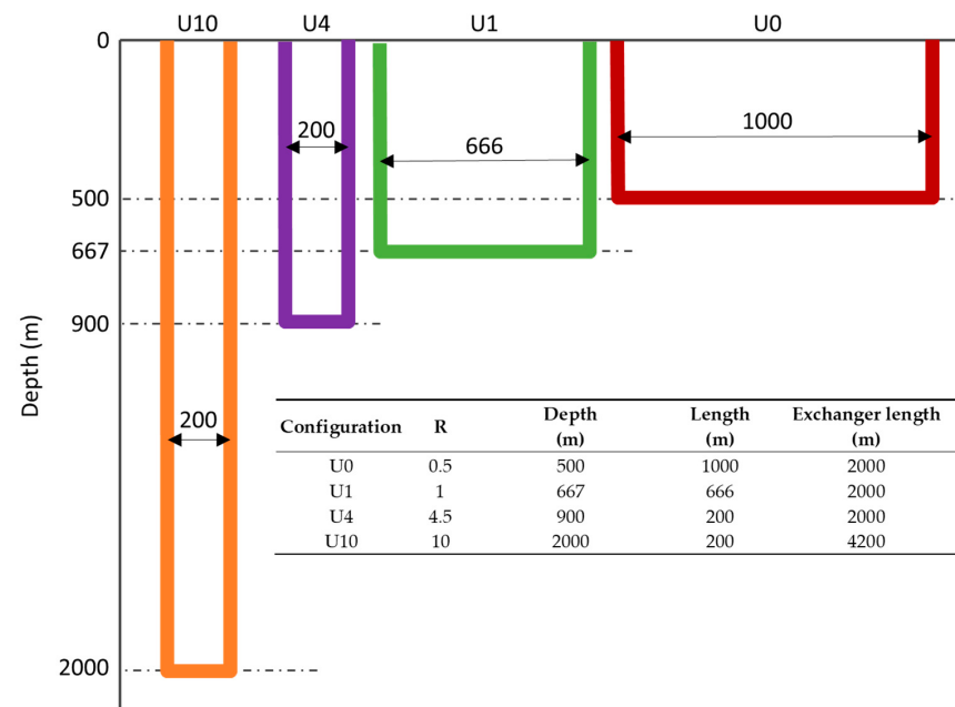
Figure 4. ULHE geometry configurations.
