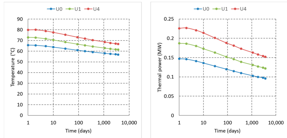
Figure 10. ULHE performances as a function of the ratio R ( Q = 0.5 \text{ m}^3/\text{h} ).
