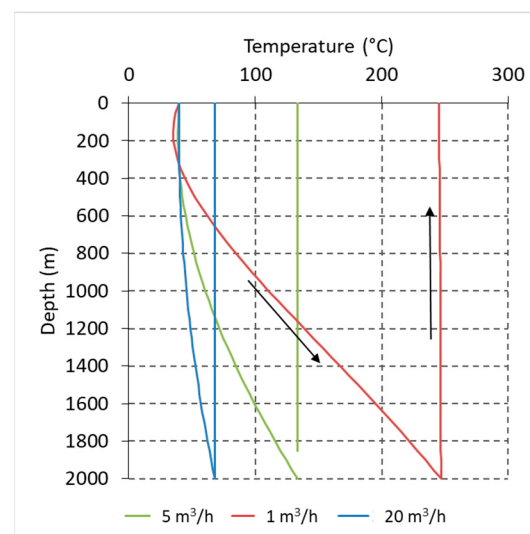
Figure 6. Temperature profiles for different flow rates in the DBHE (after one year from startup).
