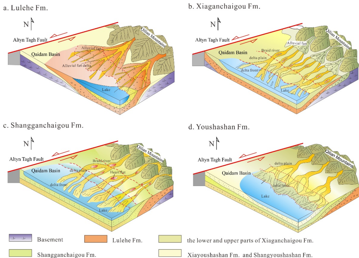
Figure 13. Cenozoic sedimentary environment evolution of the study area.
