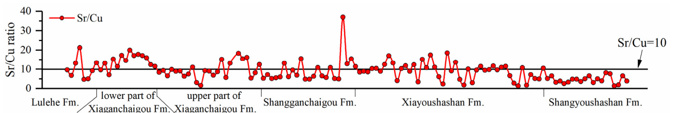
Figure 8. Sr/Cu climate discrimination diagram of lutite samples in the study area.
