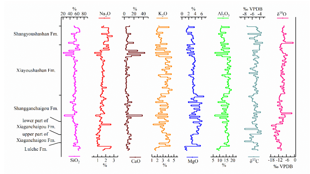
Figure 5. Variation trend of major elements and carbon and oxygen isotopes of the lutite samples in the study area.
