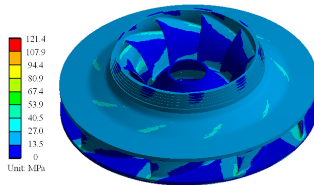
Figure 10. Von-Mises stress on the runner in rated operating condition.
