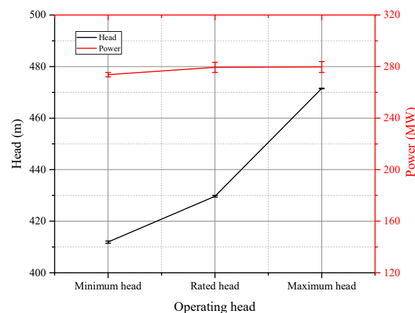
Figure 4. Validation of the numerical simulation.
