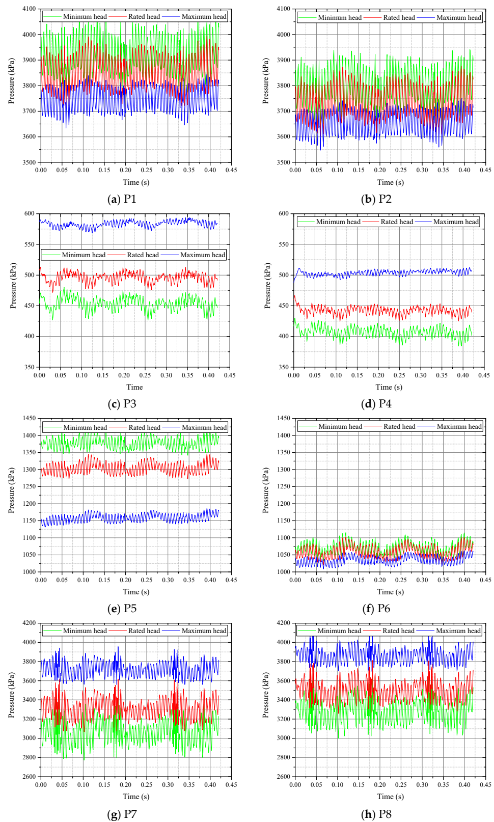
Figure 7. Pressure pulsation at monitoring points at three analyzed operating heads.
