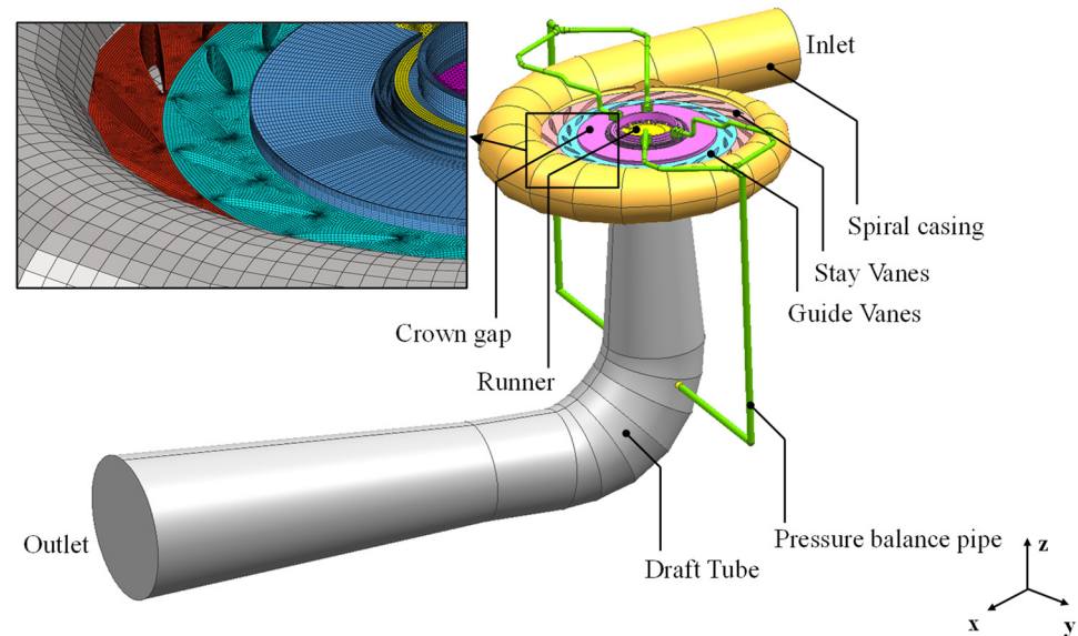
Figure 1. CFD domain and mesh of pump–turbine.
