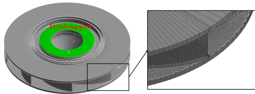
Figure 3. FEM model and boundary condition of runner.
