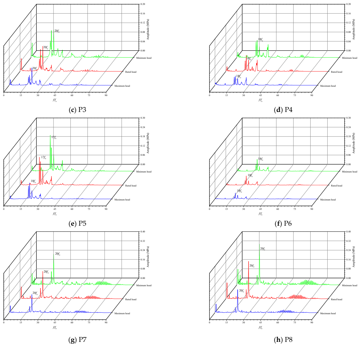
Figure 12. Frequency spectra of the dynamic stress at monitoring points.
