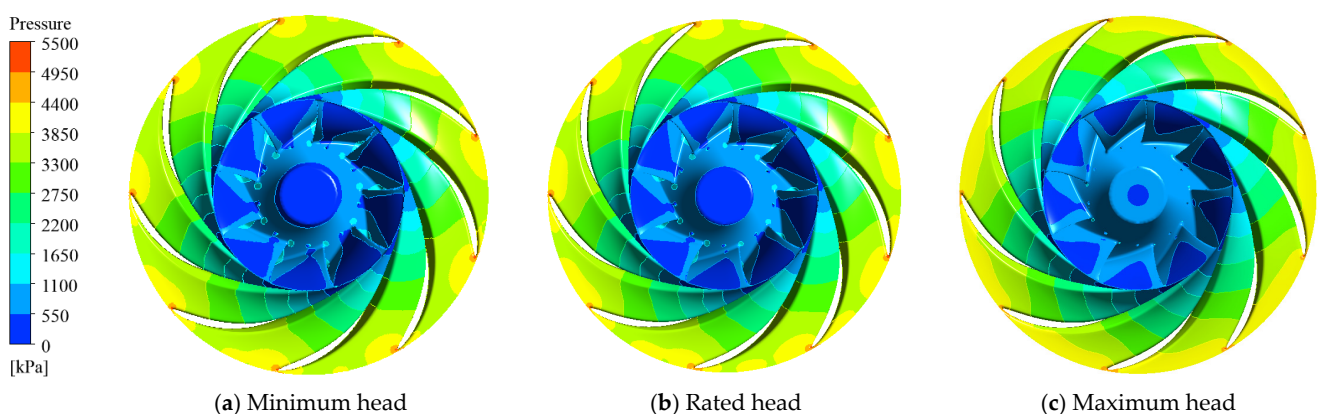
Figure 6. The pressure distribution on the runner's inner surface in three operating heads.
