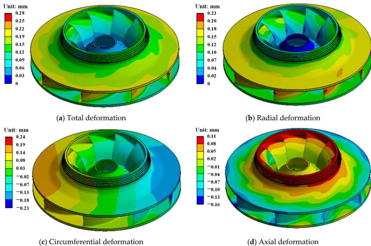
Figure 9. Total and directional deformations of the runner in rated operating condition.
