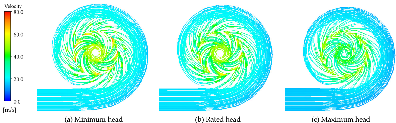
Figure 5. The streamline in the flow passage in three operating heads.
