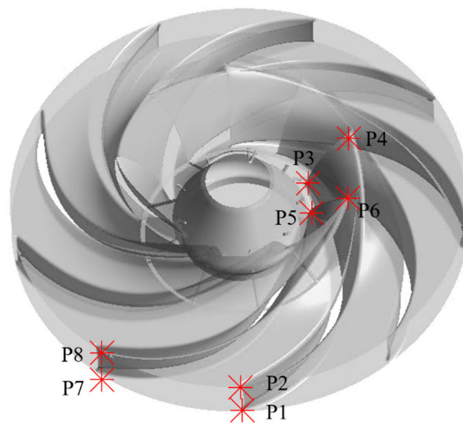
Figure 2. Pressure pulsation monitoring points and dynamic stress monitoring points.
