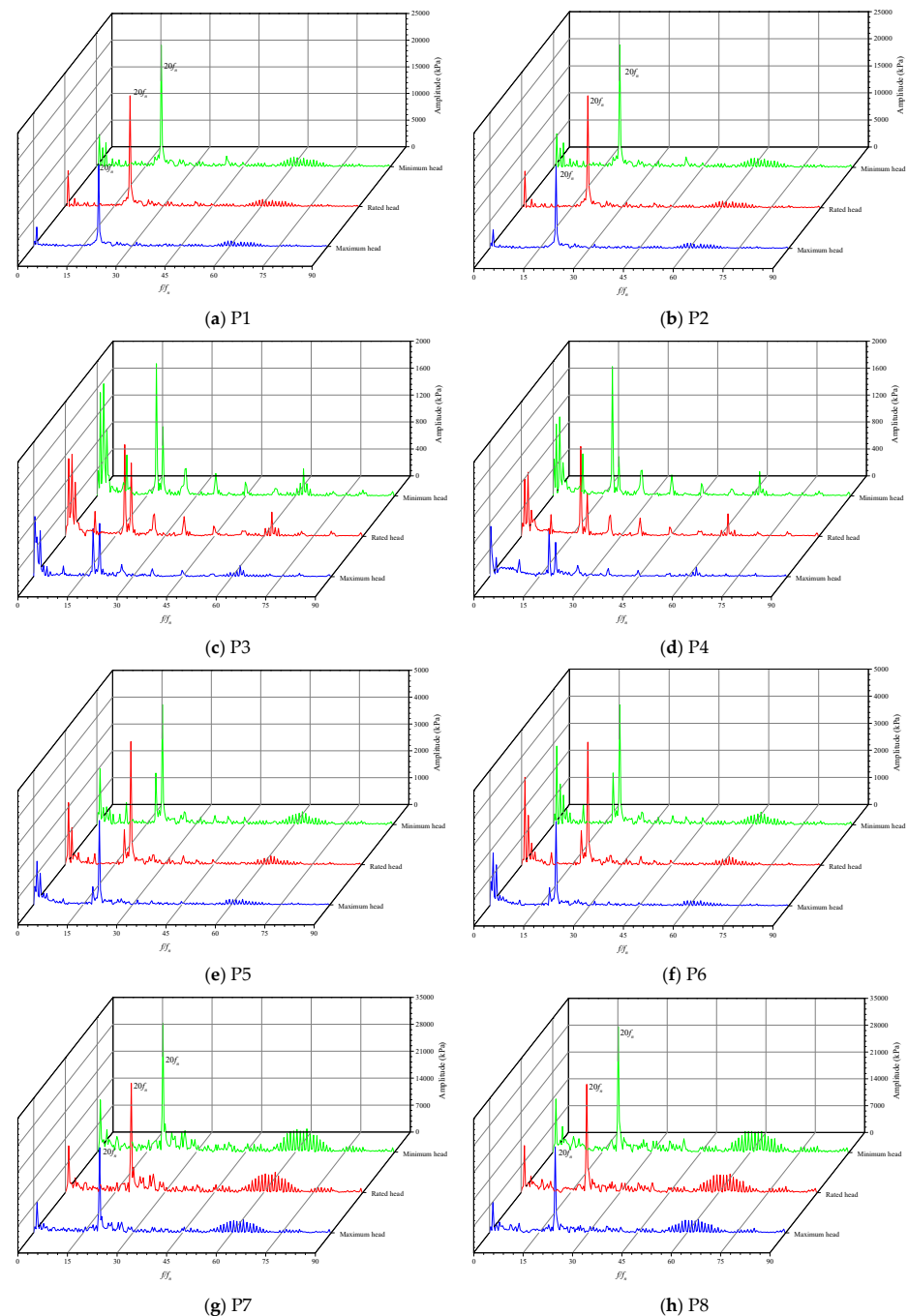
Figure 8. Frequency spectra of the pressure pulsation at monitoring points.
