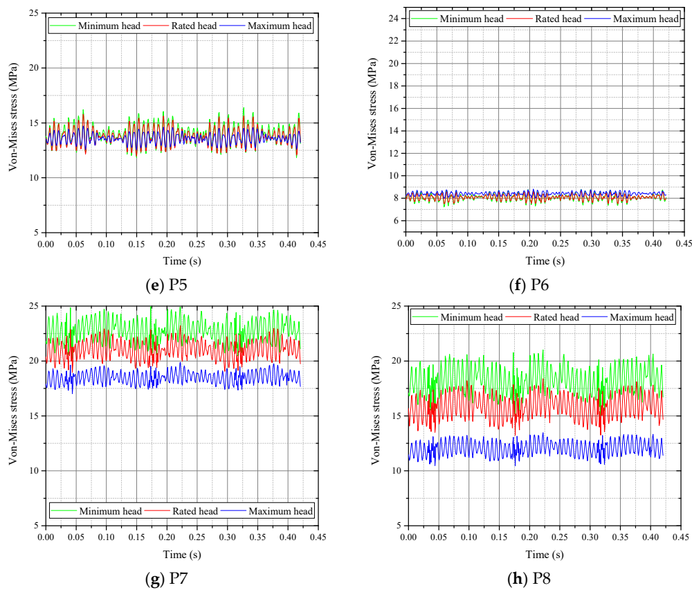
Figure 11. Dynamic stresses at monitoring points.
