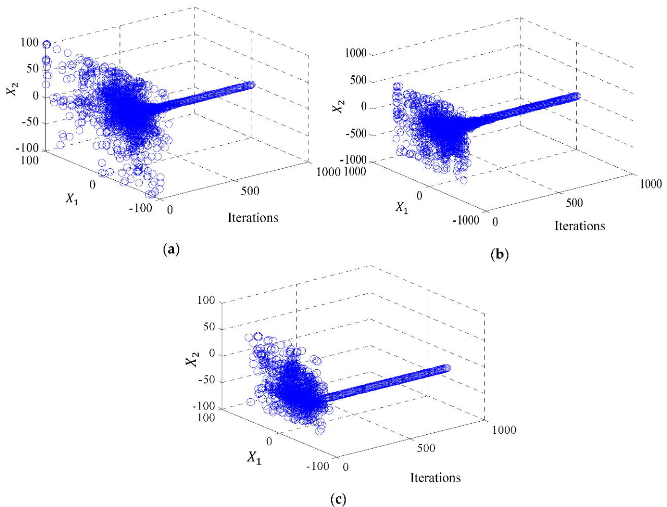
Figure 7. Evaluation of different types of benchmark functions; (a): F_1 , (b): F_{11} , (c): F_{14} .
