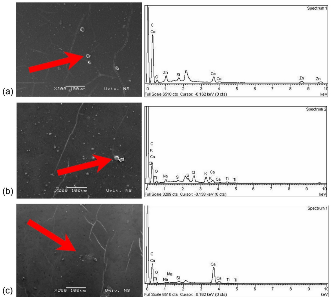
Figure 3. Position on the micrograph (red arrow) and EDS spectra on the samples: (a) 1% ZnO nanoclusters, (b) 1% TiO 2 nanoclusters, (c) 1% TiO 2 /SiO 2 nanoclusters.
