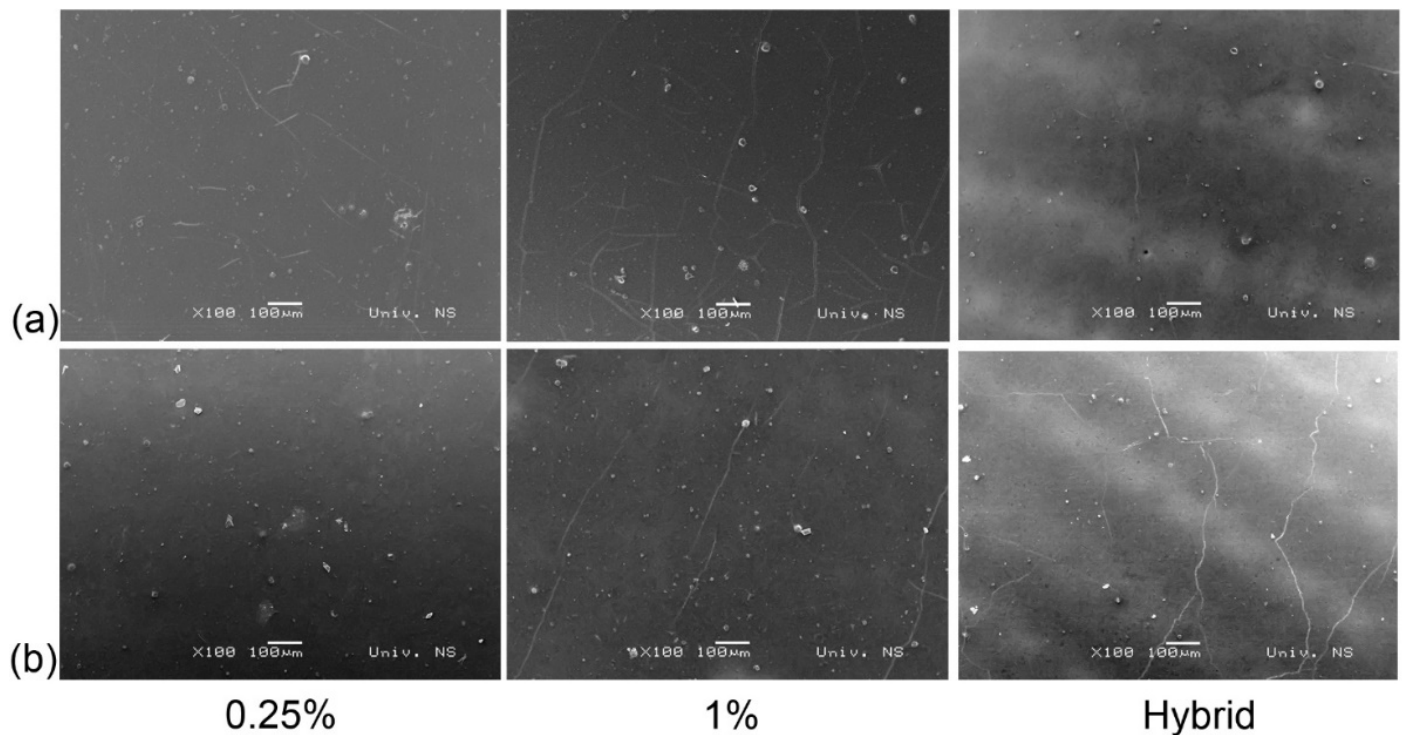
Figure 2. SEM micrographs of samples coated by nanocomposite containing (a) ZnO and (b) TiO 2 .
