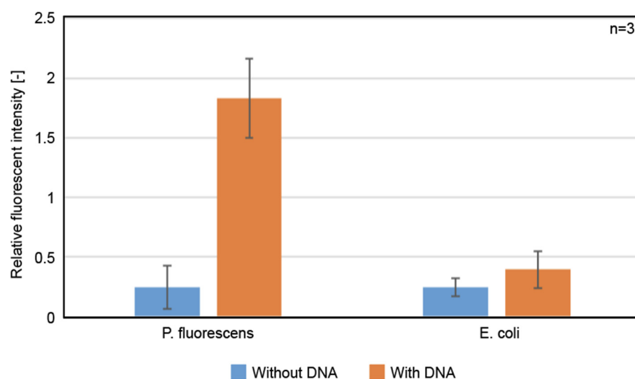
Figure 6. Relative fluorescent intensity of the LBACs encapsulating the CFPES derived from P. fluorescens and E. coli . With DNA: DNA encoding \beta -galactosidase was encapsulated. Without DNA: No DNA was encapsulated. Error bars represent standard deviations ( n = 3 ).
