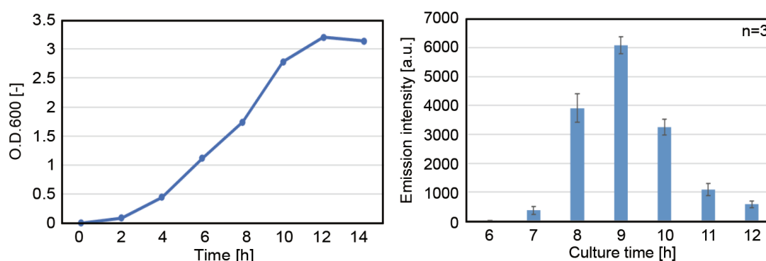
Figure 1. (a) The growth curve of P. fluorescens in 2× YT medium at 23 °C. (b) Comparison of protein expression activity of the CFPES obtained from the cells harvested after varying periods of culture time. The cell-free protein expression system (CFPES) was incubated at 29 °C for 2 h with 51.8 ng/μL of DNA encoding Luciferase under T7 promoter. Premix contained K: 160 mM, Mg: 15 mM, polyethylene glycol (PEG): 1 %. Error bars represent standard deviations ( n = 3 ).
