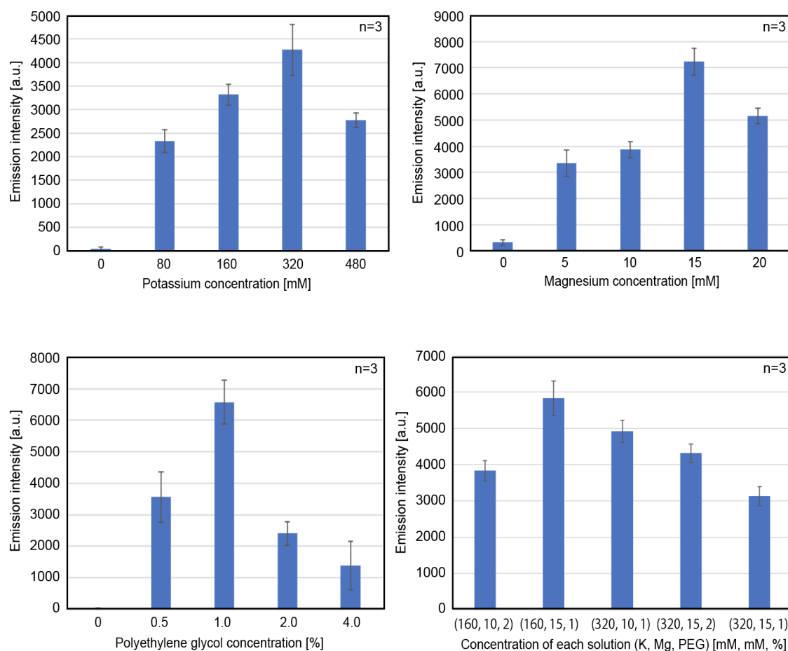
Figure 3. Luciferase assay of the CFPES obtained from Premixes containing different concentrations of potassium, magnesium, and PEG. (a) Premixes with different potassium concentrations. (Mg: 10 mM, PEG: 2 %) (b) Premixes with different magnesium concentrations. (K: 160 mM, PEG: 2 %) (c) Premixes with different PEG concentrations. (K: 160 mM, Mg: 10 mM) (d) Premixes with different concentrations of potassium, magnesium, and PEG. The leftmost bar (K: 160 mM, Mg: 10 mM, PEG: 2 %) represents the data with the Premix condition used in the previous study [11]. The CFPES was incubated at 29 °C for 2 h with 51.8 ng/ \mu L of DNA encoding Luciferase under T7 promoter. Error bars represent standard deviations ( n = 3 ).
