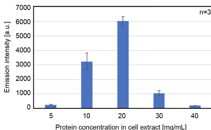
Figure 2. Protein expression activity of the CFPES obtained from the cell extract having various total protein concentrations. The CFPES was incubated at 29 °C for 2 h with 51.8 ng/μL of DNA encoding Luciferase under T7 promoter. Premix contained K: 160 mM, Mg: 15 mM, PEG: 1 %. Error bars represent standard deviations ( n = 3 ).
