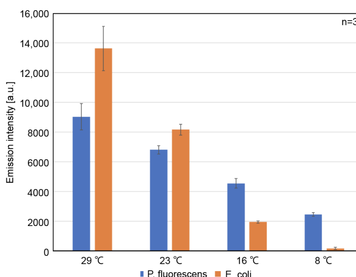
Figure 4. Luciferase assay of the CFPES obtained from the cell extract of P. fluorescens or E. coli at 29 °C, 23 °C, 16 °C, and 8 °C. The CFPES was incubated at each temperature for 2 h with 51.8 ng/μL of DNA encoding Luciferase under T7 promoter. Error bars represent standard deviations ( n = 3 ).
