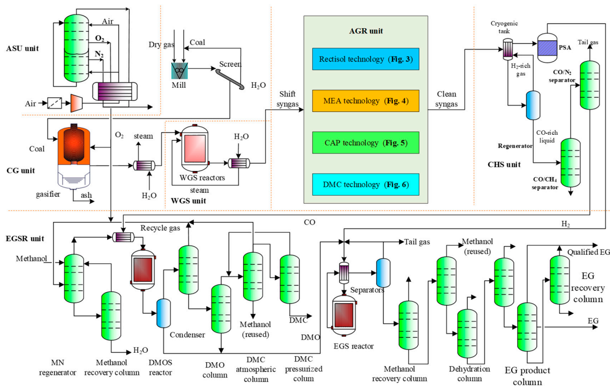
Figure 7. Simplified simulation flowsheet of CTEG process with different CO 2 capture technologies.
