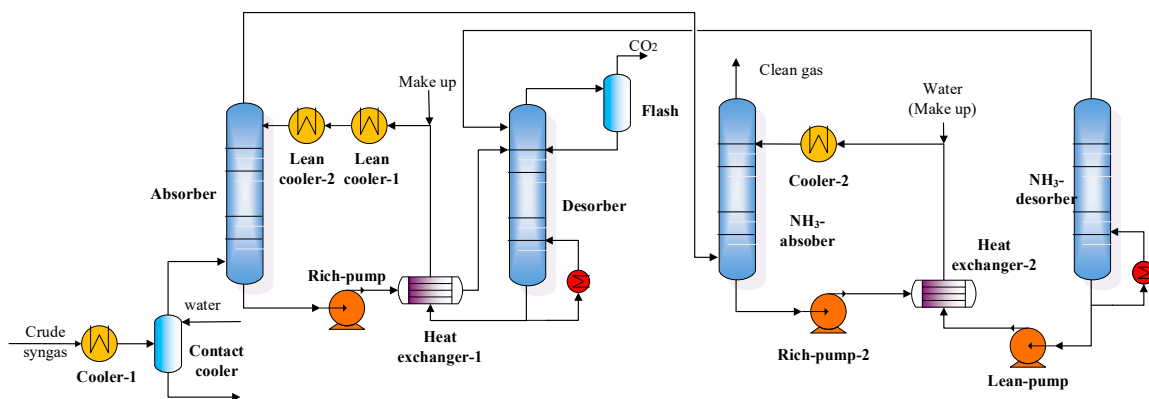
Figure 5. Simplified simulation flowsheet of the CAP technology.
