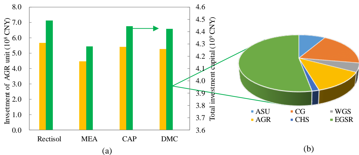
Figure 9. Total capital investment of CTEG process with different CO 2 capture technologies.
