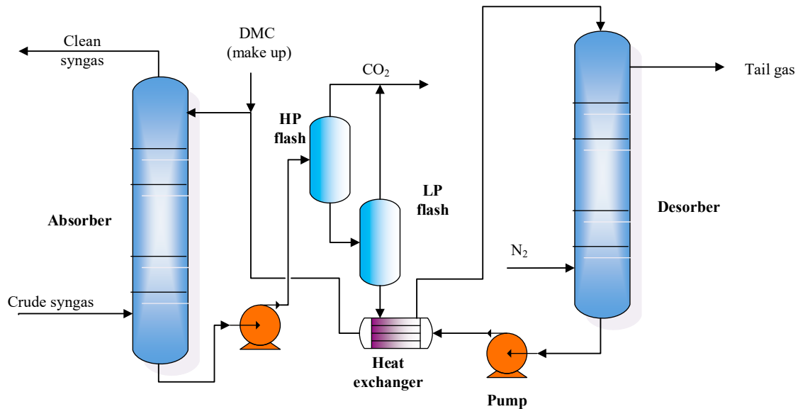
Figure 6. Simplified simulation flowsheet of the DMC technology.
