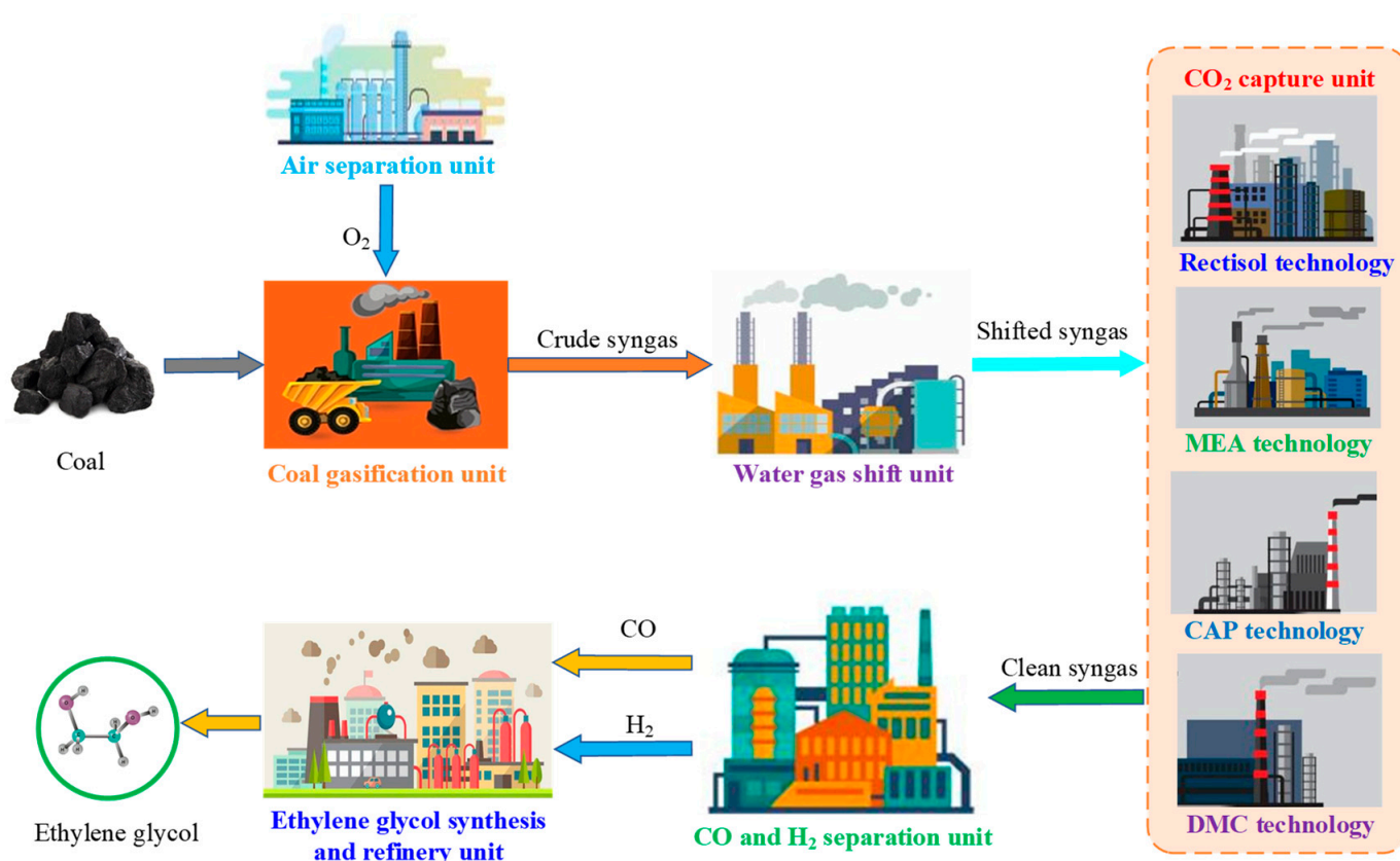
Figure 2. Schematic diagram of the CTEG process with different CO 2 capture technologies.
