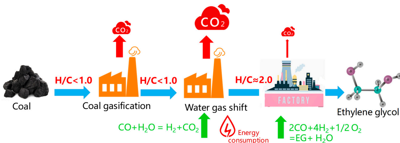
Figure 1. Schematic diagram of the high CO 2 emission reasons for coal to ethylene glycol (CTEG) process.
