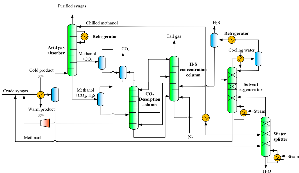
Figure 3. Simplified simulation flowsheet of the Rectisol technology.
