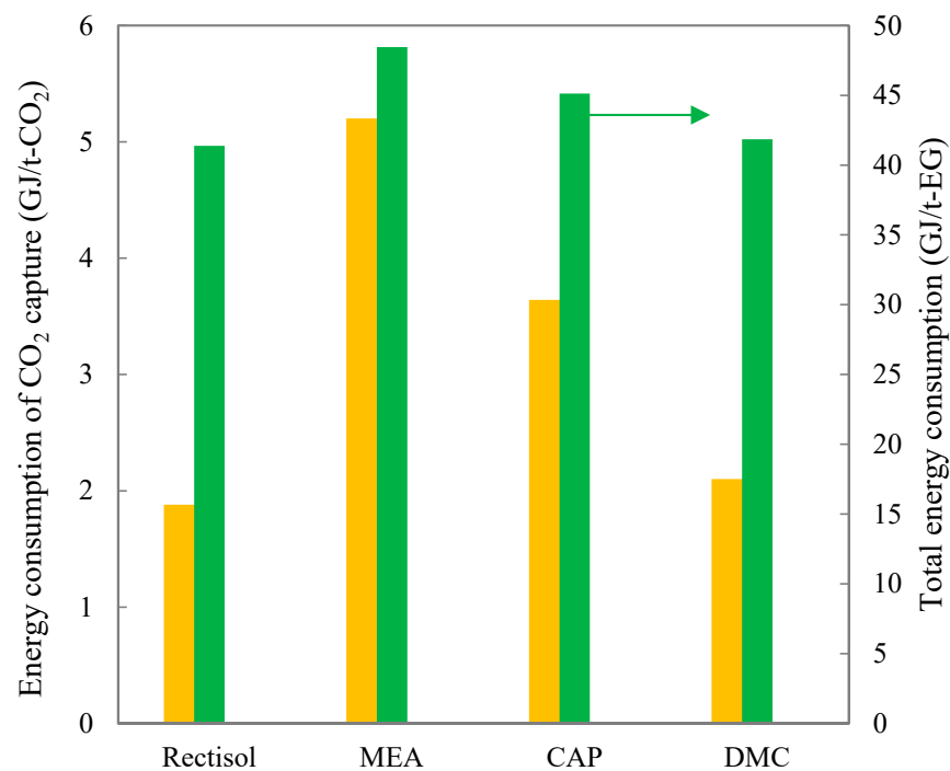
Figure 8. Energy consumption of CTEG process with different CO 2 capture technologies.
