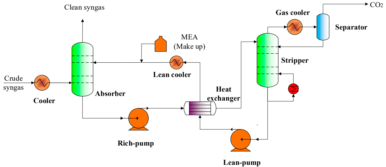
Figure 4. Simplified simulation flowsheet of the MEA technology.
