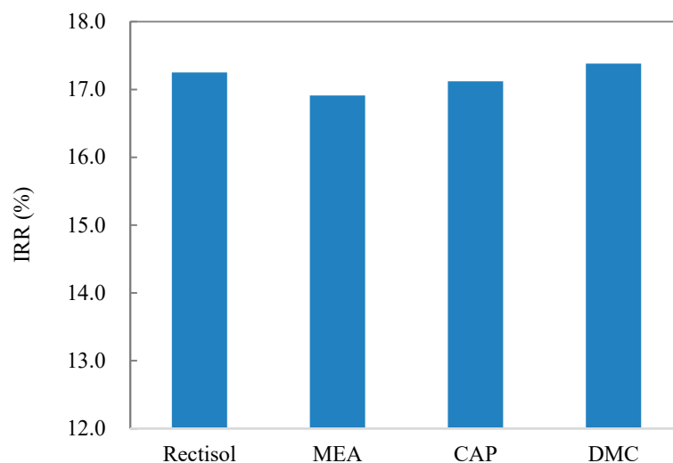
Figure 11. Internal rate of return of CTEG process with different CO 2 capture technologies.
