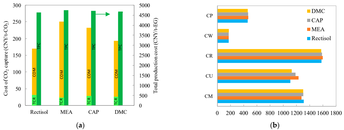
Figure 10. (a) Total production cost, (b) production cost compositions of the CTEG process with different CO 2 capture technologies.
