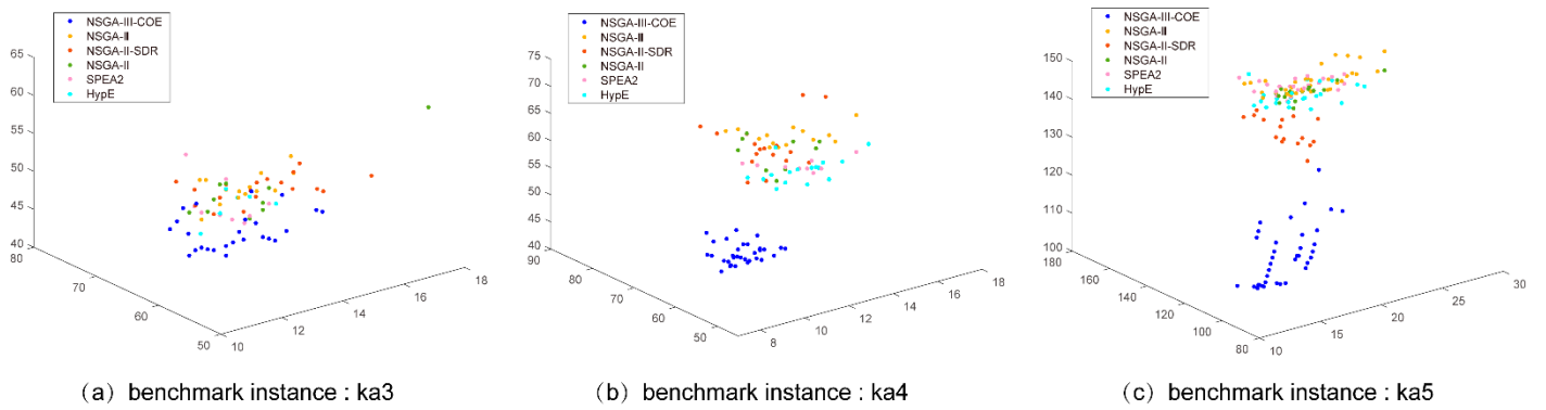
Figure 8. The non-dominated solutions of NSGA-III-COE, NSGA-III, NSGA-II, NSGA-II/SDR, SPEA2, and HypE on instances ka3, ka4, and ka5.
