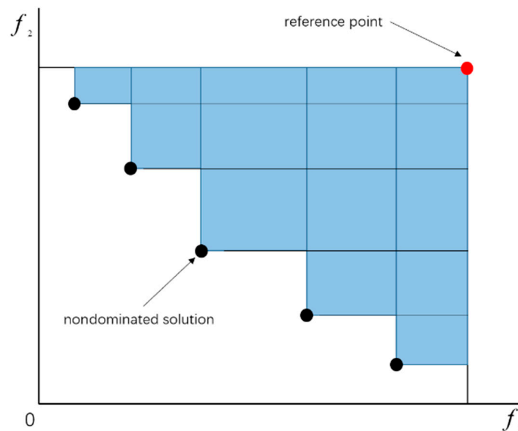
Figure 6. Diagram of the hypervolume ( HV ).
