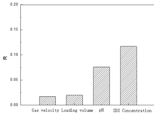
Figure 8. R value distribution of enrichment ratio E.
