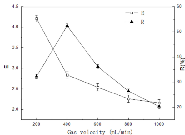
Figure 3. Effects of separated gas velocity on enrichment ratio and recovery.
