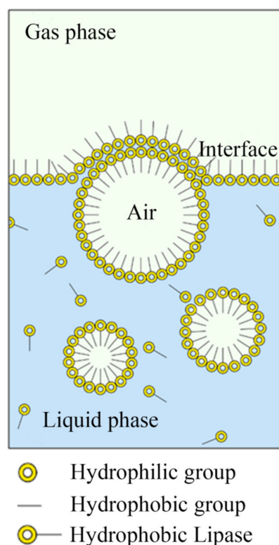
Figure 1. Adsorption of lipase B on the surface of bubbles.
