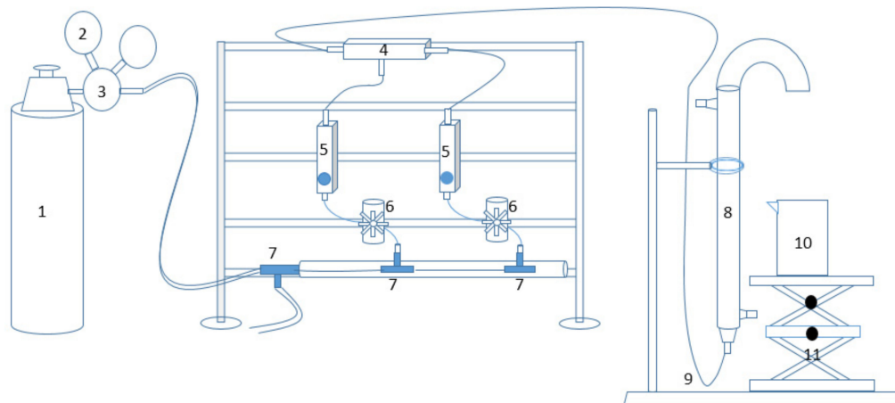
Figure 2. Schematic diagram of the foam separation device. 1, compressed air cylinder; 2, gas cylinder pressure gauge; 3, cylinder reduction valve; 4, gas mixer; 5, rotameter; 6, branch control valve; 7, main control valve; 8, foam separation column; 9, iron stand; 10, sample collection beaker; 11, lift.
