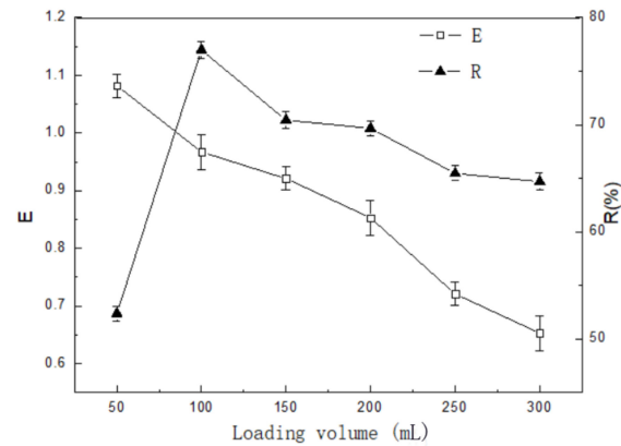
Figure 4. Effects of loading volume on enrichment ratio and recovery.
