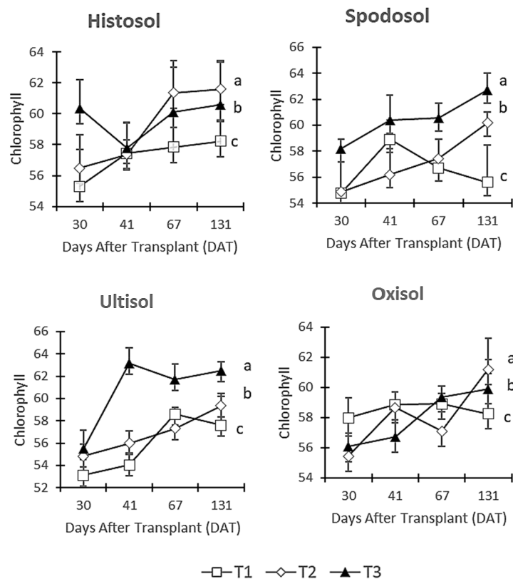
Figure 3. Chlorophyll index of the seedlings throughout the treatment period. Vertical bar represents the standard deviation. Different letters represent significant differences in Tukey's HSD comparison. Means sharing the same letter across treatments do not differ significantly at p -value ( p \leq 0.05 ).
