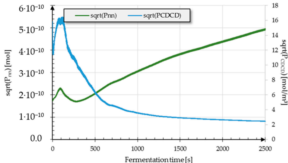
Figure 6. Estimation error of the CO 2 in non-gaseous dough and the amount of CO 2 in the bubble.
