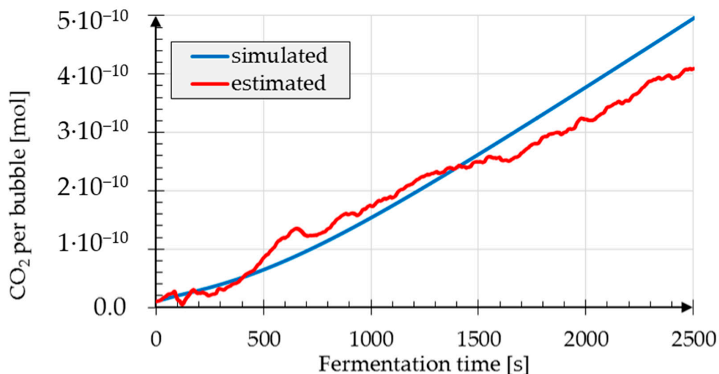
Figure 2. Simulated and Kalman estimation of the amount of \text{CO}_2 in a bubble.
