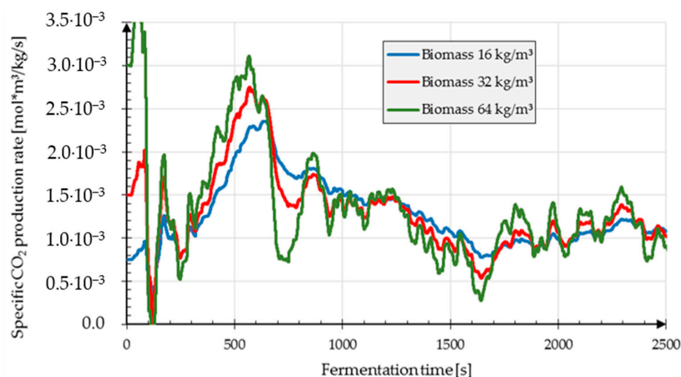
Figure 7. Estimated specific \text{CO}_2 production rate calculated during three runs of the extended Kalman filter with the same measurements but with different assumed yeast concentrations; the production rate was multiplied by 2 where the yeast concentration was considered to be 64 \text{ kg/m}^3 ; the production rate was divided by 2 where the yeast concentration was considered to be 16 \text{ kg/m}^3 ; the correct yeast concentration was 16 \text{ kg/m}^3 .
