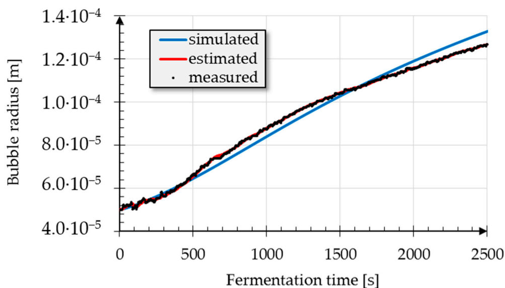
Figure 1. Bubble radii calculated by the imaging system compared to the values estimated by the extended Kalman filter as well as simulated values.
