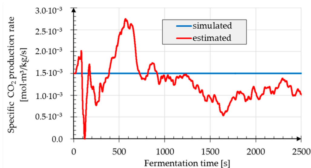
Figure 4. Simulated and Kalman estimation of the specific \text{CO}_2 production rate.
