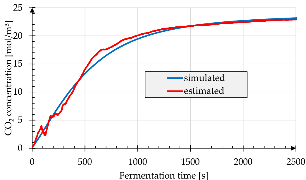
Figure 3. Simulated and Kalman estimation of the \text{CO}_2 concentration in non-gaseous dough.
