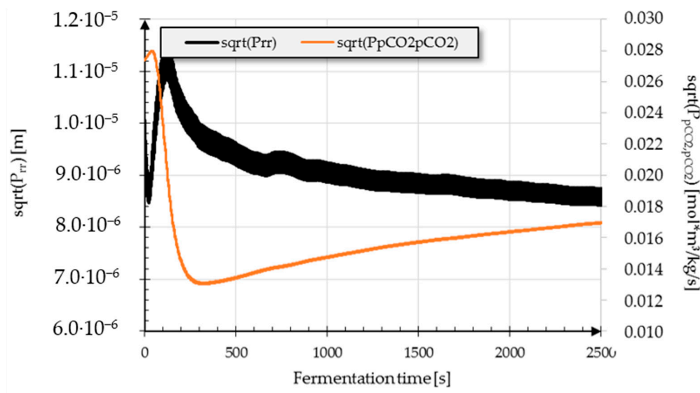
Figure 5. Estimation error variance of the radius and the specific CO 2 production rate.
