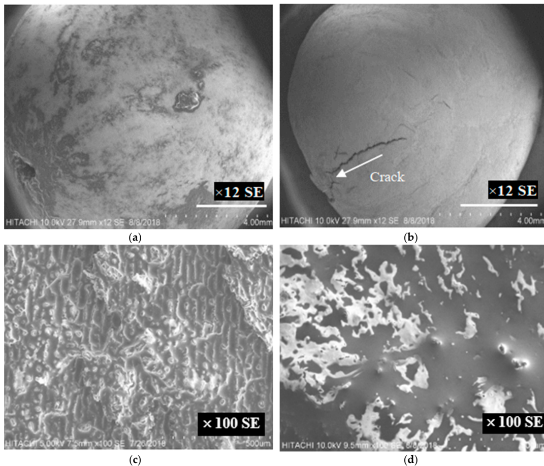
Figure 7. SEM of the surface of palm kernel before and after the drying process at 80 °C (a) 0.28 kg/kg, \times 12 SE, (b) 0.07 kg/kg, \times 12 SE, (c) 0.28 kg/kg, \times 100 SE, and (d) 0.07 kg/kg, \times 100 SE.
