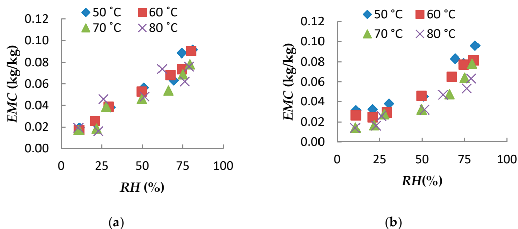
Figure 8. Desorption isotherm of whole palm kernel (a) and ground palm kernel (b).
