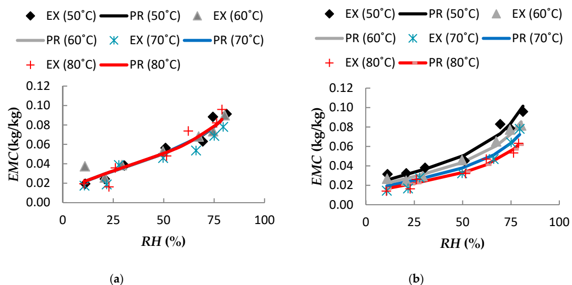
Figure 10. Experimental and predicted desorption isotherms for whole and ground palm kernel using modified Oswin model (a) and modified Halsey (b), respectively.
