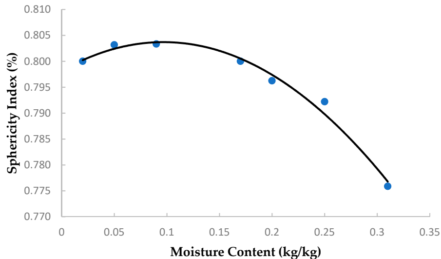
Figure 2. Sphericity index ( \gamma ) of palm kernel at different moisture contents.
