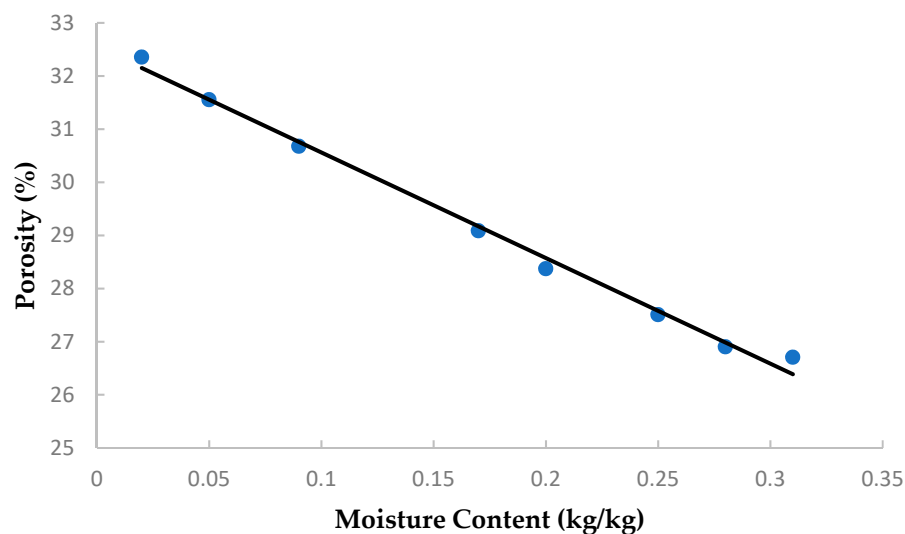
Figure 5. Total porosity of palm kernel at different moisture contents.
