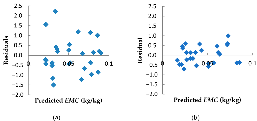
Figure 9. Residuals of predicated EMC for (a) whole kernel (modified Oswin model) and (b) ground kernel (modified Halsey model).
