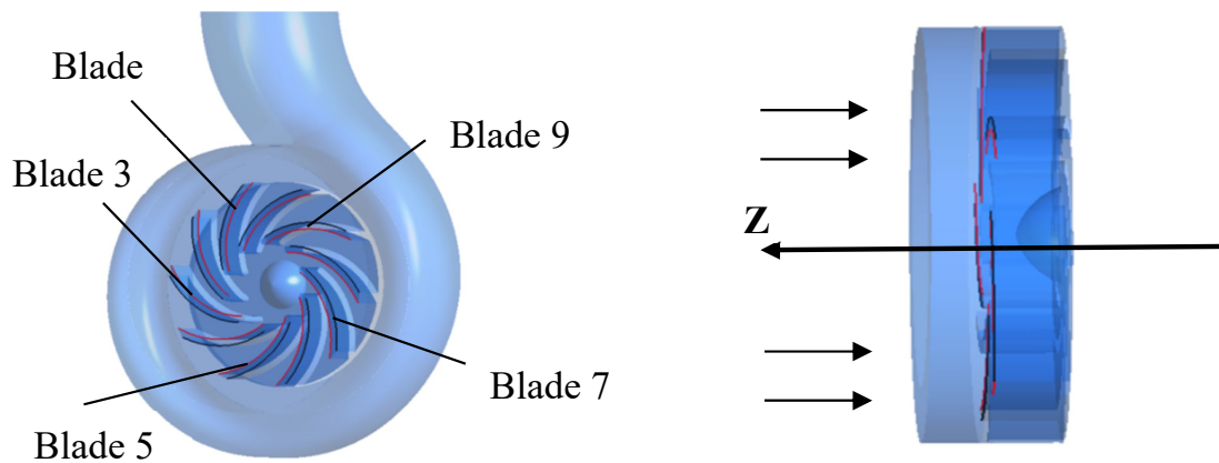
Figure 13. Schematic of blade number.
